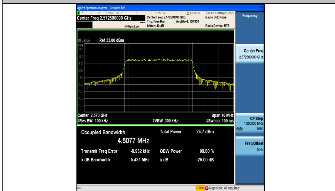
Band38-5MHz-16QAM-37775-25RB#0-PASS
