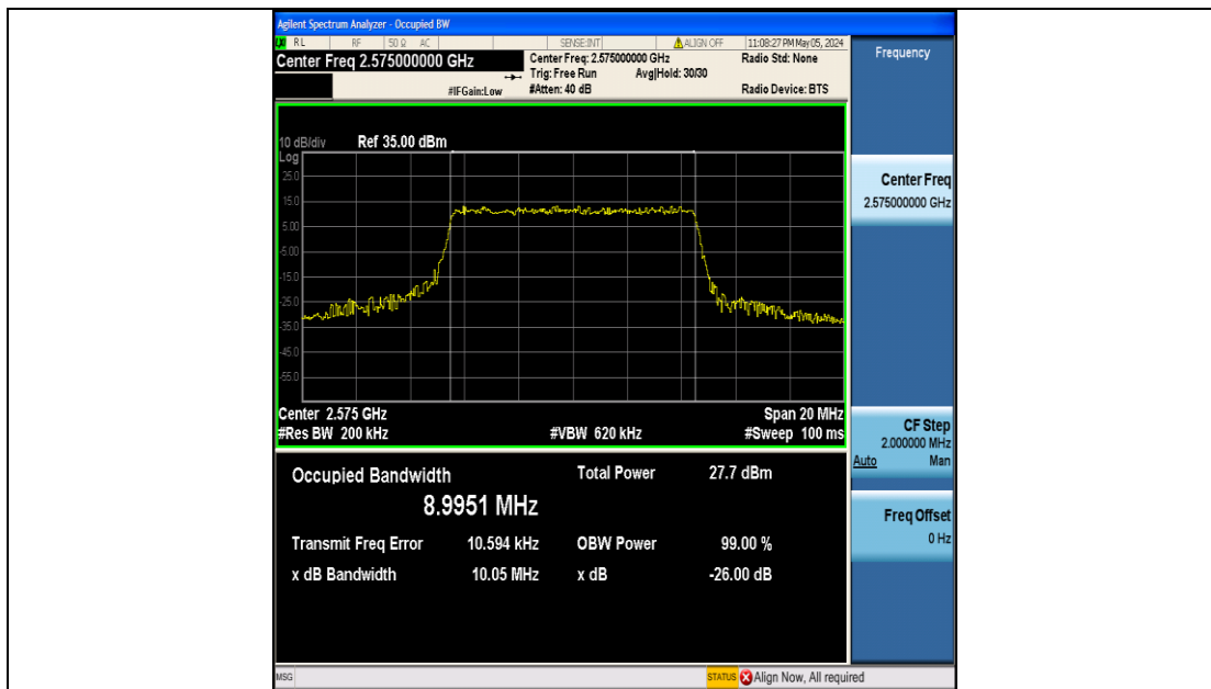
Band38-10MHz-QPSK-37800-50RB#0-PASS
