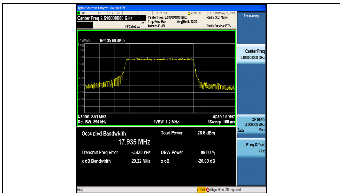
Band38-20MHz-QPSK-38150-100RB#0-PASS
