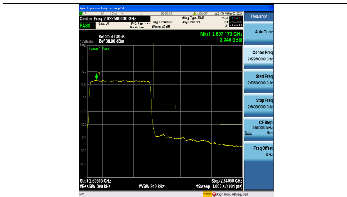
Band38_15MHz_16QAM_38175_75RB#0
