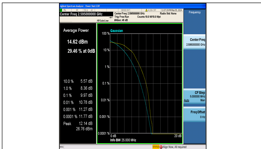
Band38-5MHz-16QAM-38000-25RB#0-PASS
