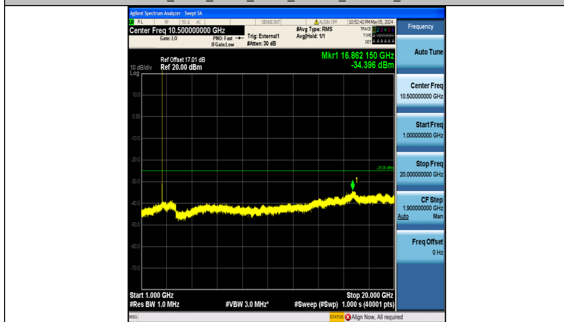
Band38_5MHz_QPSK_37775_25RB#0_1000~20000_1000~20000
