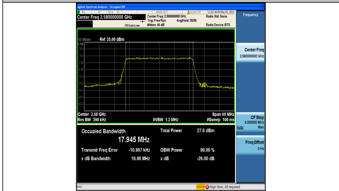
Band38-20MHz-16QAM-37850-100RB#0-PASS
