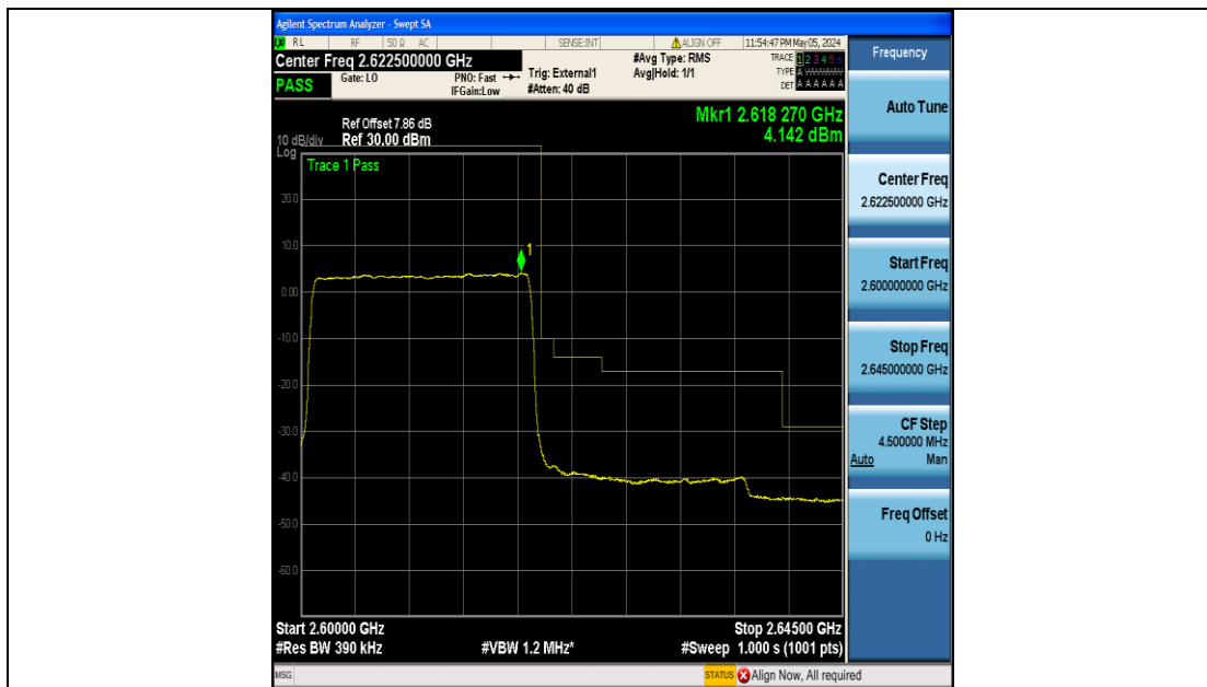
Band38_20MHz_QPSK_38150_100RB#0
