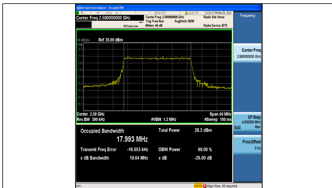
Band38-20MHz-QPSK-37850-100RB#0-PASS
