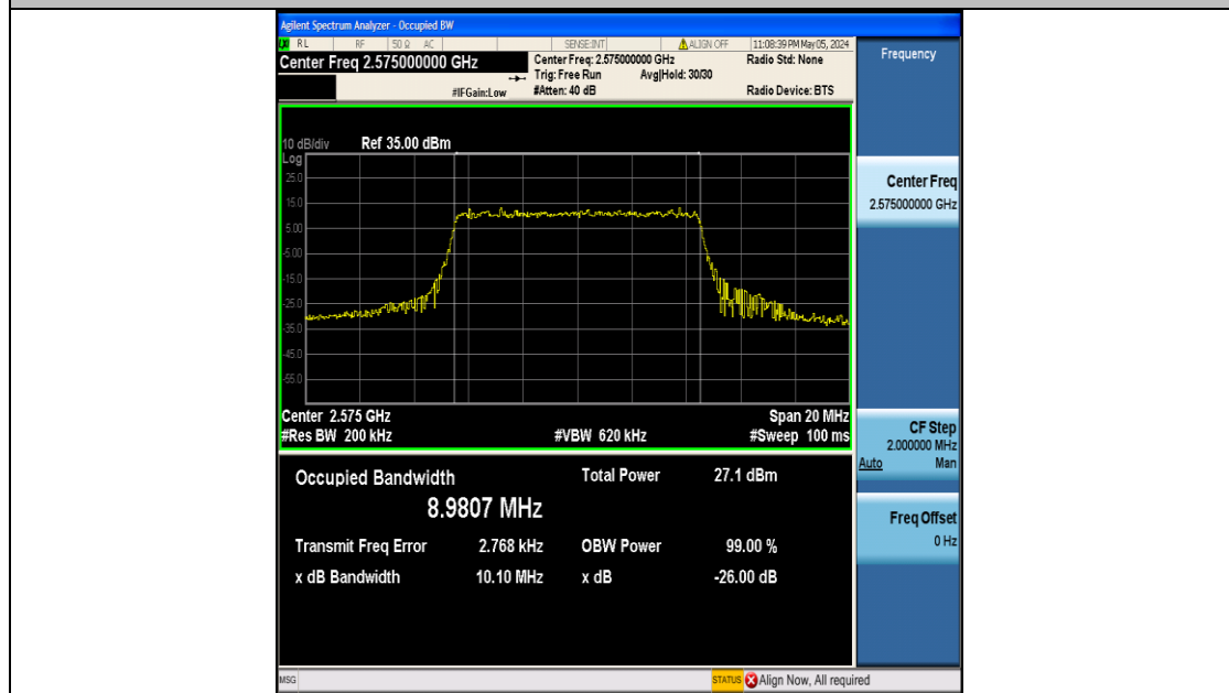
Band38-10MHz-16QAM-37800-50RB#0-PASS
