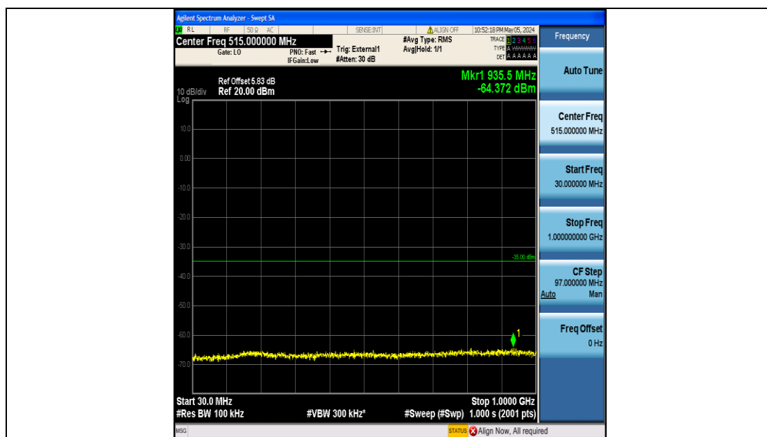
Band38_5MHz_QPSK_37775_25RB#0_30~1000_30~1000
