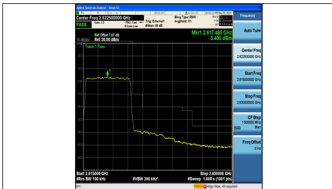
Band38_5MHz_16QAM_38225_25RB#0
