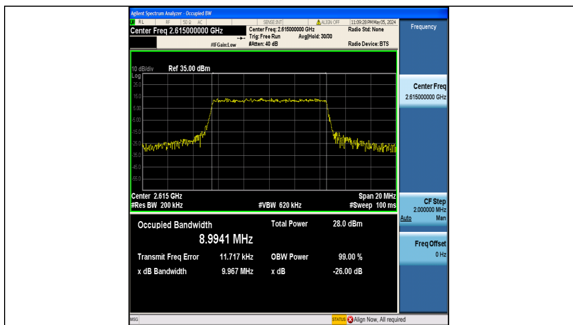
Band38-10MHz-QPSK-38200-50RB#0-PASS
