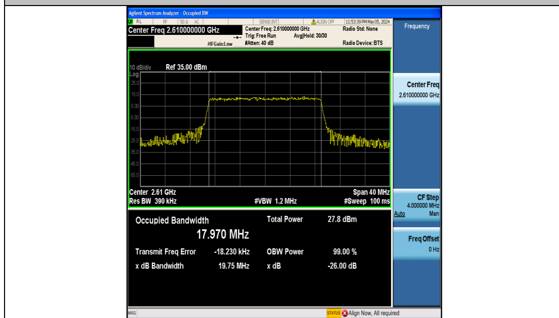
Band38-20MHz-16QAM-38150-100RB#0-PASS
