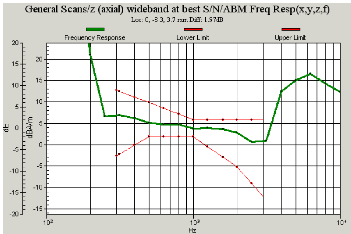
Figure 18 T-Coil GSM 1900 Z Axial
