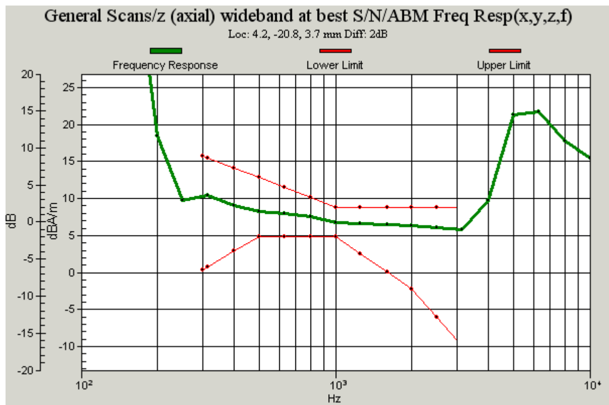
Figure 26 T-Coil WCDMA Band V Z Axial
