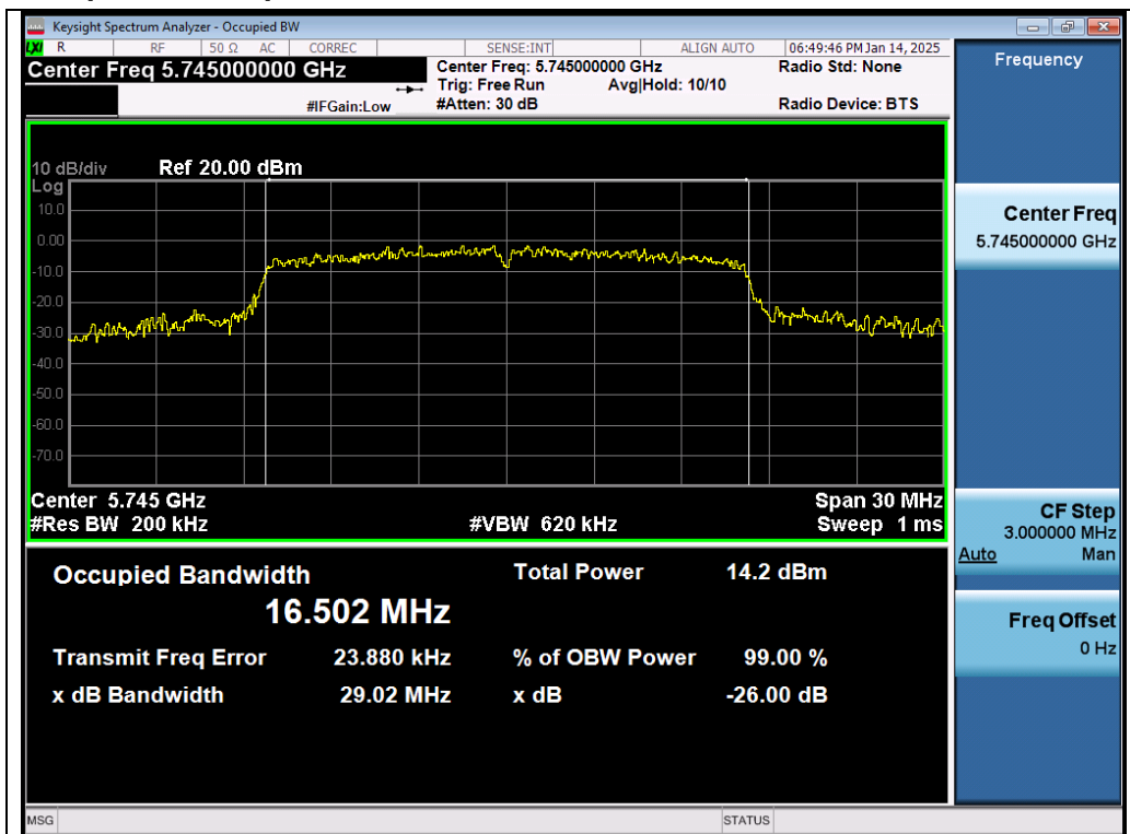
Test_Graph_802.11a_Chain A_5745_6Mbps_OBW
