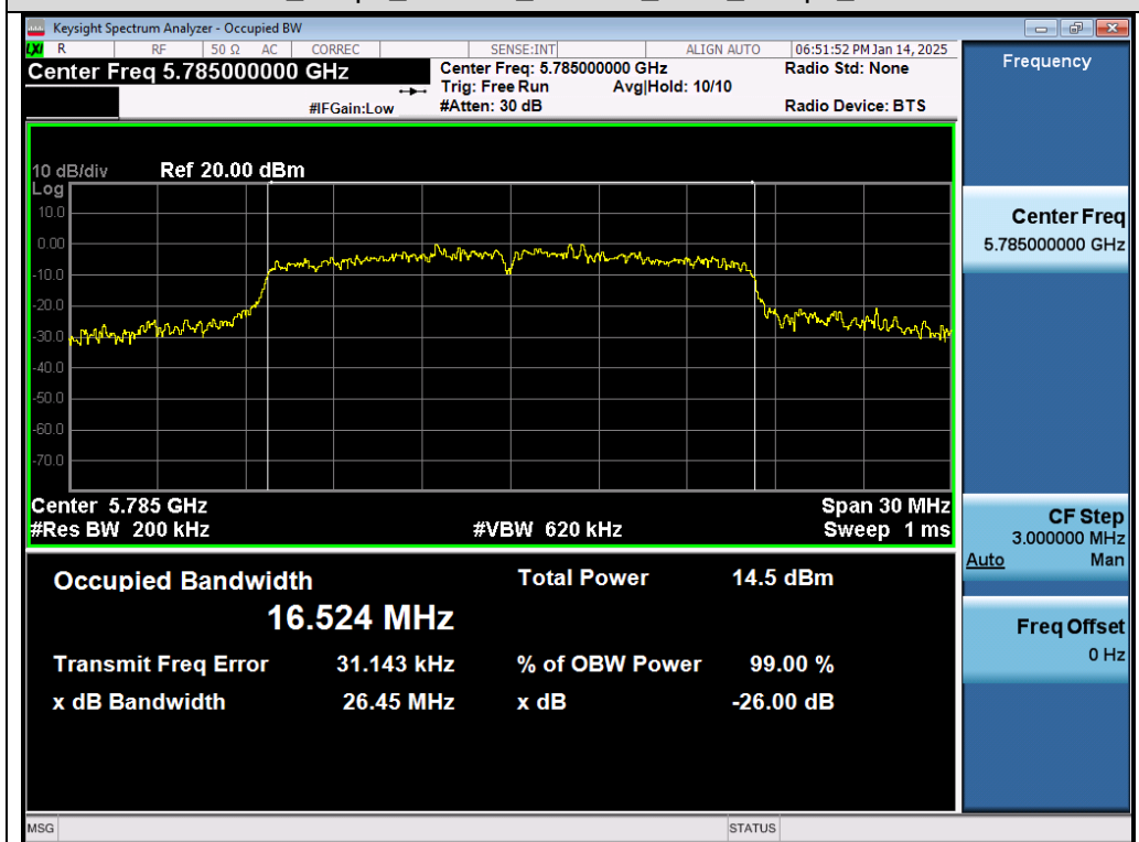
Test_Graph_802.11a_Chain A_5785_6Mbps_OBW
