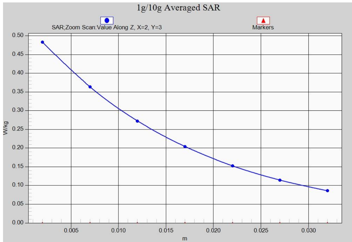
Fig. 25-1 Z-Scan at power reference point (LTE Band14)
