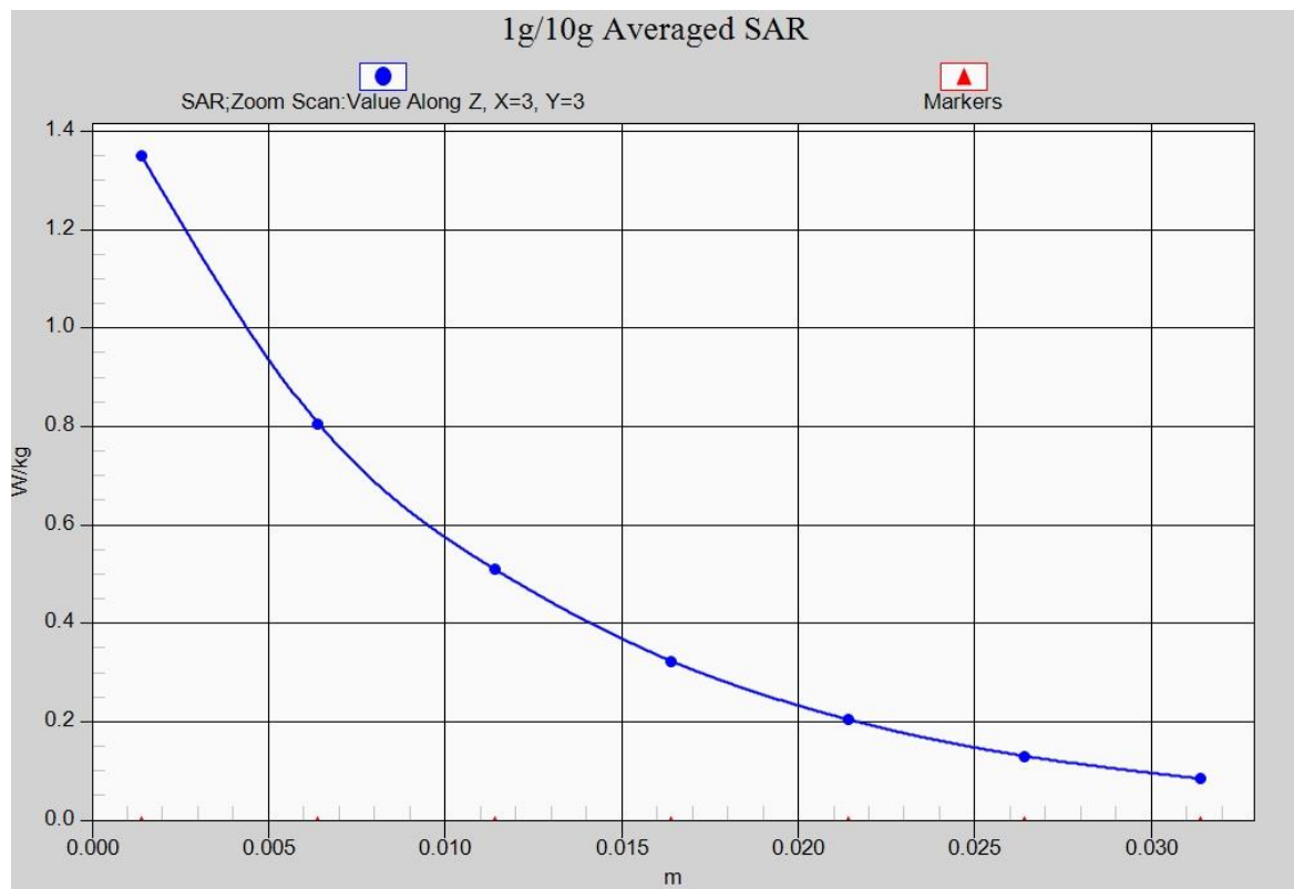
Fig. 18-1 Z-Scan at power reference point (LTE Band4)
