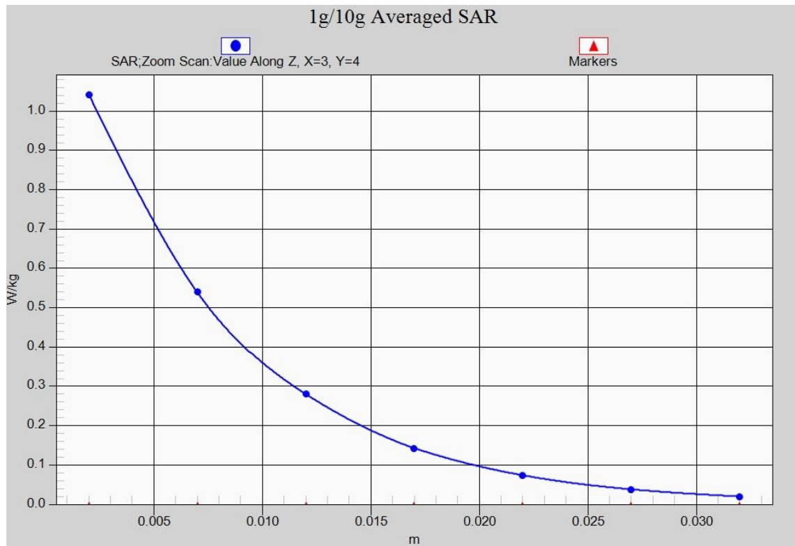
Fig. 29-1 Z-Scan at power reference point (2450 MHz)
