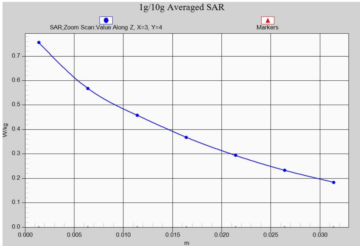
Fig. 7-1 Z-Scan at power reference point (WCDMA850)
