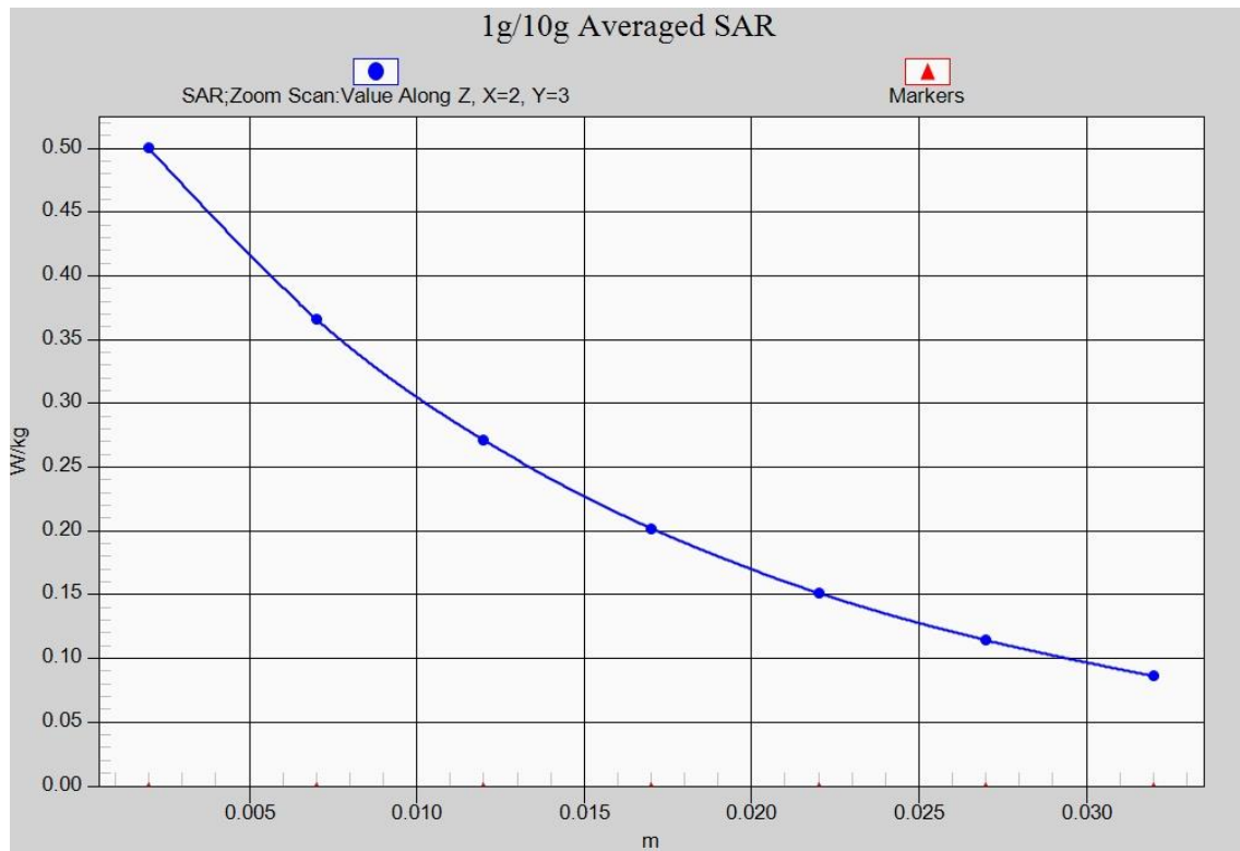
Fig. 23-1 Z-Scan at power reference point (LTE Band12)
