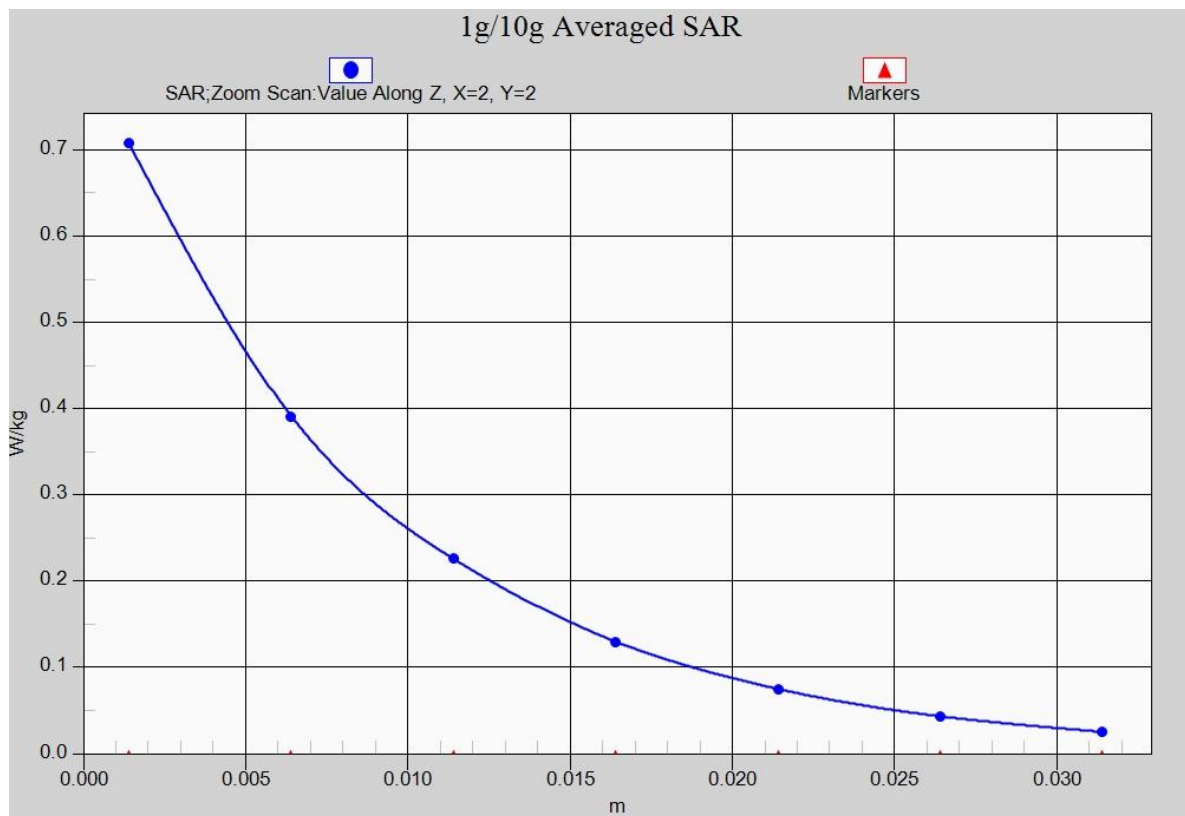
Fig. 28-1 Z-Scan at power reference point (LTE Band30)
