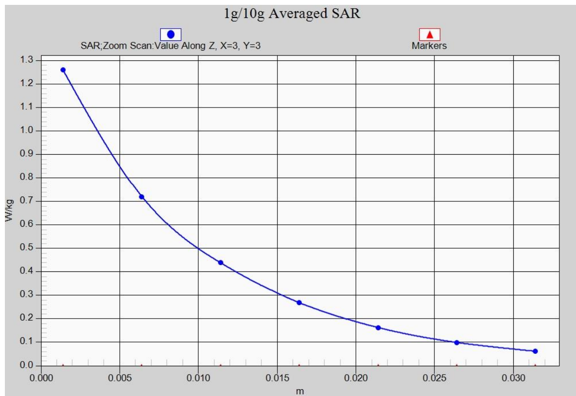
Fig. 12-1 Z-Scan at power reference point (WCDMA1900)
