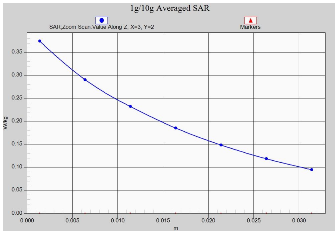
Fig. 24-1 Z-Scan at power reference point (LTE Band14)
