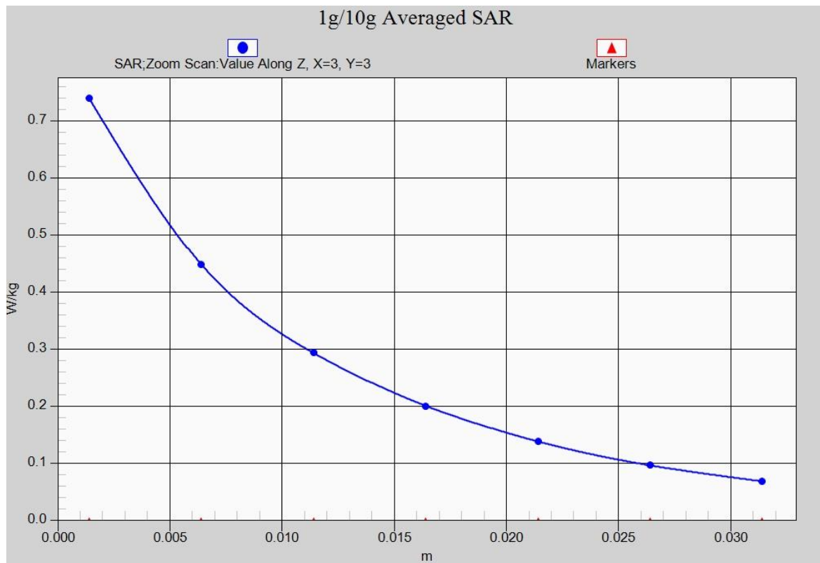
Fig. 11-1 Z-Scan at power reference point (WCDMA1900)
