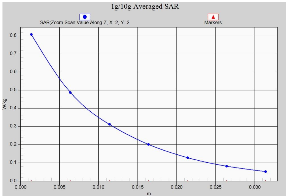
Fig. 16-1 Z-Scan at power reference point (LTE Band2)
