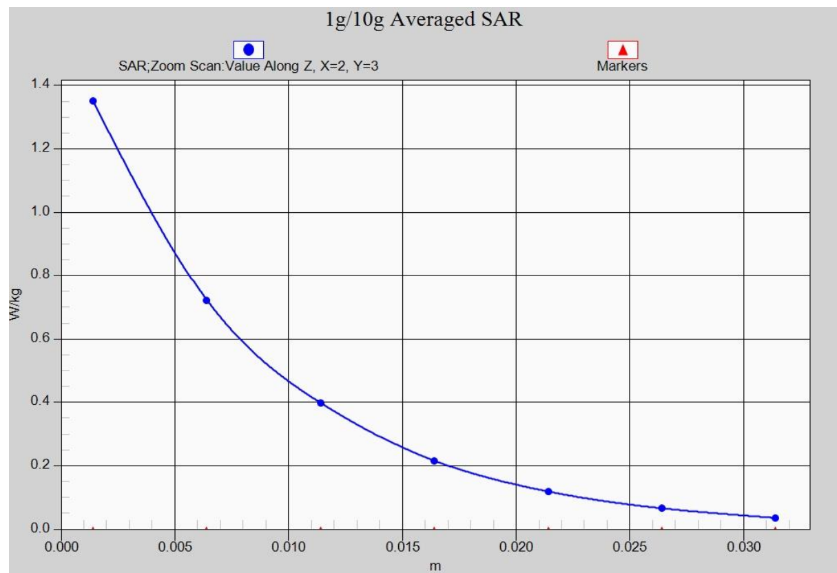
Fig. 27-1 Z-Scan at power reference point (LTE Band30)
