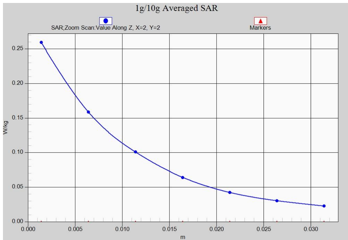
Fig. 26-1 Z-Scan at power reference point (LTE Band30)
