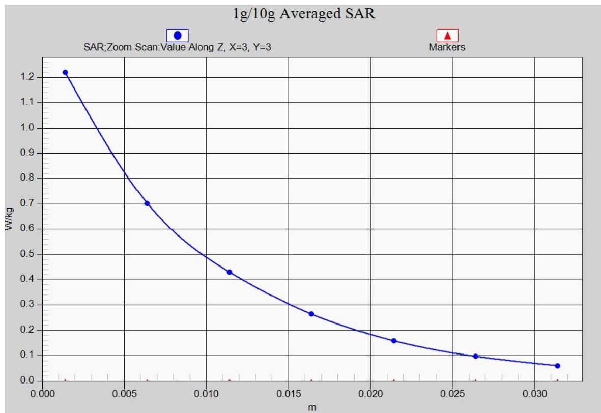
Fig. 15-1 Z-Scan at power reference point (LTE Band2)
