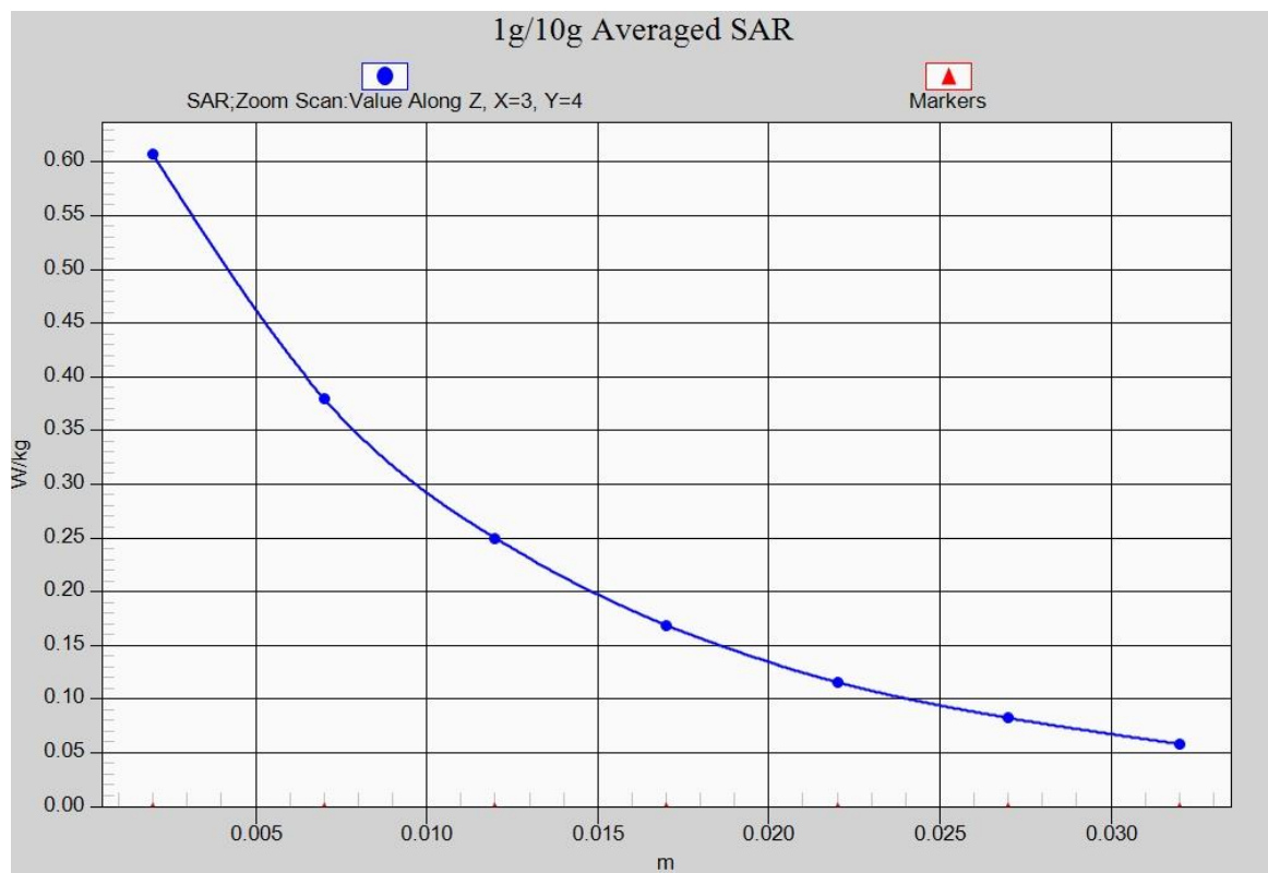
Fig. 14-1 Z-Scan at power reference point (LTE Band2)
