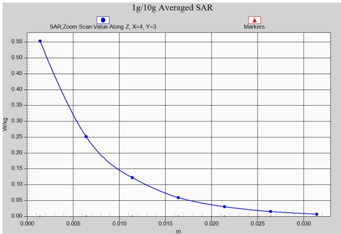
Fig. 30-1 Z-Scan at power reference point (2450 MHz)
