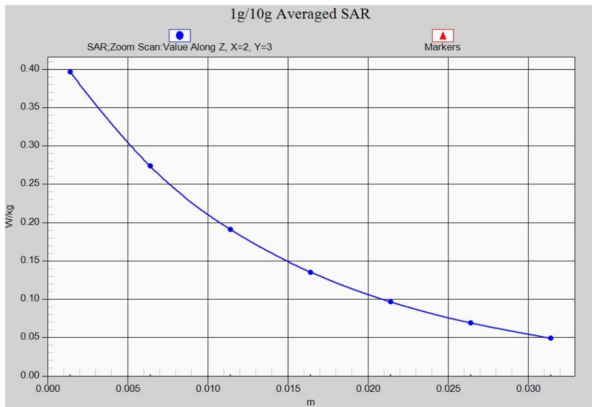
Fig. 17-1 Z-Scan at power reference point (LTE Band4)
