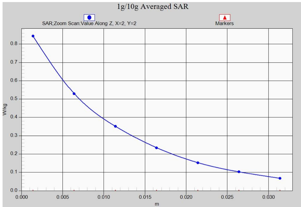
Fig. 19-1 Z-Scan at power reference point (LTE Band4)
