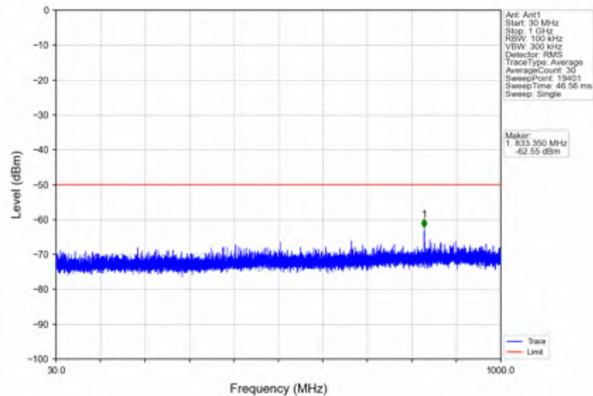
n78d_30kHz_SISO_NTNV_90MHz_DFT-s-OFDM QPSK_3654.99MHz_Inner_1RB_Right
