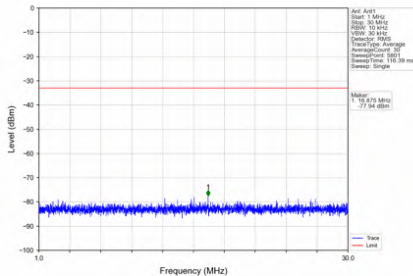
n78e_15kHz_SISO_NTNV_15MHz_DFT-s-OFDM_QPSK_3457.5MHz_Outer_Full
