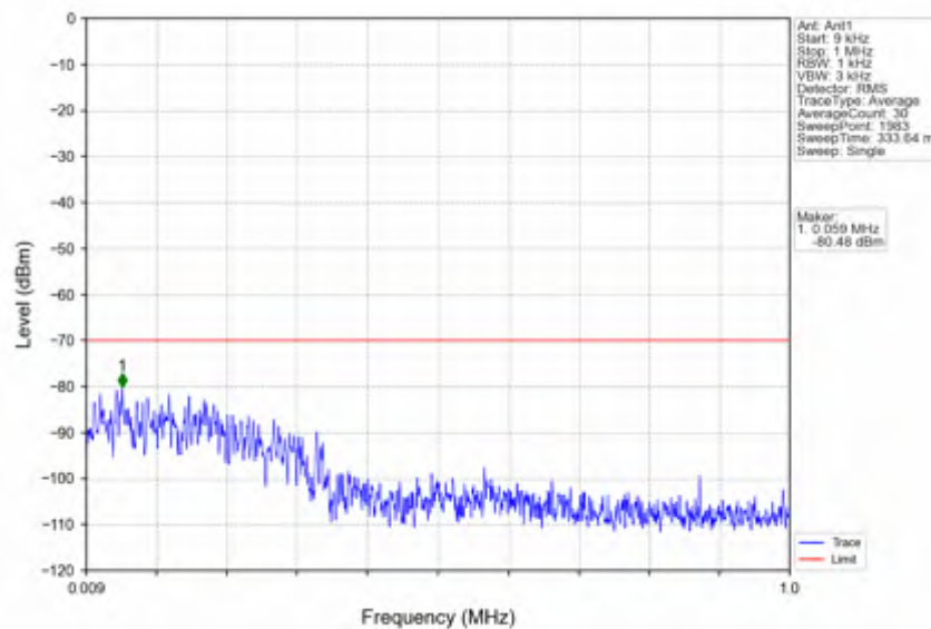
n78d_30kHz_SISO_NTNV_100MHz_CP-OFDM QPSK_3600MHz_Edge_1RB_Left
