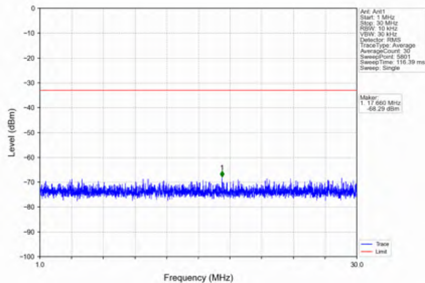
n78e_15kHz_SISO_NTNV_15MHz_DFT-s-OFDM QPSK_3499.995MHz_Edge_1RB_Left
