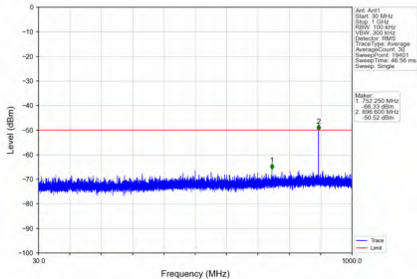
n78d_30kHz_SISO_NTNV_90MHz_CP-OFDM QPSK_3654.99MHz_Edge_1RB_Right
