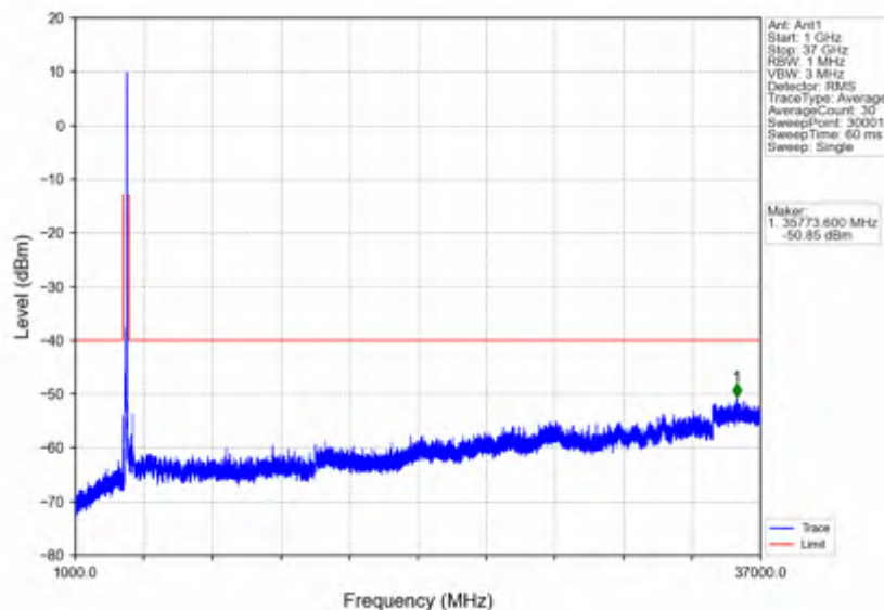
n78d_30kHz_SISO_NTNV_100MHz_DFT-s-OFDM QPSK_3600MHz_Edge_1RB_Left
