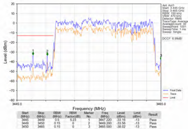
n78e_15kHz_SISO_NTNV_15MHz_DFT-s-OFDM_QPSK_3457.5MHz_Outer_Full
