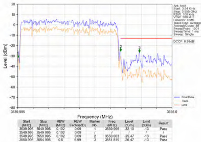
n78e_15kHz_SISO_NTNV_10MHz_CP-OFDM QPSK_3544.995MHz_Outer_Full
