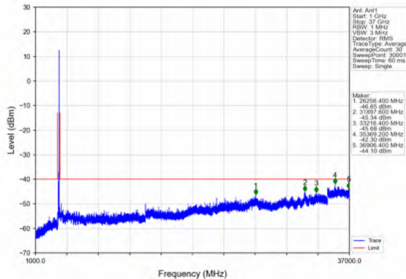
n78d_30kHz_SISO_NTNV_90MHz_DFT-s-OFDM QPSK_3654.99MHz_Inner_1RB_Right
