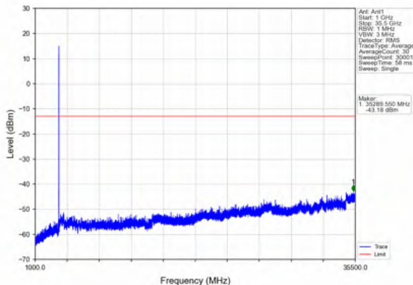
n78e_15kHz_SISO_NTNV_15MHz_CP-OFDM QPSK_3542.49MHz_Outer_Full
