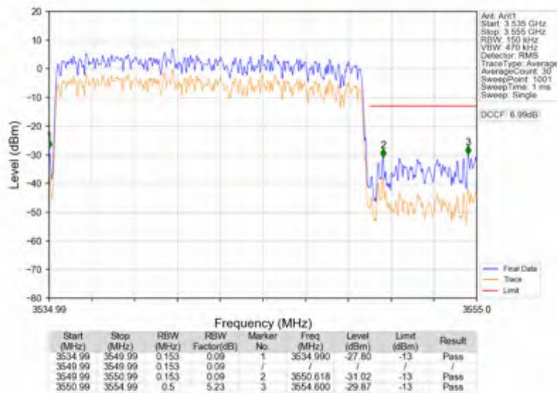
n78e_15kHz_SISO_NTNV_15MHz_CP-OFDM QPSK_3542.49MHz_Outer_Full
