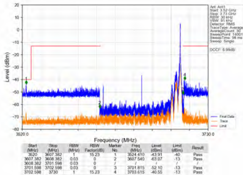
n78d_30kHz_SISO_NTNV_90MHz_CP-OFDM_QPSK_3654.99MHz_Inner_1RB_Right
