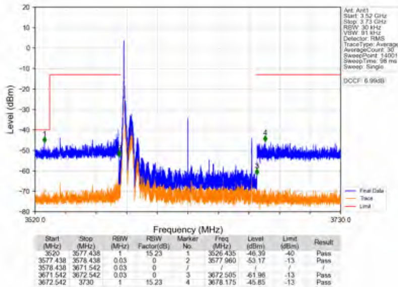
n78d_30kHz_SISO_NTV_90MHz_CP-OFDM QPSK_3624.99MHz_Edge_1RB_Left
