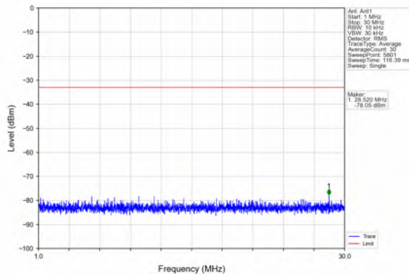
n78e_15kHz_SISO_NTNV_15MHz_DFT-s-OFDM QPSK_3542.49MHz_Inner_1RB_Right
