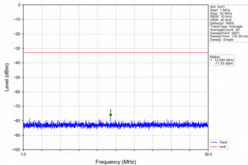
n78e_15kHz_SISO_NTNV_15MHz_CP-OFDM QPSK_3542.49MHz_Inner_1RB_Right
