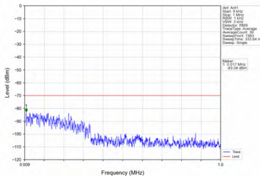
n78d_30kHz_SISO_NTNV_90MHz_CP-OFDM_QPSK_3654.99MHz_Inner_1RB_Right
