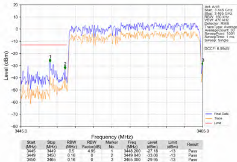
n78e_15kHz_SISO_NTNV_15MHz_CP-OFDM QPSK_3457.5MHz_Outer_Full
