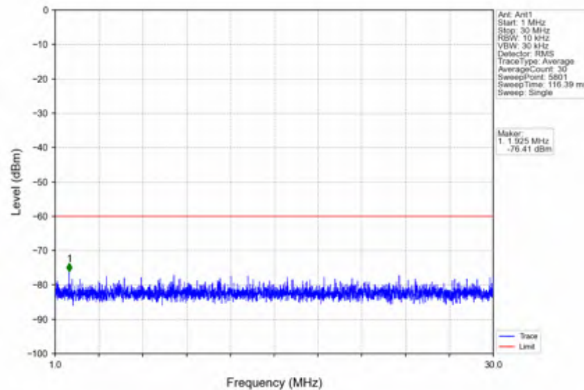
n78d_30kHz_SISO_NTNV_100MHz_DFT-s-OFDM QPSK_3600MHz_Edge_1RB_Left
