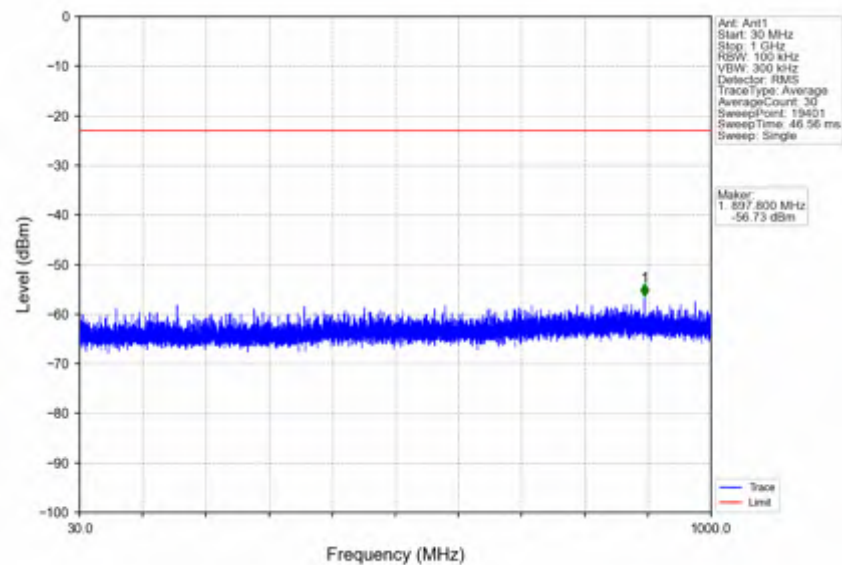
n78e_15kHz_SISO_NTNV_15MHz_CP-OFDM_QPSK_3499.995MHz_Edge_1RB_Left
