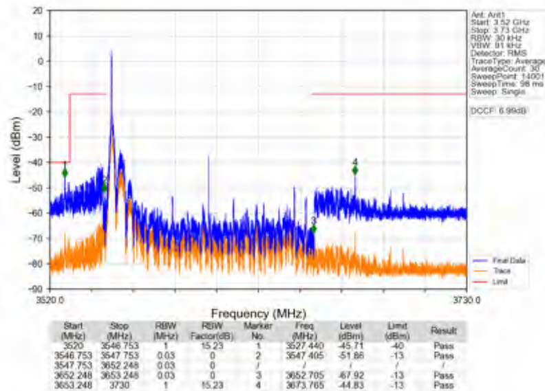
n78d_30kHz_SISO_NTNV_100MHz_DFT-s-OFDM_PI/2_BPSK_3600MHz_Edge_1RB_Left
