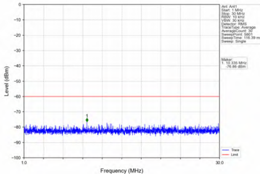
n78d_30kHz_SISO_NTNV_100MHz_CP-OFDM QPSK_3600MHz_Edge_1RB_Left
