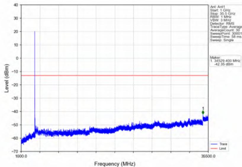
n78e_15kHz_SISO_NTNV_15MHz_CP-OFDM_QPSK_3499.995MHz_Edge_1RB_Left
