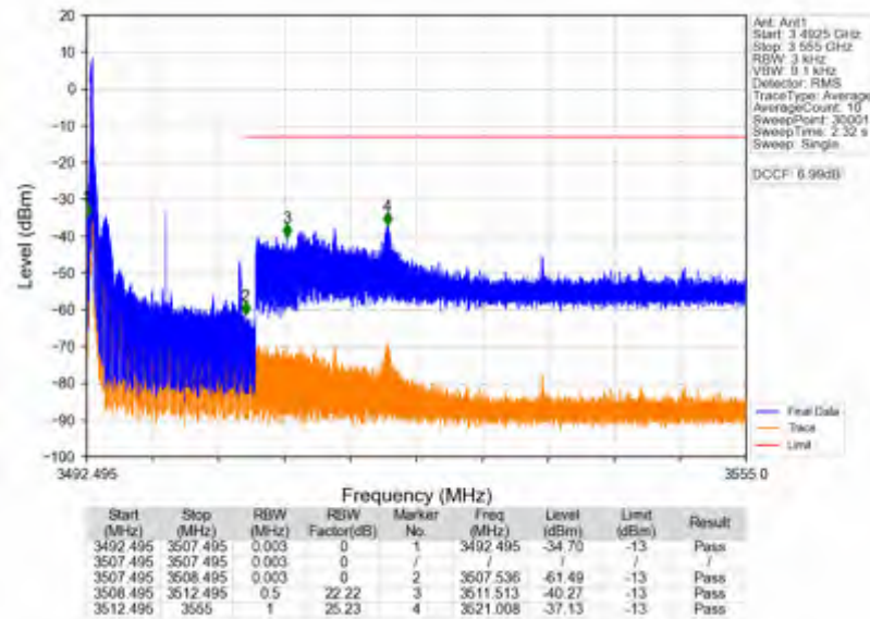
n78e_15kHz_SISO_NTNV_15MHz_DFT-s-OFDM_QPSK_3499.995MHz_Edge_1RB_Left
