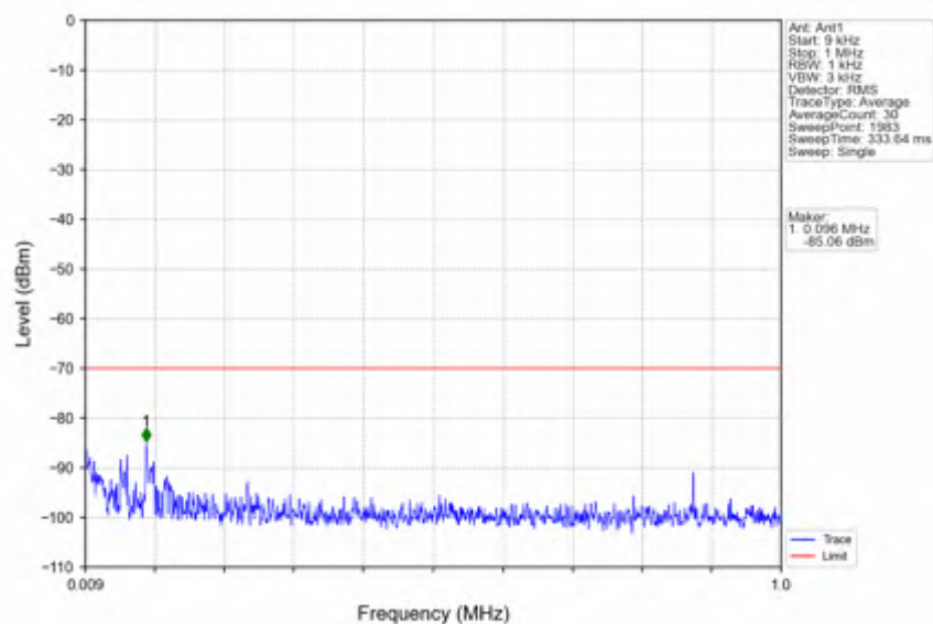
n78d_30kHz_SISO_NTNV_100MHz_DFT-s-OFDM_PI/2_BPSK_3600MHz_Edge_1RB_Left
