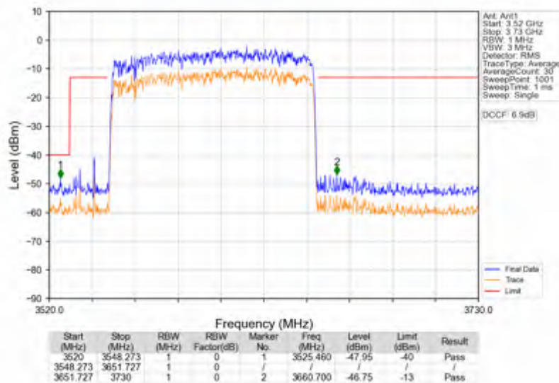
n78d_30kHz_SISO_NTNV_100MHz_CP-OFDM QPSK_3600MHz_Outer_Full
