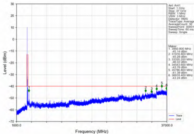
n78d_30kHz_SISO_NTNV_100MHz_CP-OFDM QPSK_3600MHz_Outer_Full
