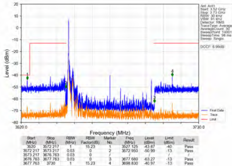
n78d_30kHz_SISO_NTNV_100MHz_DFT-s-OFDM QPSK_3624.99MHz_Edge_1RB_Left
