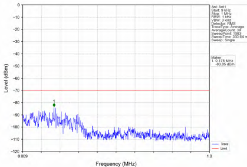
n78d_30kHz_SISO_NTNV_100MHz_DFT-s-OFDM QPSK_3624.99MHz_Edge_1RB_Left
