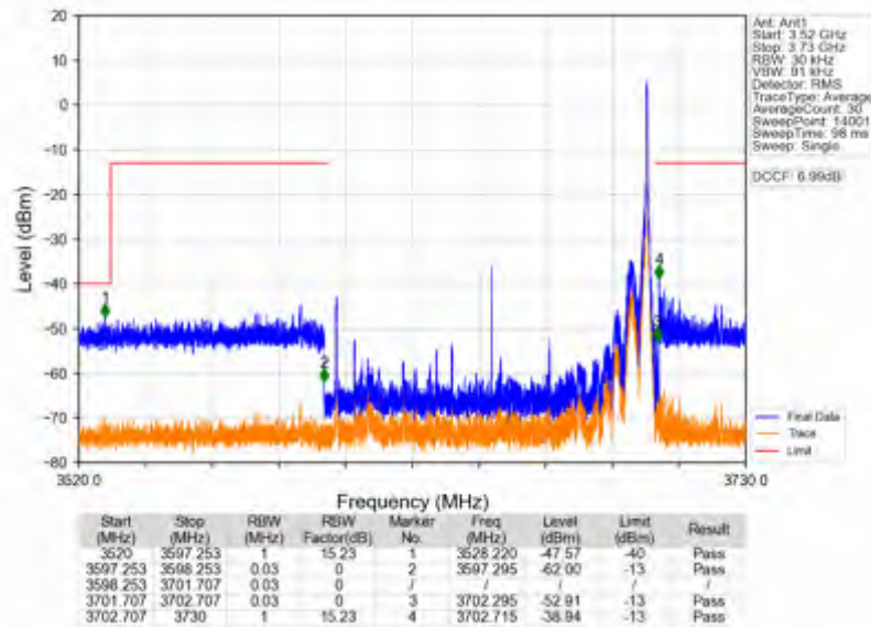
n78d_30kHz_SISO_NTNV_100MHz_DFT-s-OFDM QPSK_3649.98MHz_Edge_1RB_Right
