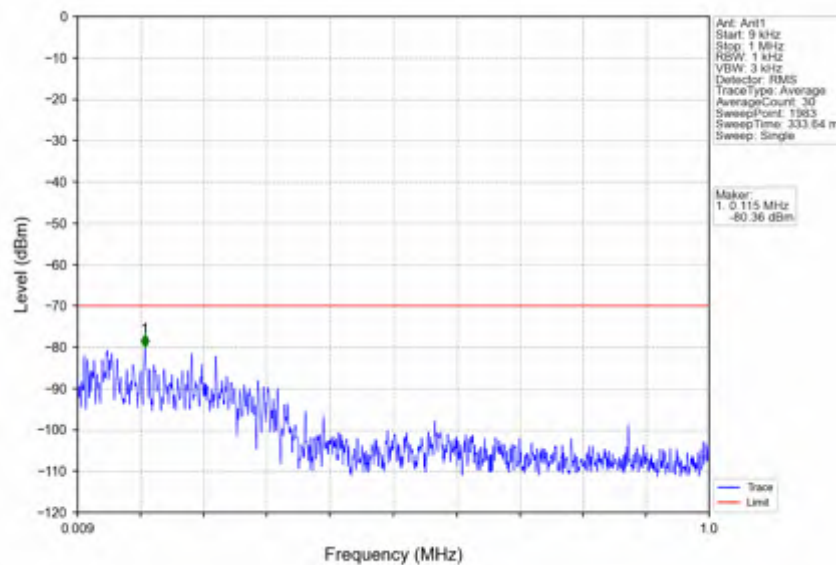
n78d_30kHz_SISO_NTNV_100MHz_CP-OFDM QPSK_3600MHz_Inner_1RB_Left
