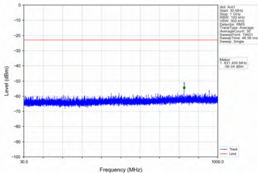
n78e_15kHz_SISO_NTNV_15MHz_CP-OFDM QPSK_3542.49MHz_Edge_1RB_Right
