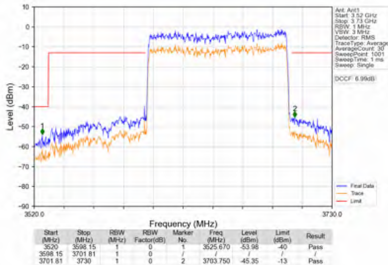
n78d_30kHz_SISO_NTNV_100MHz_DFT-s-OFDM PI/2 BPSK_3649.98MHz_Outer_Full
