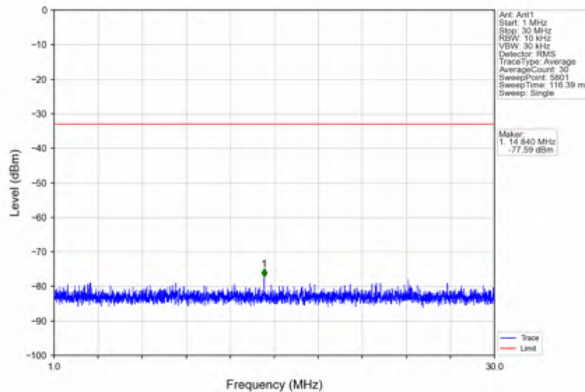
n78e_15kHz_SISO_NTNV_15MHz_DFT-s-OFDM_QPSK_3542.49MHz_Outer_Full
