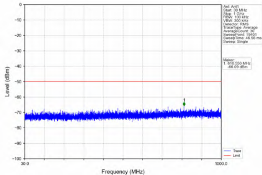
n78d_30kHz_SISO_NTNV_100MHz_DFT-s-OFDM_QPSK_3600MHz_Inner_1RB_Left
