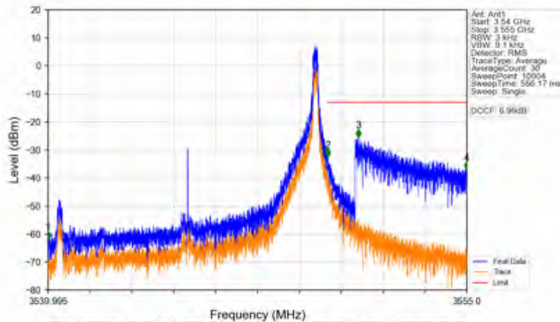
n78e_15kHz_SISO_NTNV_10MHz_DFT-s-OFDM_QPSK_3544.995MHz_Edge_1RB_Right
