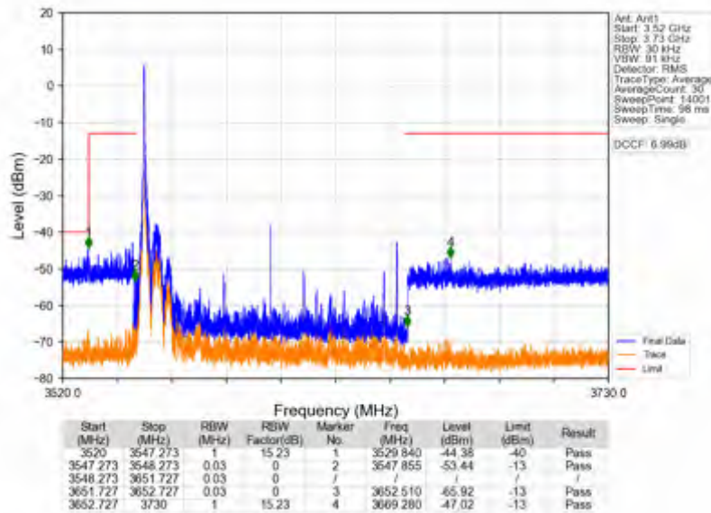
n78d_30kHz_SISO_NTNV_100MHz_DFT-s-OFDM QPSK_3600MHz_Inner_1RB_Left
