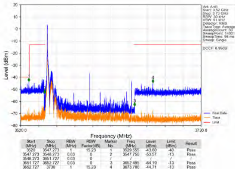
n78d_30kHz_SISO_NTNV_100MHz_DFT-s-OFDM QPSK_3600MHz_Edge_1RB_Left
