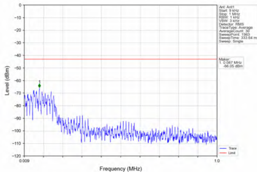
n78e_15kHz_SISO_NTNV_15MHz_DFT-s-OFDM QPSK_3542.49MHz_Edge_1RB_Right
