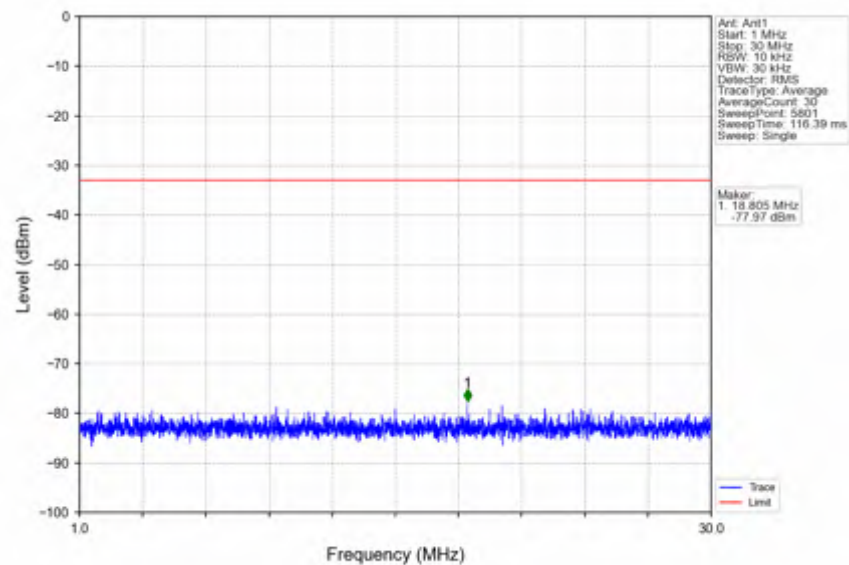
n78e_15kHz_SISO_NTNV_10MHz_CP-OFDM_QPSK_3544.995MHz_Outer_Full
