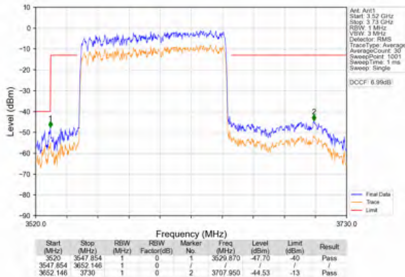
n78d_30kHz_SISO_NTNV_100MHz_DFT-s-OFDM PI/2 BPSK_3600MHz_Outer_Full
