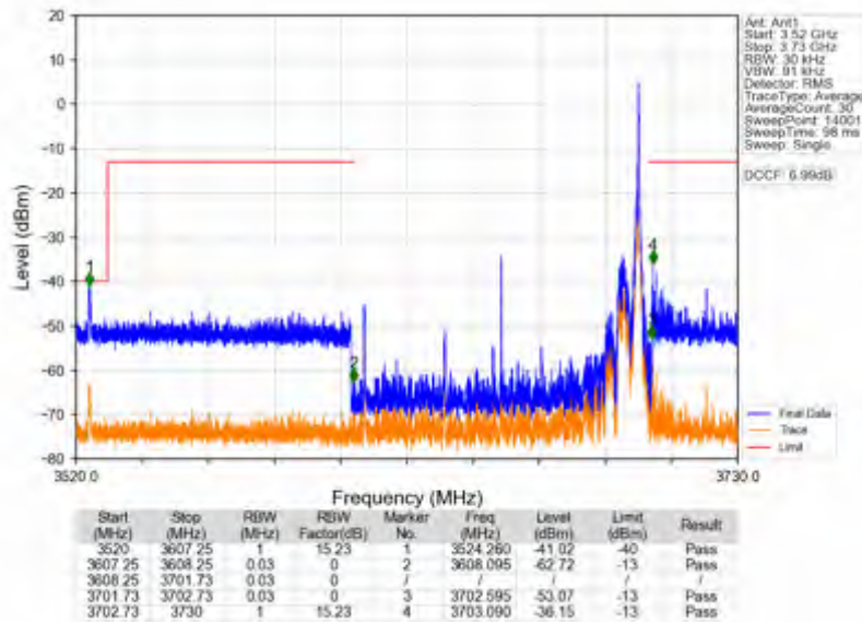
n78d_30kHz_SISO_NTNV_90MHz_DFT-s-OFDM QPSK_3654.99MHz_Inner_1RB_Right
