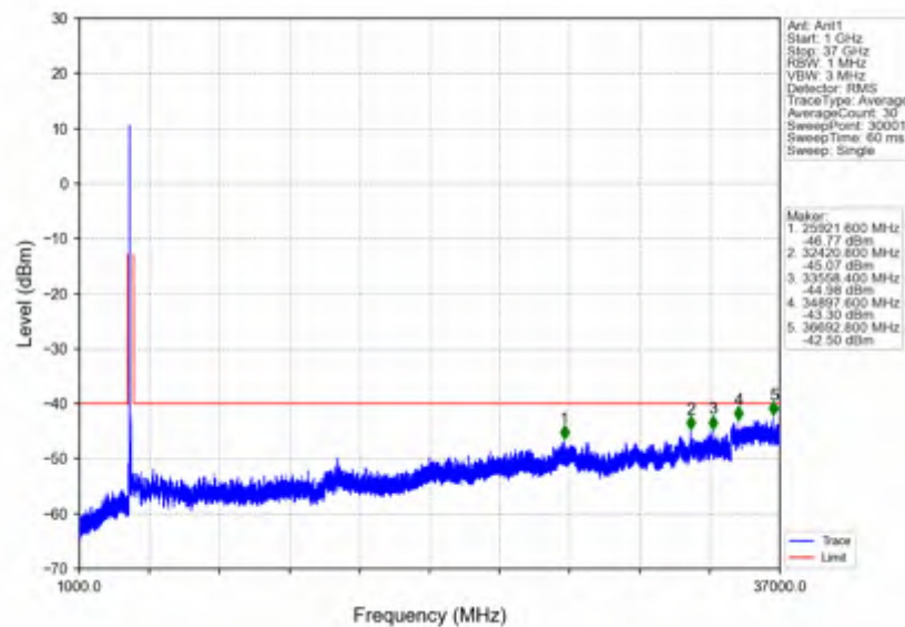
n78d_30kHz_SISO_NTNV_100MHz_DFT-s-OFDM QPSK_3649.98MHz_Edge_1RB_Right
