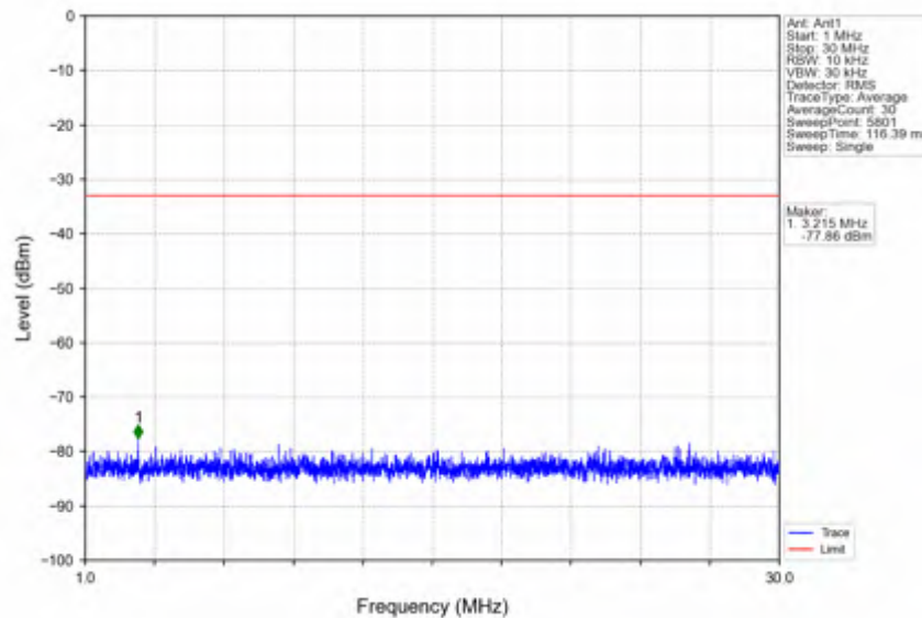
n78e_15kHz_SISO_NTNV_10MHz_DFT-s-OFDM_QPSK_3455.01MHz_Outer_Full
