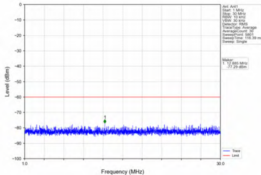
n78d_30kHz_SISO_NTNV_100MHz_CP-OFDM QPSK_3600MHz_Inner_1RB_Left
