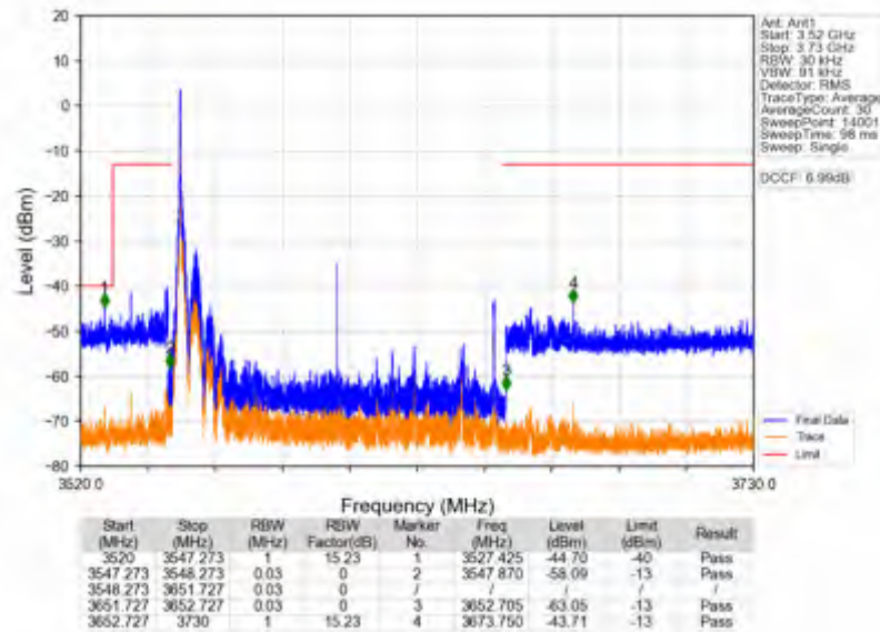
n78d_30kHz_SISO_NTNV_100MHz_CP-OFDM QPSK_3600MHz_Edge_1RB_Left
