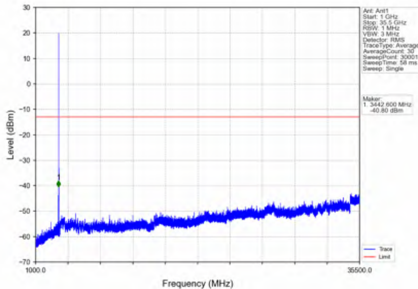
n78e_15kHz_SISO_NTNV_15MHz_DFT-s-OFDM QPSK_3457.5MHz_Edge_1RB_Left
