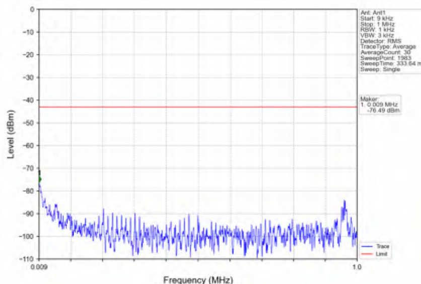
n78e 15kHz SISO NTN 15MHz DFT-s-OFDM QPSK 3457.5MHz Outer Full
