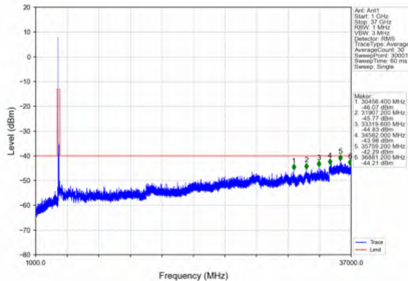
n78d_30kHz_SISO_NTNV_100MHz_DFT-s-OFDM_QPSK_3600MHz_Inner_1RB_Left
