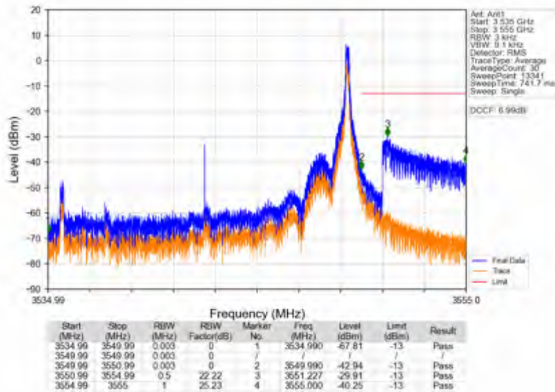
n78e_15kHz_SISO_NTNV_15MHz_DFT-s-OFDM QPSK_3542.49MHz_Inner_1RB_Right
