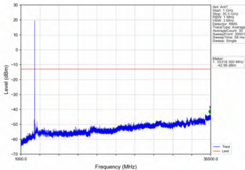
n78e_15kHz_SISO_NTNV_10MHz_DFT-s-OFDM_QPSK_3544.995MHz_Edge_1RB_Right
