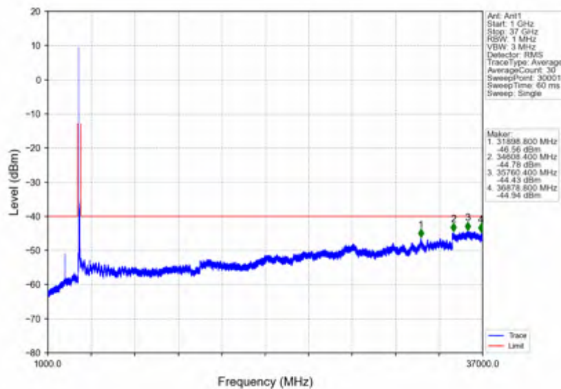
n78d_30kHz_SISO_NTV_90MHz_CP-OFDM QPSK_3624.99MHz_Edge_1RB_Left
