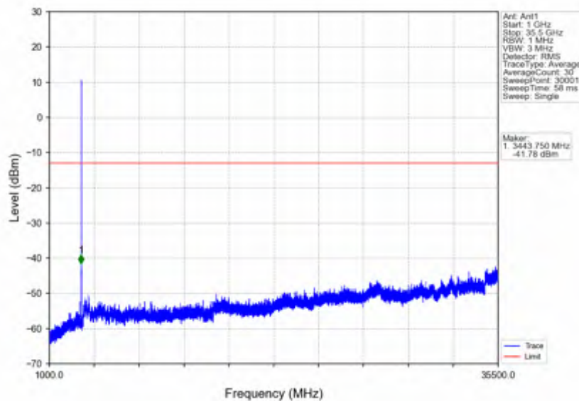
n78e_15kHz_SISO_NTNV_15MHz_DFT-s-OFDM QPSK_3457.5MHz_Inner_1RB_Left
