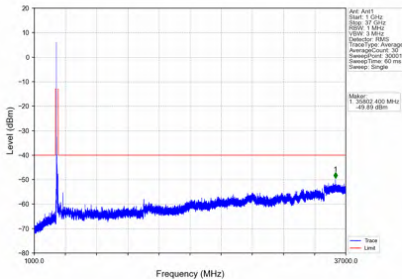
n78d_30kHz_SISO_NTNV_100MHz_DFT-s-OFDM PI/2 BPSK_3600MHz_Outer_Full
