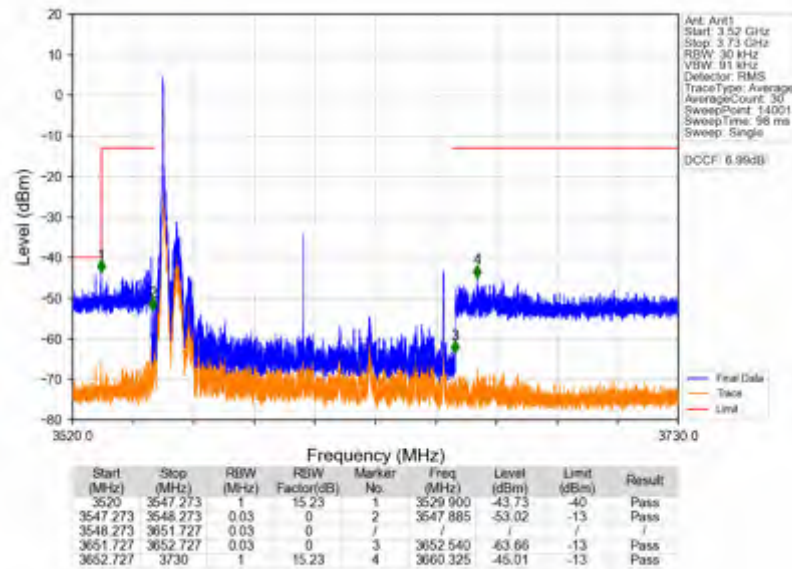
n78d_30kHz_SISO_NTNV_100MHz_CP-OFDM QPSK_3600MHz_Inner_1RB_Left
