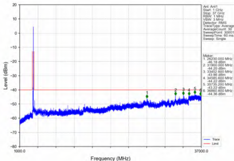
n78d_30kHz_SISO_NTNV_100MHz_CP-OFDM QPSK_3649.98MHz_Outer_Full
