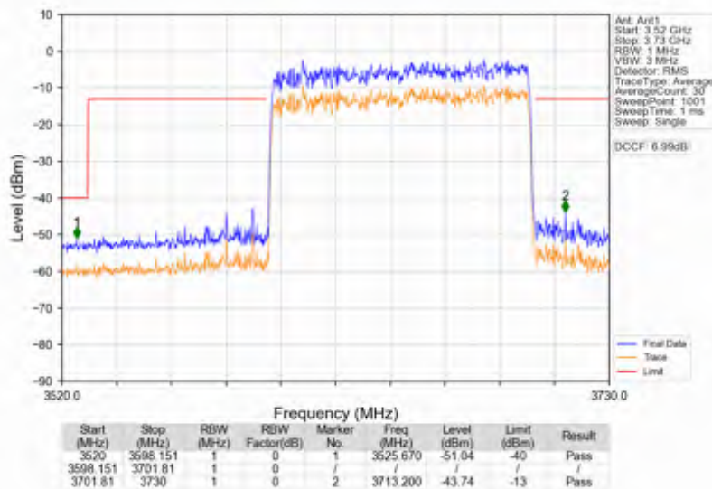
n78d_30kHz_SISO_NTNV_100MHz_CP-OFDM QPSK_3649.98MHz_Outer_Full
