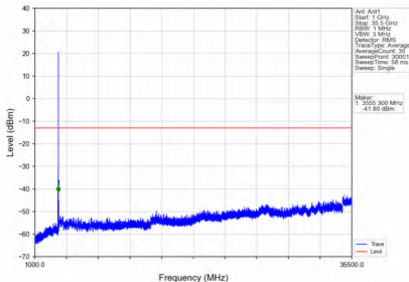
n78e_15kHz_SISO_NTNV_10MHz_CP-OFDM QPSK_3544.995MHz_Outer_Full
