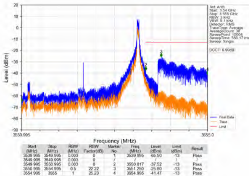
n78e_15kHz_SISO_NTNV_10MHz_DFT-s-OFDM QPSK_3544.995MHz_Inner_1RB_Right
