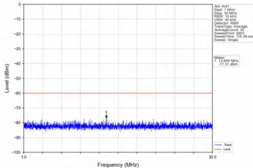
n78d_30kHz_SISO_NTNV_90MHz_DFT-s-OFDM QPSK_3654.99MHz_Edge_1RB_Right
