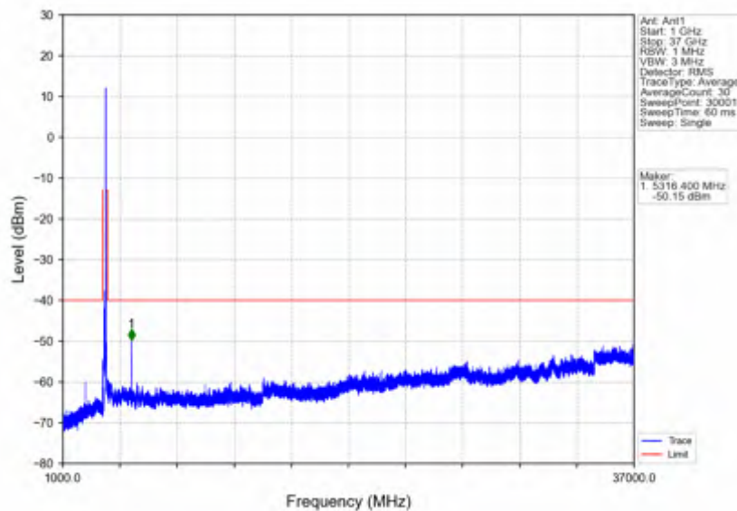
n78d_30kHz_SISO_NTNV_100MHz_DFT-s-OFDM PI/2 BPSK_3649.98MHz_Outer_Full
