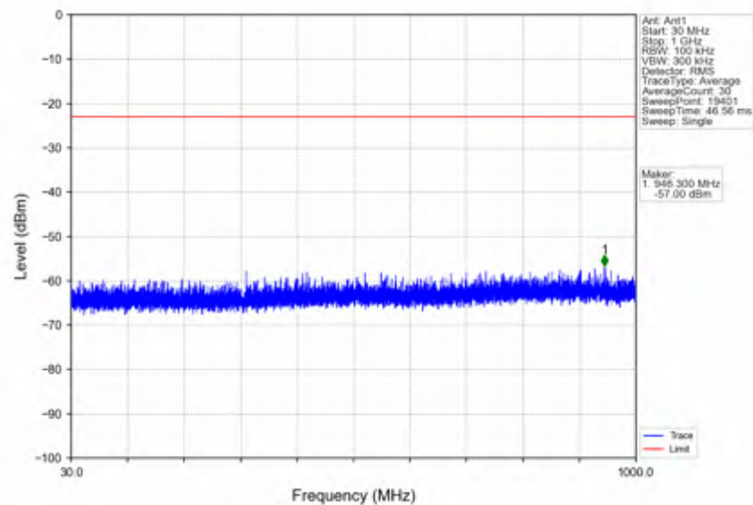
n78e_15kHz_SISO_NTNV_15MHz_DFT-s-OFDM QPSK_3499.995MHz_Edge_1RB_Left
