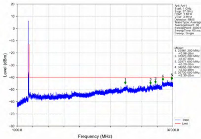
n78d_30kHz_SISO_NTNV_90MHz_DFT-s-OFDM QPSK_3654.99MHz_Edge_1RB_Right
