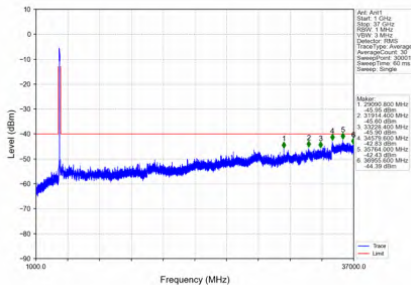
n78d 30kHz SISO NTNv 90MHz CP-OFDM QPSK 3654.99MHz Outer Full
