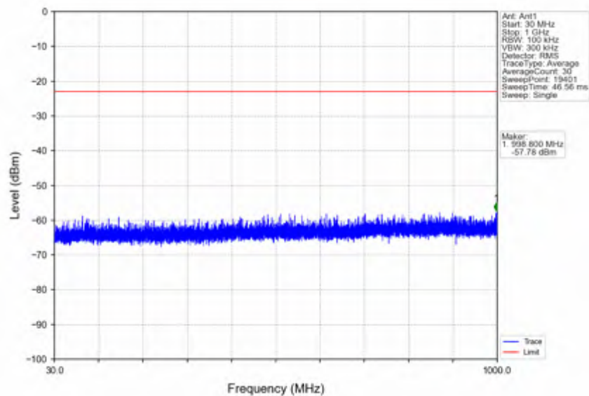
n78e_15kHz_SISO_NTNV_10MHz_DFT-s-OFDM_QPSK_3455.01MHz_Edge_1RB_Left
