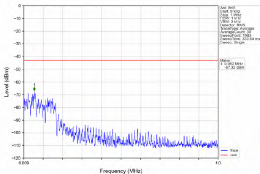
n78e_15kHz_SISO_NTNV_10MHz_DFT-s-OFDM PI/2 BPSK_3455.01MHz_Edge_1RB_Left
