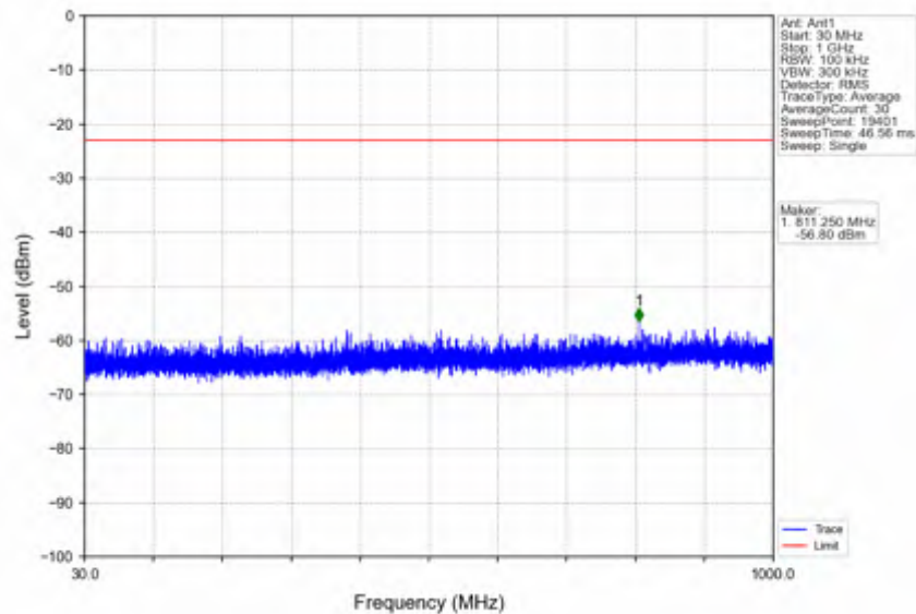
n78e_15kHz_SISO_NTNV_15MHz_DFT-s-OFDM QPSK_3457.5MHz_Edge_1RB_Left
