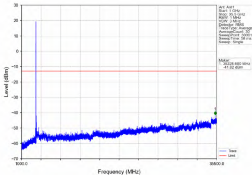
n78e_15kHz_SISO_NTNV_10MHz_DFT-s-OFDM PI/2 BPSK_3544.995MHz_Outer_Full
