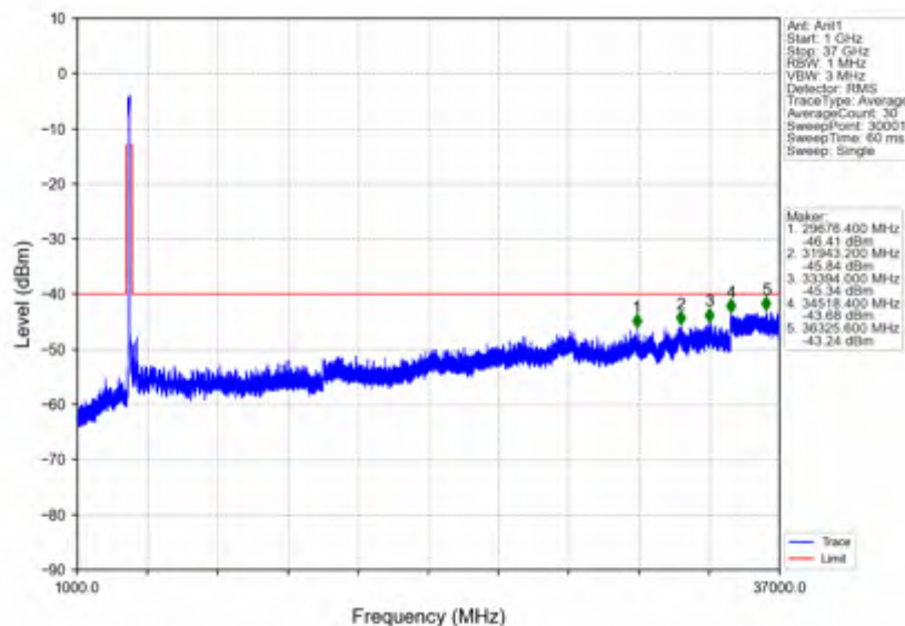
n78d_30kHz_SISO_NTNV_100MHz_DFT-s-OFDM QPSK_3649.98MHz_Inner_1RB_Right
