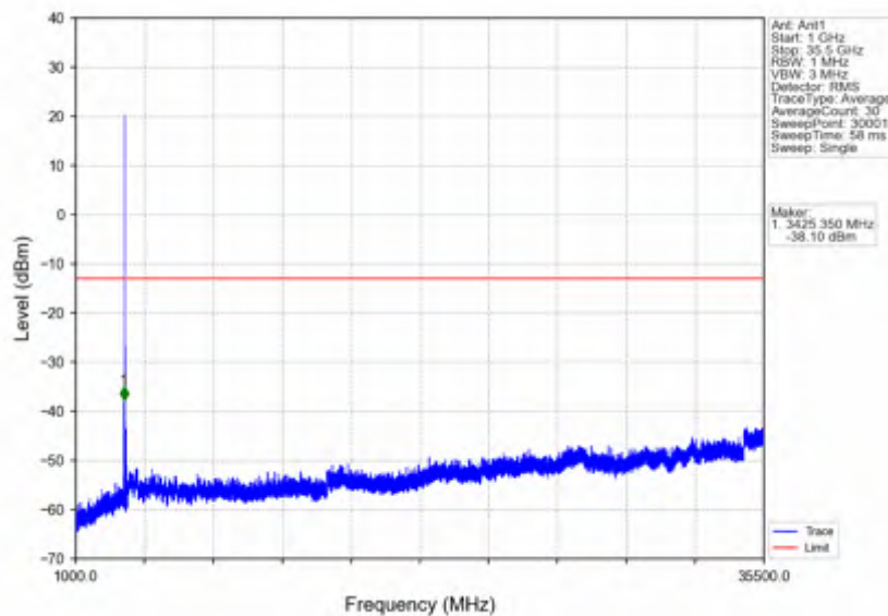
n78e_15kHz_SISO_NTNV_10MHz_DFT-s-OFDM_QPSK_3455.01MHz_Edge_1RB_Left
