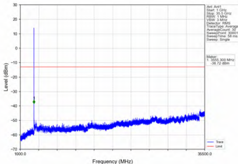
n78e_15kHz_SISO_NTNV_10MHz_DFT-s-OFDM QPSK_3544.995MHz_Inner_1RB_Right
