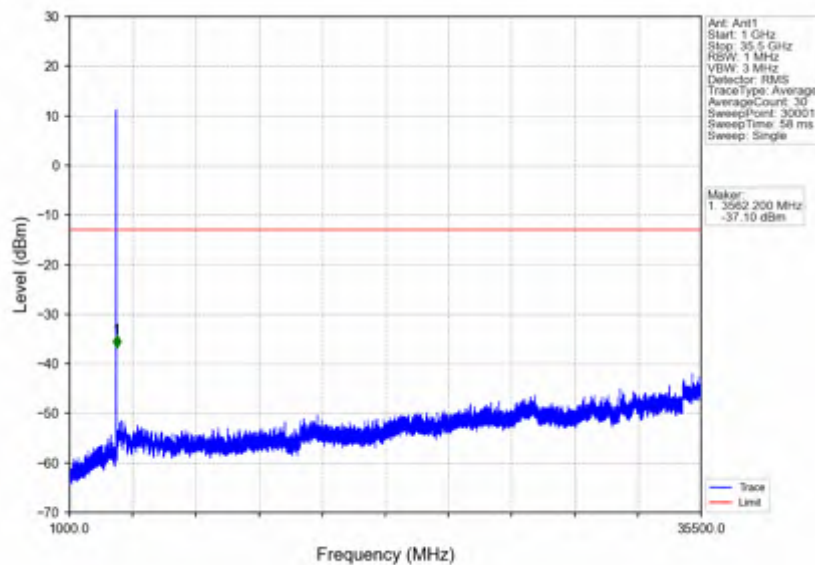
n78e_15kHz_SISO_NTNV_15MHz_DFT-s-OFDM QPSK_3542.49MHz_Inner_1RB_Right
