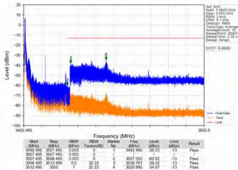
n78e_15kHz_SISO_NTNV_15MHz_CP-OFDM QPSK_3499.995MHz_Edge_1RB_Left
