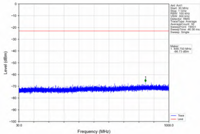
n78e_15kHz_SISO_NTNV_15MHz_CP-OFDM QPSK_3542.49MHz_Inner_1RB_Right
