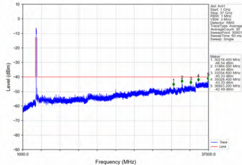
n78d_30kHz_SISO_NTNV_100MHz_CP-OFDM QPSK_3600MHz_Outer_Full
