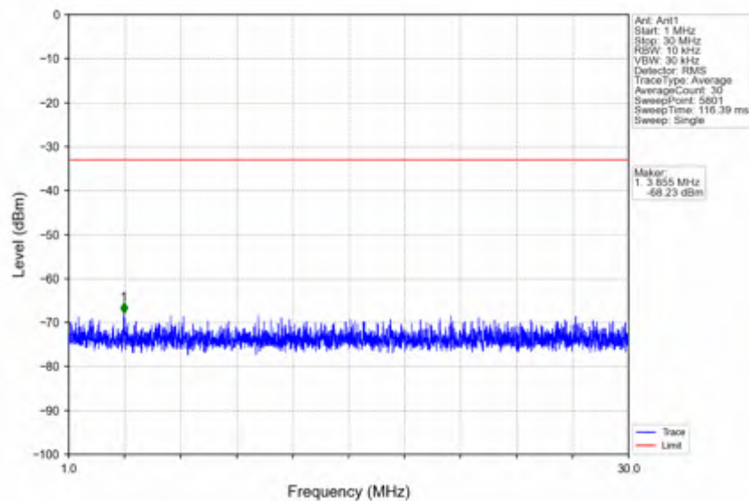
n78e_15kHz_SISO_NTNV_15MHz_CP-OFDM QPSK_3542.49MHz_Edge_1RB_Right
