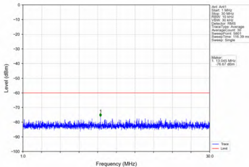
n78d_30kHz_SISO_NTNV_100MHz_CP-OFDM QPSK_3600MHz_Outer_Full
