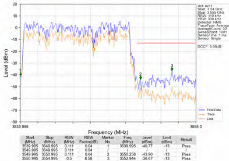
n78e_15kHz_SISO_NTNV_10MHz_DFT-s-OFDM PI/2 BPSK_3544.995MHz_Outer_Full
