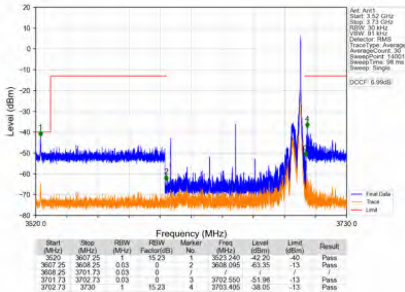
n78d_30kHz_SISO_NTNV_90MHz_DFT-s-OFDM QPSK_3654.99MHz_Edge_1RB_Right
