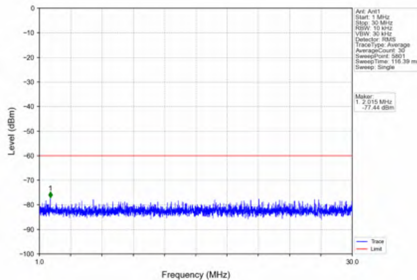
n78d_30kHz_SISO_NTNV_100MHz_DFT-s-OFDM QPSK_3624.99MHz_Edge_1RB_Left
