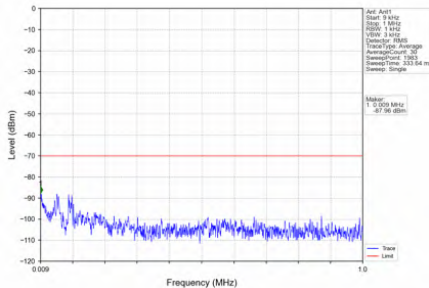
n78d_30kHz_SISO_NTNV_90MHz_CP-OFDM_QPSK_3595.02MHz_Outer_Full
