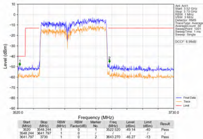
n78d 30kHz SISO NTNv 90MHz CP-OFDM QPSK 3595.02MHz Outer Full
