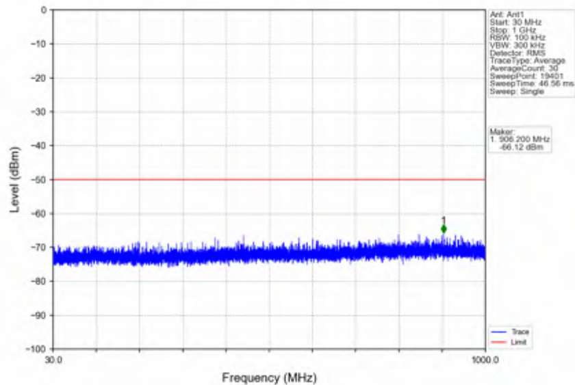
n78d_30kHz_SISO_NTNV_100MHz_CP-OFDM QPSK_3600MHz_Outer_Full
