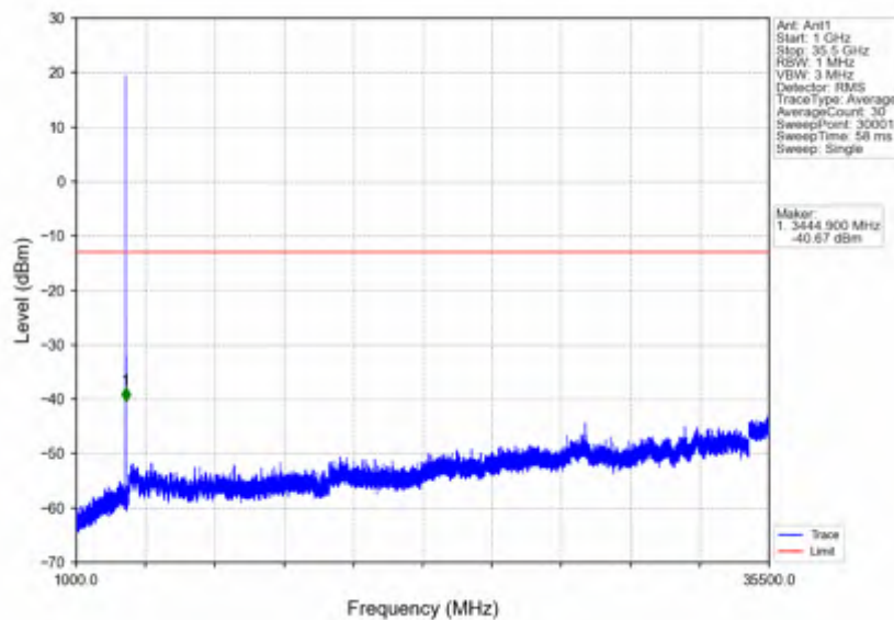
n78e_15kHz_SISO_NTNV_10MHz_CP-OFDM_QPSK_3455.01MHz_Outer_Full
