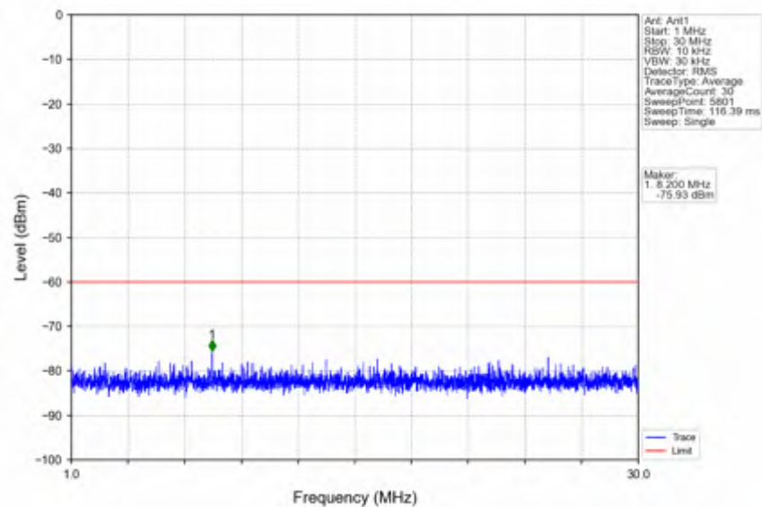
n78d_30kHz_SISO_NTNV_100MHz_DFT-s-OFDM QPSK_3600MHz_Inner_1RB_Left
