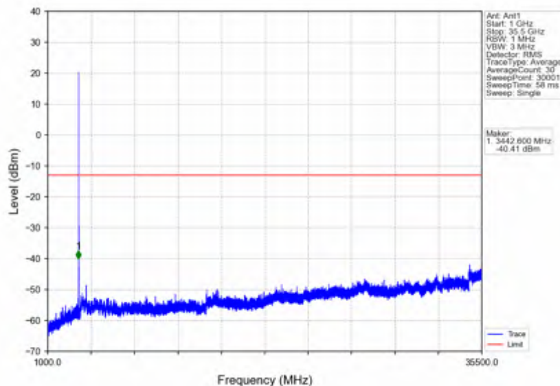
n78e_15kHz_SISO_NTNV_15MHz_CP-OFDM QPSK_3457.5MHz_Outer_Full
