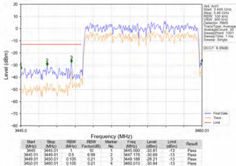
n78e_15kHz_SISO_NTNV_10MHz_CP-OFDM_QPSK_3455.01MHz_Outer_Full
