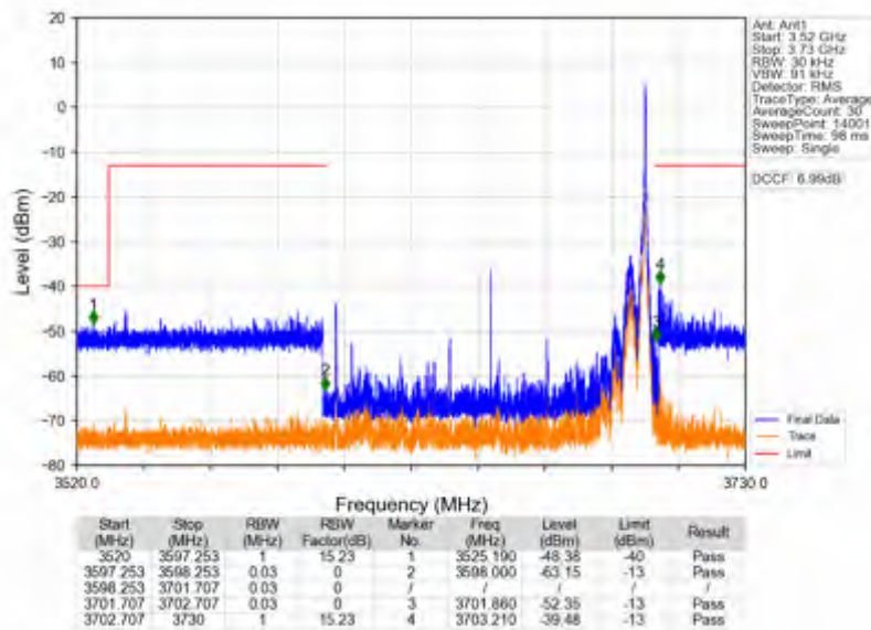
n78d_30kHz_SISO_NTNV_100MHz_DFT-s-OFDM QPSK_3649.98MHz_Inner_1RB_Right
