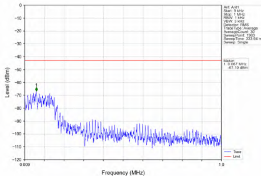
n78e_15kHz_SISO_NTNV_15MHz_DFT-s-OFDM_QPSK_3499.995MHz_Edge_1RB_Left
