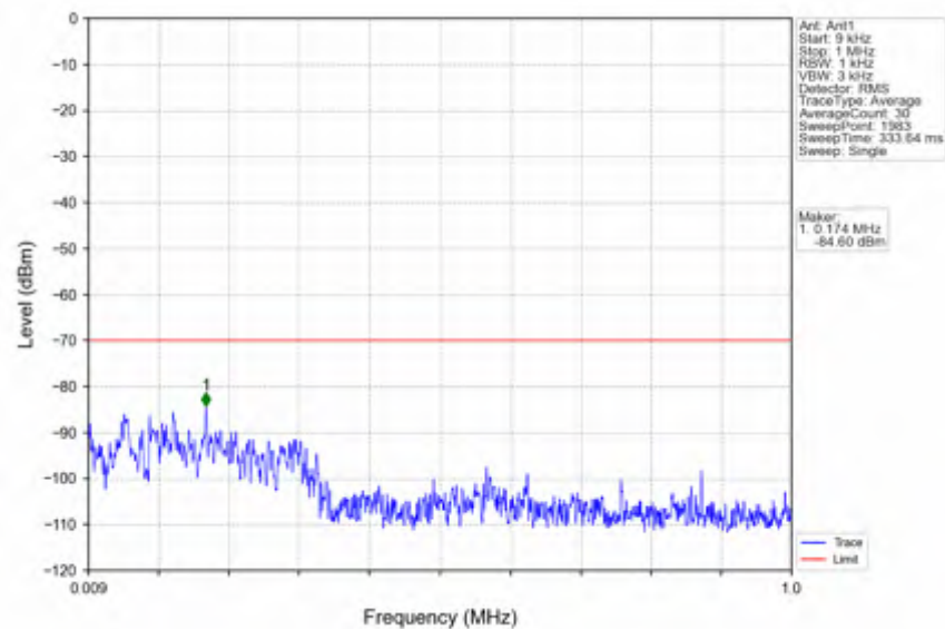
n78d_30kHz_SISO_NTNV_90MHz_DFT-s-OFDM QPSK_3654.99MHz_Inner_1RB_Right
