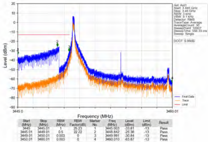
n78e_15kHz_SISO_NTNV_10MHz_DFT-s-OFDM QPSK_3455.01MHz_Edge_1RB_Left
