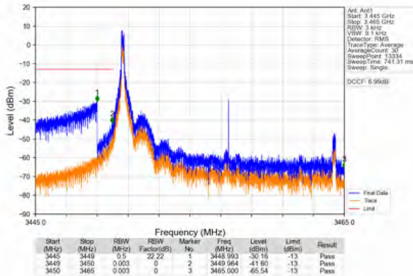
n78e_15kHz_SISO_NTNV_15MHz_DFT-s-OFDM QPSK_3457.5MHz_Inner_1RB_Left
