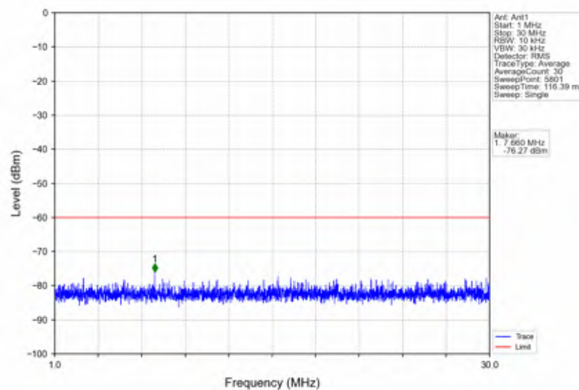
n78d_30kHz_SISO_NTNV_90MHz_CP-OFDM_QPSK_3595.02MHz_Outer_Full
