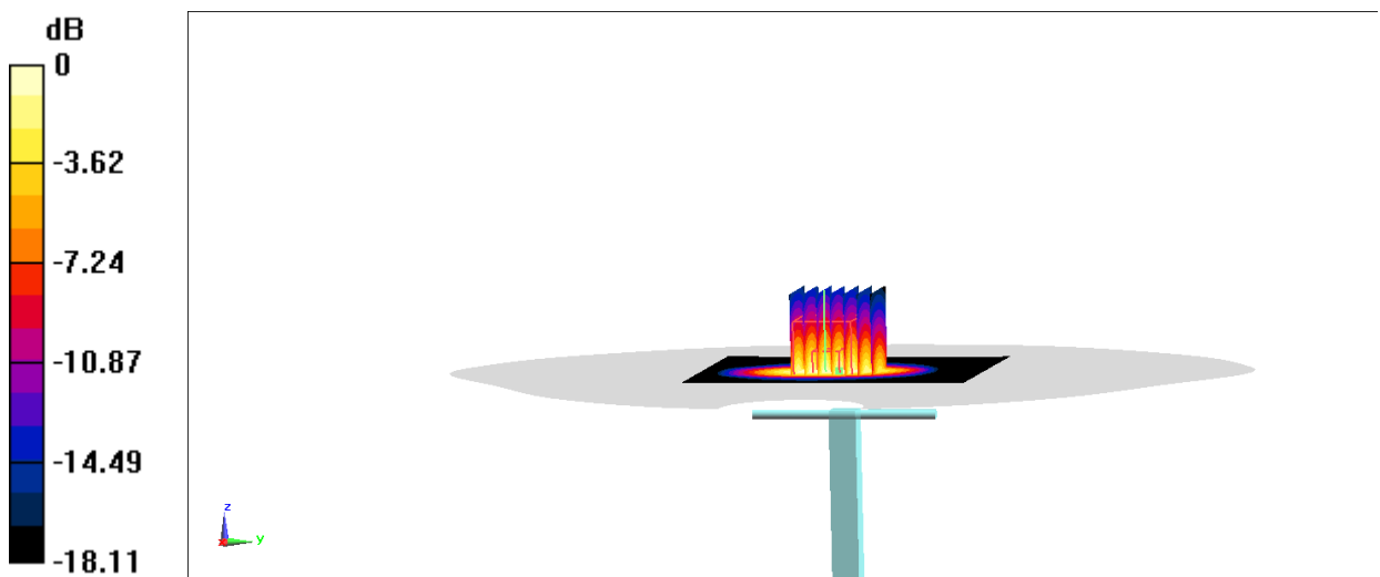
Fig.B.9 validation 1900 MHz 250mW
