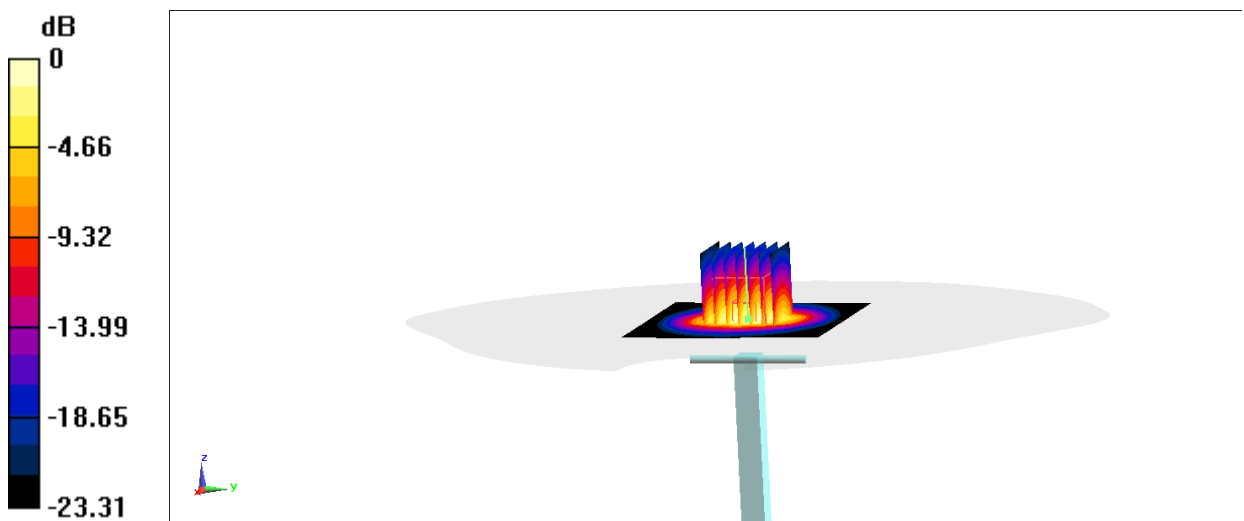
Fig.B.14 validation 2600 MHz 250mW
