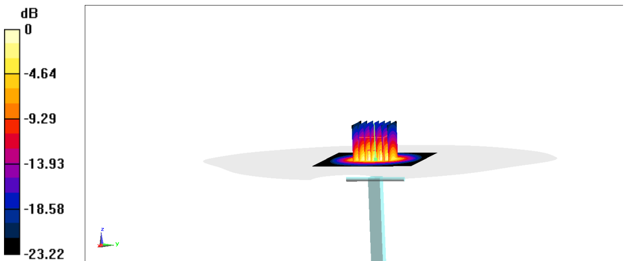
Fig.B.13 validation 2600 MHz 250mW
