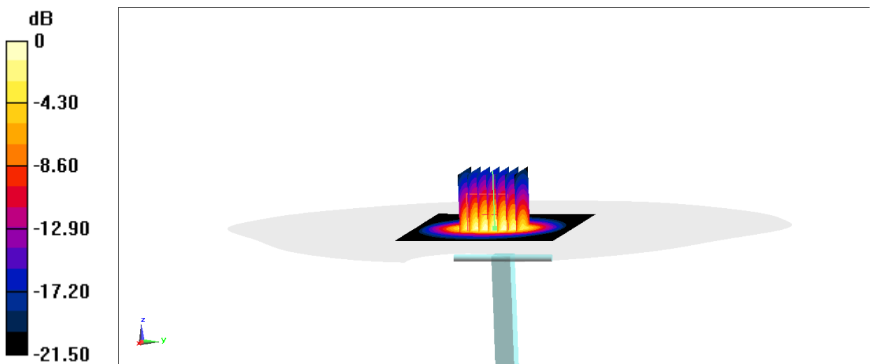
Fig.B.15 validation 2450 MHz 250mW
