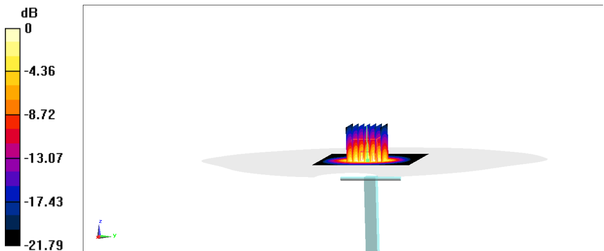
Fig.B.10 validation 2450 MHz 250mW
