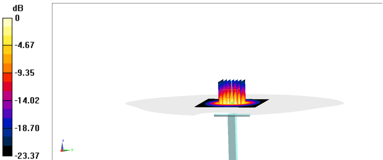
Fig.B.12 validation 2600 MHz 250mW
