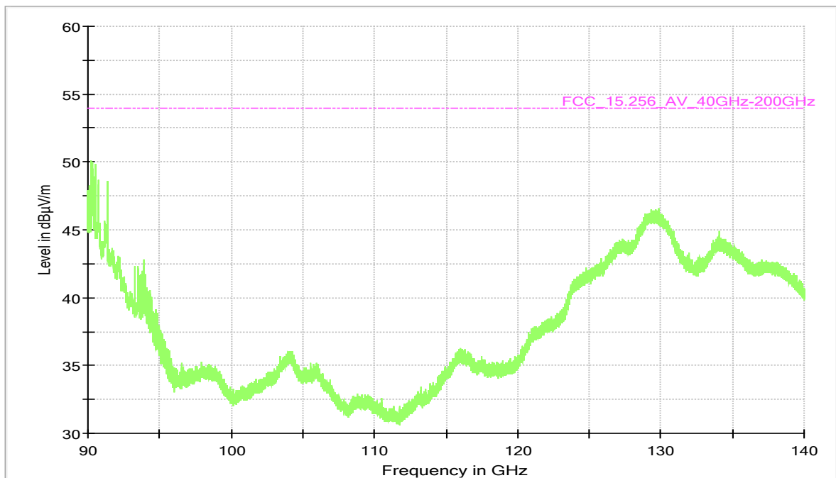
S01_AC01 90 GHz – 140 GHz
