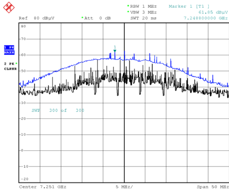
Radiated Spurious Emissions plot – Peak Reading (802.11g, Ch.2 3rd Harmonic)
