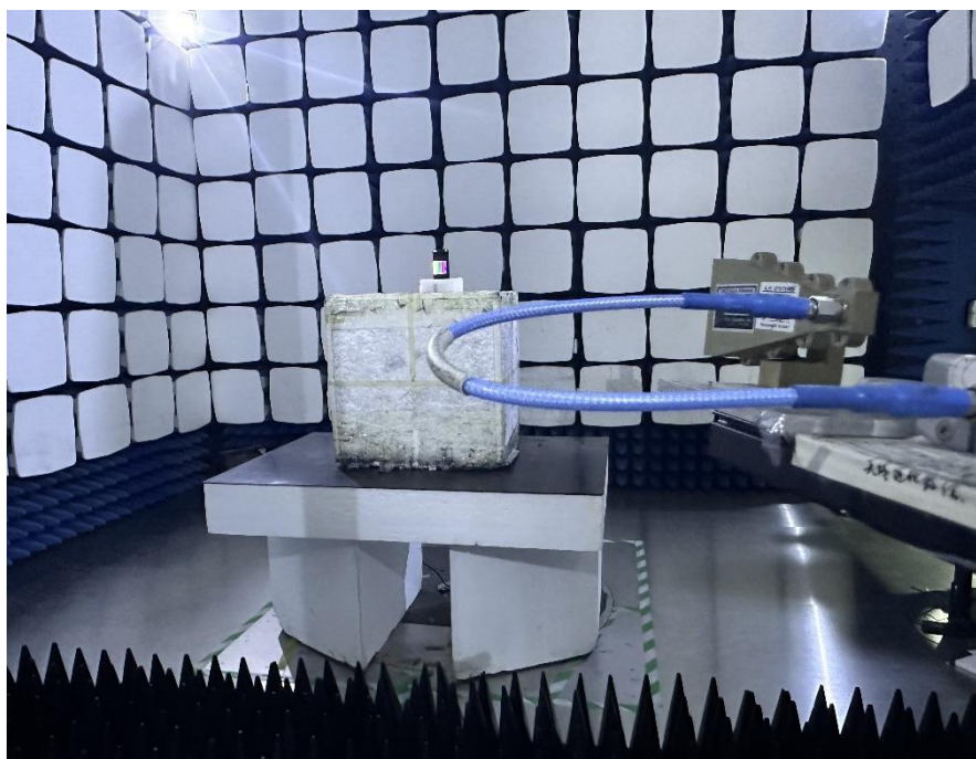
Radiation Emission Test Setup (Above18GHz)
