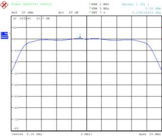
Figure 5-7: Peak Power Spectral Density 802.11n, Channel 36, MCS 0
