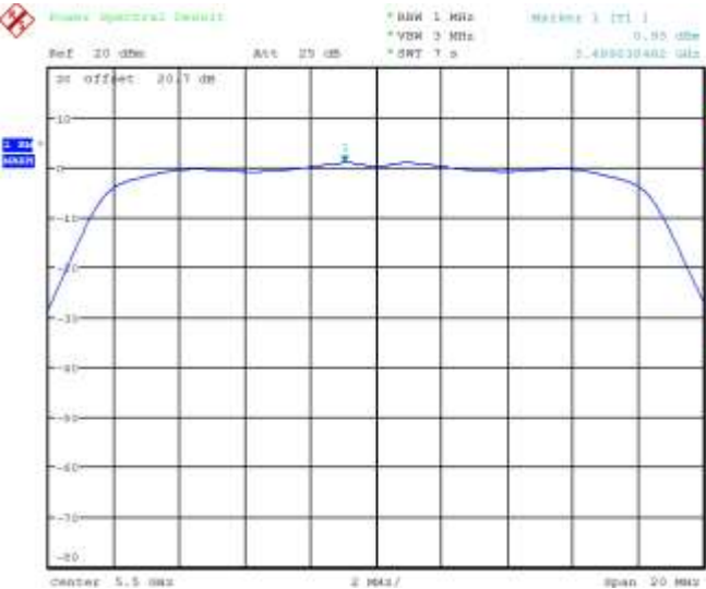
Figure 5-4: Peak Power Spectral Density 802.11a, Channel 100, 6 Mbps
