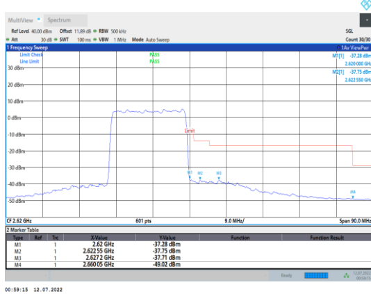
Band38-20MHz-16QAM-38150-100RB#0
