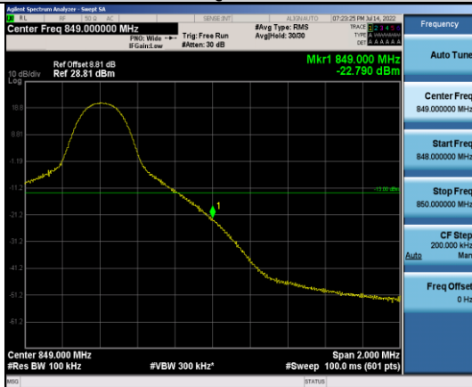
Band5-10MHz-QPSK-20600-1RB#49
