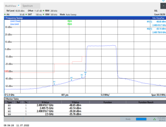
Band7-10MHz-16QAM-20800-50RB#0
