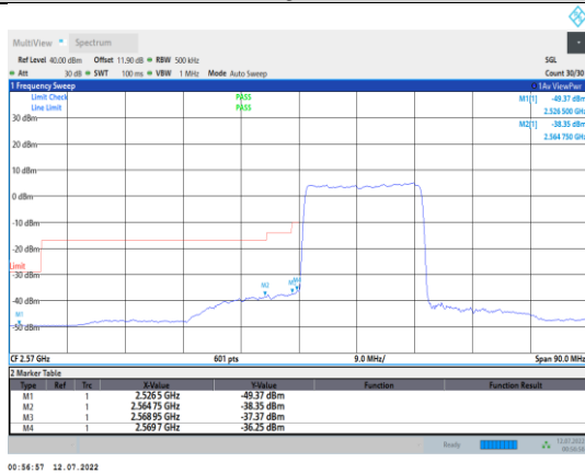
Band38-20MHz-QPSK-37850-100RB#0
