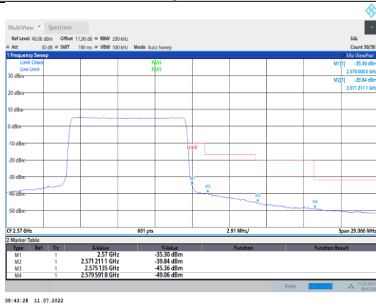
Band7-10MHz-QPSK-21400-50RB#0
