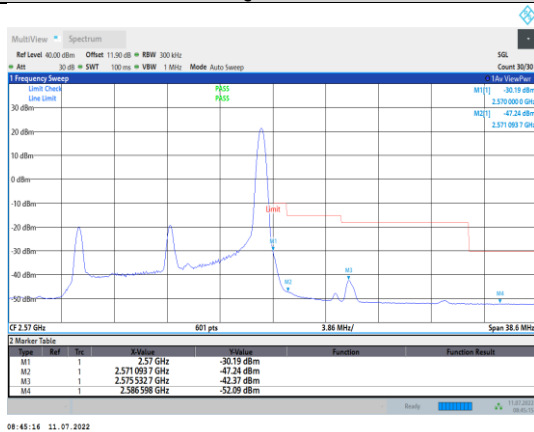
Band7-15MHz-QPSK-21375-1RB#74
