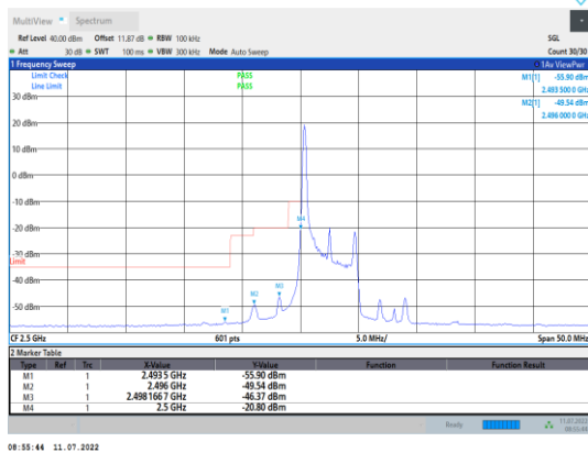
Band7-5MHz-16QAM-20775-1RB#0
