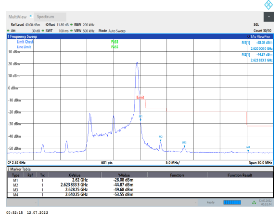
Band38-10MHz-QPSK-38200-1RB#49
