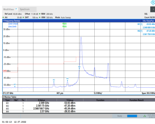
Band38-10MHz-QPSK-37800-1RB#0
