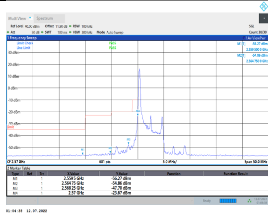
Band38-5MHz-16QAM-37775-1RB#0
