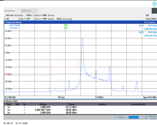
Band41-10MHz-QPSK-39700-1RB#0
