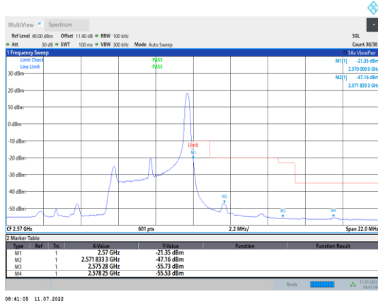
Band7-5MHz-16QAM-21425-1RB#24
