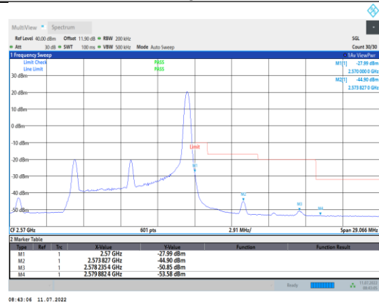
Band7-10MHz-16QAM-21400-1RB#49
