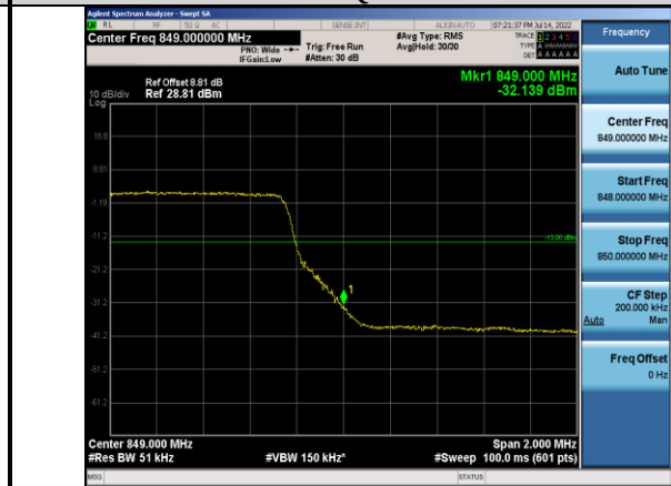
Band5-5MHz-16QAM-20625-25RB#0
