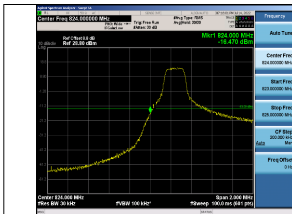
Band5-3MHz-16QAM-20415-1RB#0
