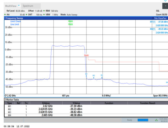
Band38-20MHz-QPSK-38150-100RB#0
