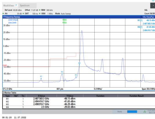
Band7-15MHz-QPSK-20825-1RB#0
