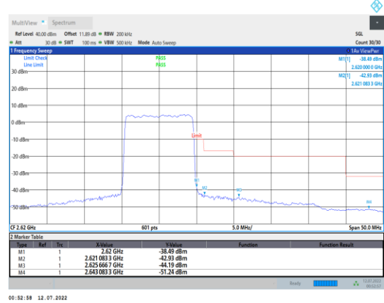
Band38-10MHz-QPSK-38200-50RB#0
