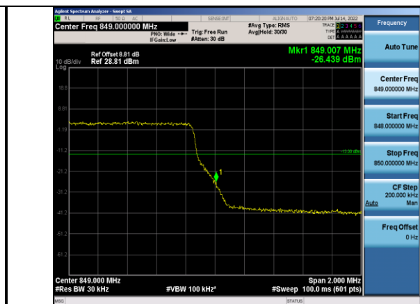
Band5-3MHz-16QAM-20635-15RB#0
