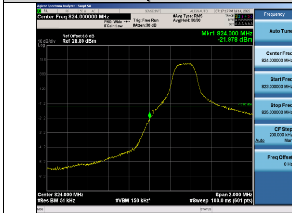
Band5-5MHz-16QAM-20425-1RB#0
