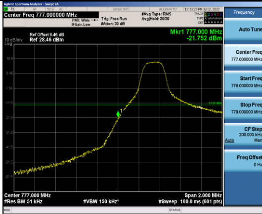
Band13-5MHz-16QAM-23205-1RB#0
