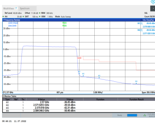
Band7-15MHz-16QAM-21375-75RB#0
