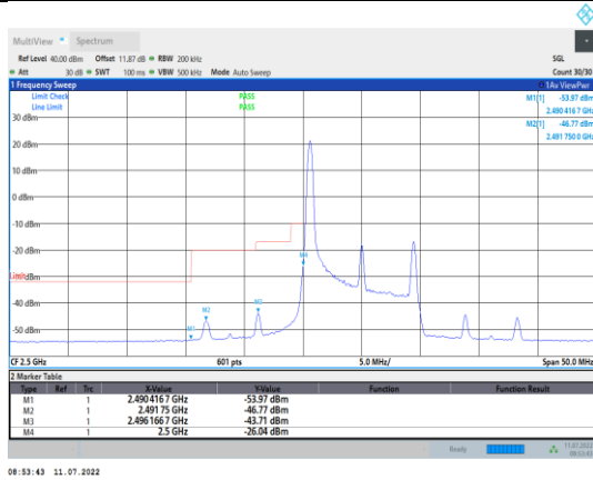
Band7-10MHz-16QAM-20800-1RB#0
