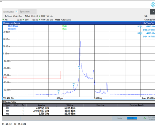
Band41-5MHz-QPSK-39675-1RB#0
