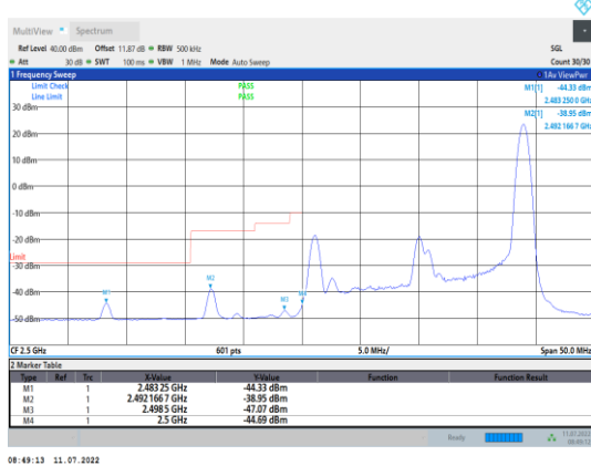
Band7-20MHz-QPSK-20850-1RB#99
