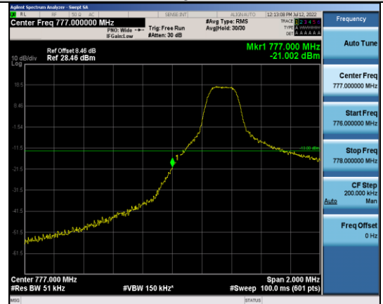
Band13-5MHz-QPSK-23205-1RB#0
