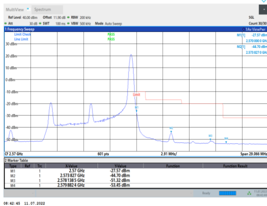
Band7-10MHz-QPSK-21400-1RB#49
