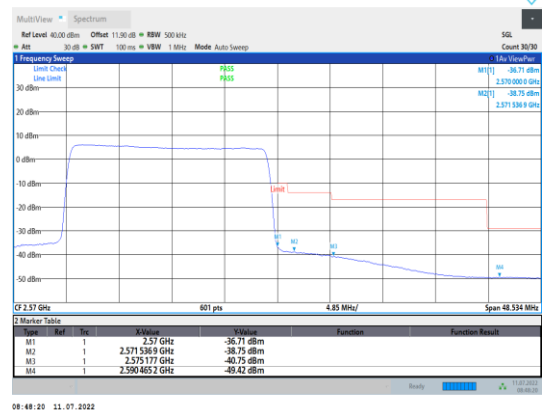
Band7-20MHz-16QAM-21350-100RB#0
