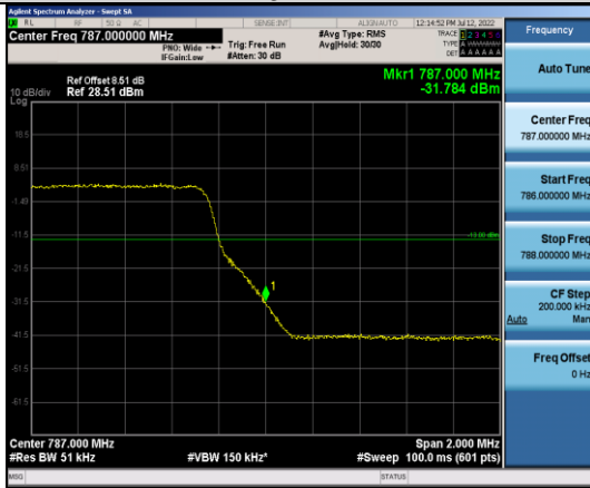
Band13-5MHz-QPSK-23255-25RB#0
