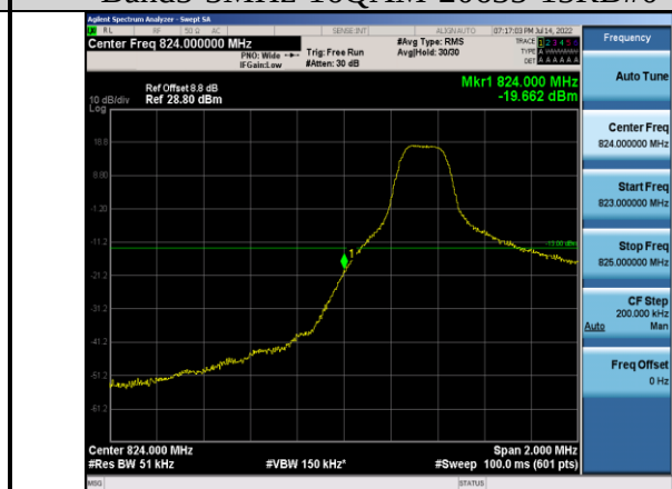
Band5-5MHz-QPSK-20425-1RB#0
