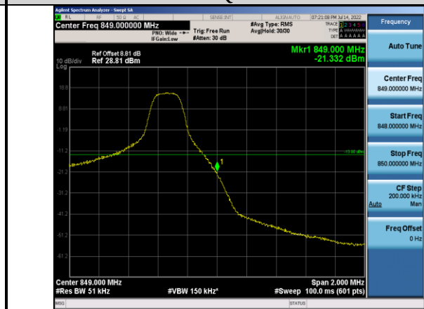
Band5-5MHz-16QAM-20625-1RB#24
