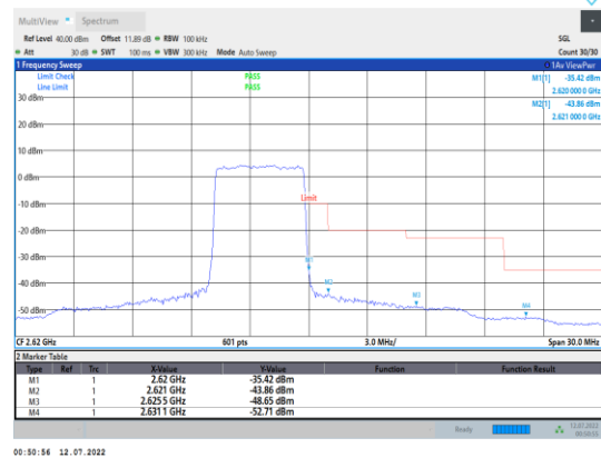
Band38-5MHz-QPSK-38225-25RB#0
