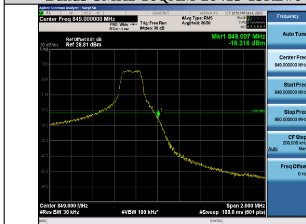
Band5-3MHz-16QAM-20635-1RB#14
