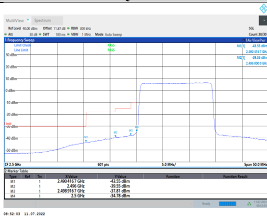
Band7-15MHz-QPSK-20825-75RB#0
