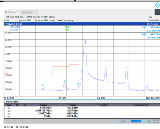
Band7-15MHz-16QAM-20825-1RB#0
