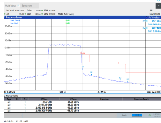
Band41-5MHz-16QAM-41565-25RB#0
