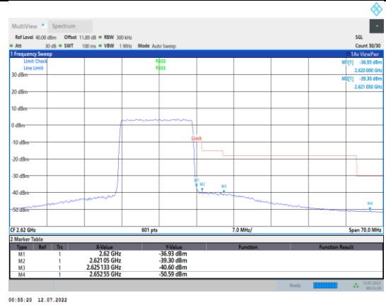
Band38-15MHz-16QAM-38175-75RB#0
