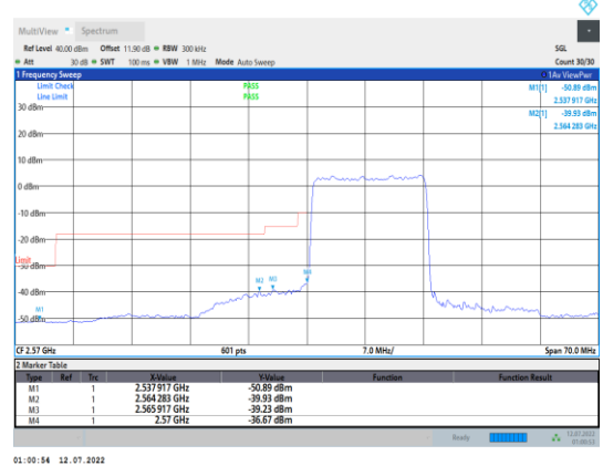
Band38-15MHz-QPSK-37825-75RB#0
