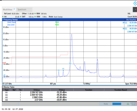
Band38-15MHz-16QAM-37825-1RB#0
