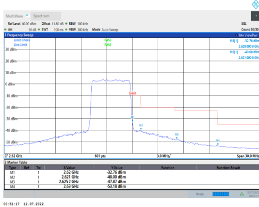
Band38-5MHz-16QAM-38225-25RB#0
