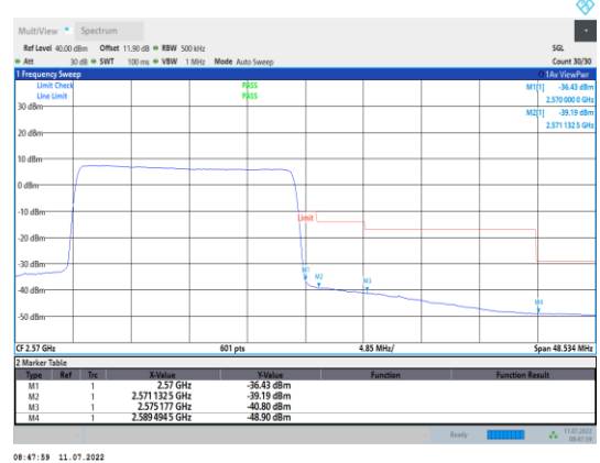
Band7-20MHz-QPSK-21350-100RB#0
