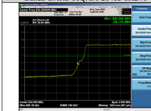
Band5-3MHz-16QAM-20415-15RB#0
