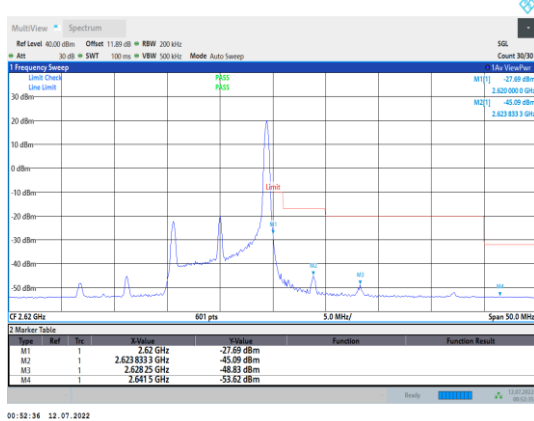
Band38-10MHz-16QAM-38200-1RB#49
