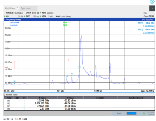
Band38-15MHz-QPSK-37825-1RB#0
