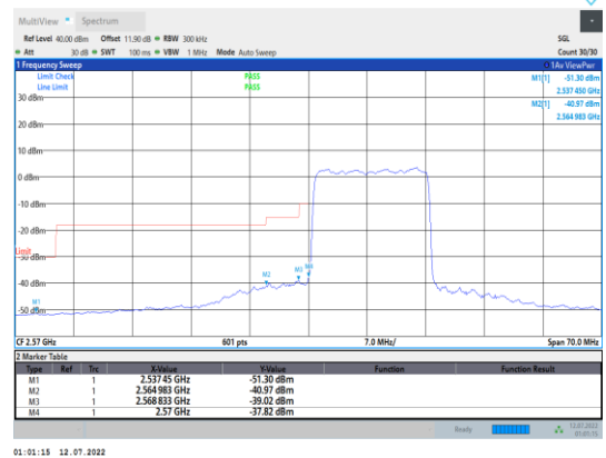
Band38-15MHz-16QAM-37825-75RB#0
