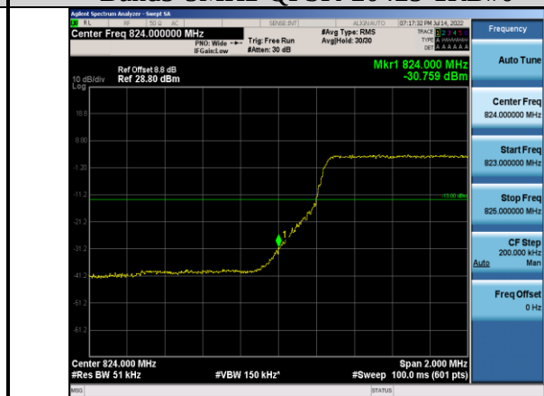
Band5-5MHz-QPSK-20425-25RB#0
