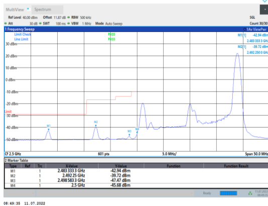
Band7-20MHz-16QAM-20850-1RB#99
