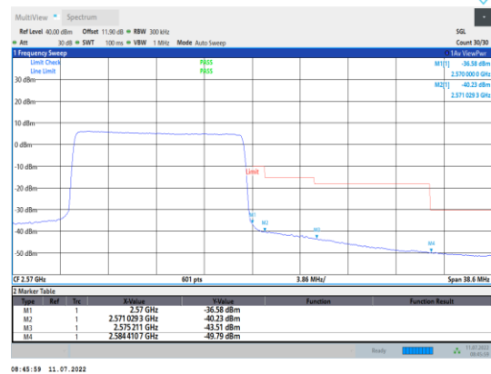
Band7-15MHz-QPSK-21375-75RB#0
