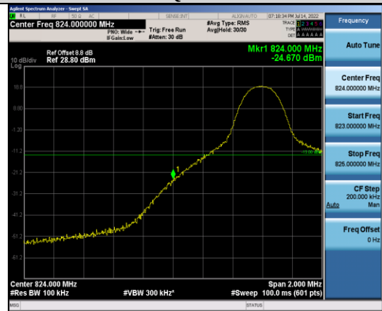
Band5-10MHz-16QAM-20450-1RB#0
