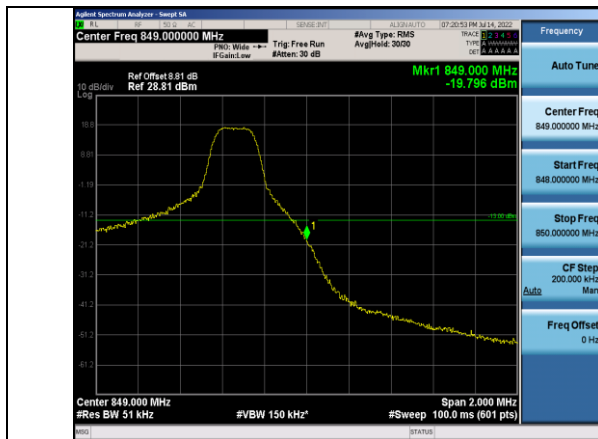
Band5-5MHz-QPSK-20625-1RB#24
