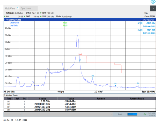
Band41-5MHz-QPSK-41565-1RB#24
