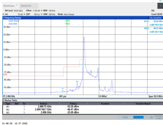
Band41-5MHz-16QAM-39675-1RB#0
