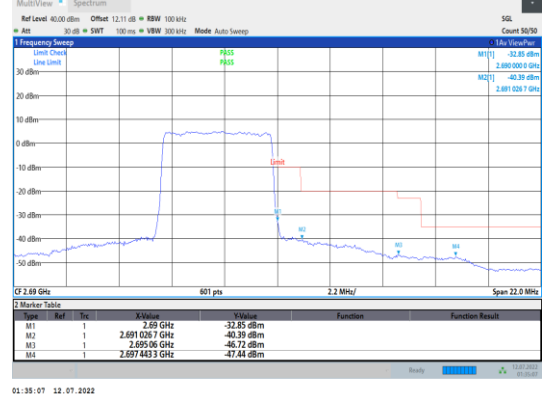
Band41-5MHz-QPSK-41565-25RB#0
