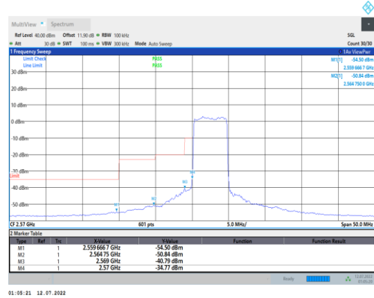
Band38-5MHz-16QAM-37775-25RB#0
