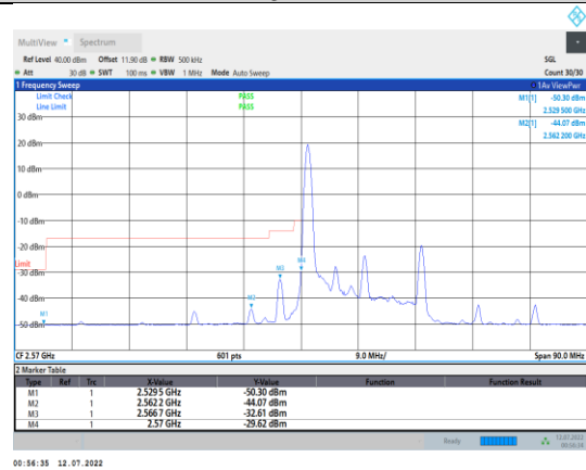
Band38-20MHz-16QAM-37850-1RB#0
