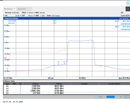
Band38-20MHz-16QAM-37850-100RB#0
