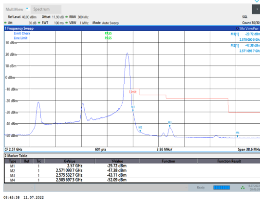
Band7-15MHz-16QAM-21375-1RB#74
