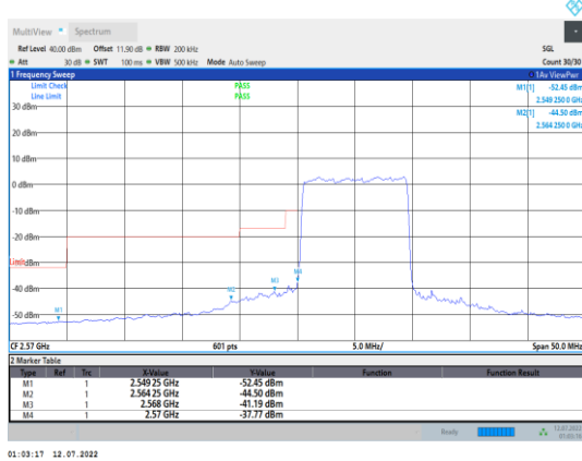
Band38-10MHz-16QAM-37800-50RB#0
