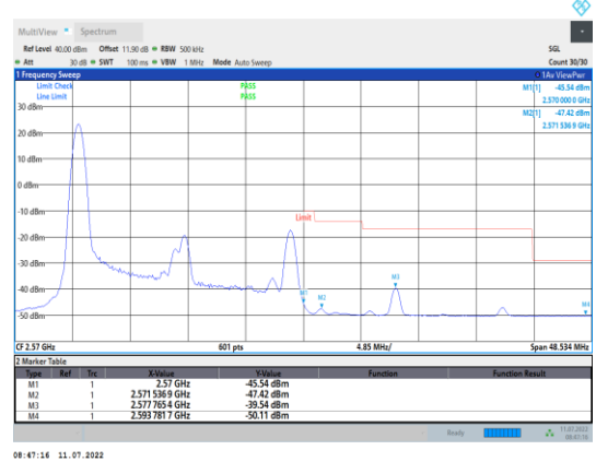
Band7-20MHz-QPSK-21350-100RB#0
