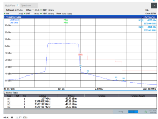
Band7-5MHz-16QAM-21425-25RB#0
