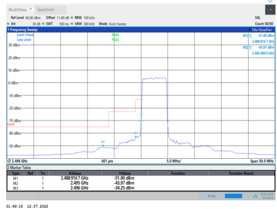
Band41-5MHz-QPSK-39675-25RB#0
