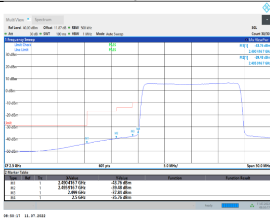
Band7-20MHz-16QAM-20850-100RB#0
