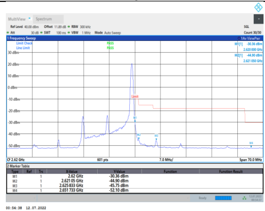
Band38-15MHz-16QAM-38175-1RB#74
