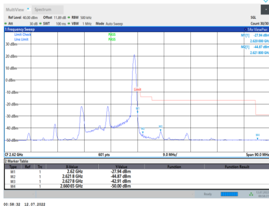
Band38-20MHz-16QAM-38150-1RB#99
