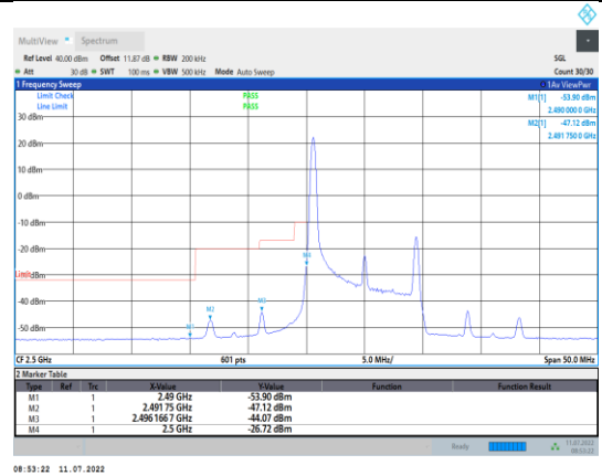
Band7-10MHz-QPSK-20800-1RB#0
