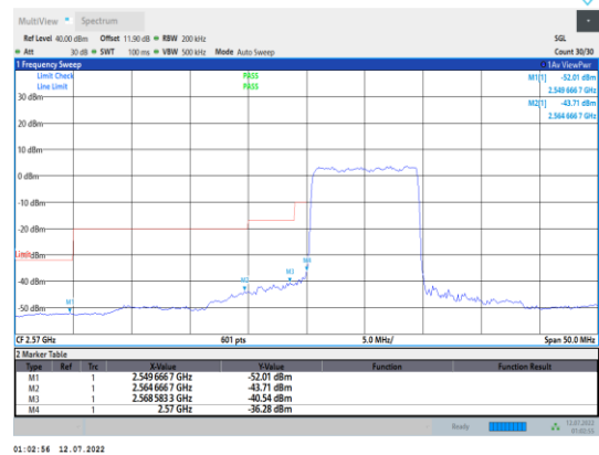
Band38-10MHz-QPSK-37800-50RB#0
