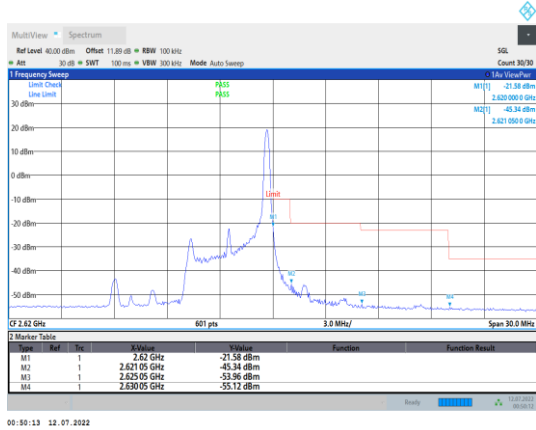
Band38-5MHz-QPSK-38225-1RB#24
