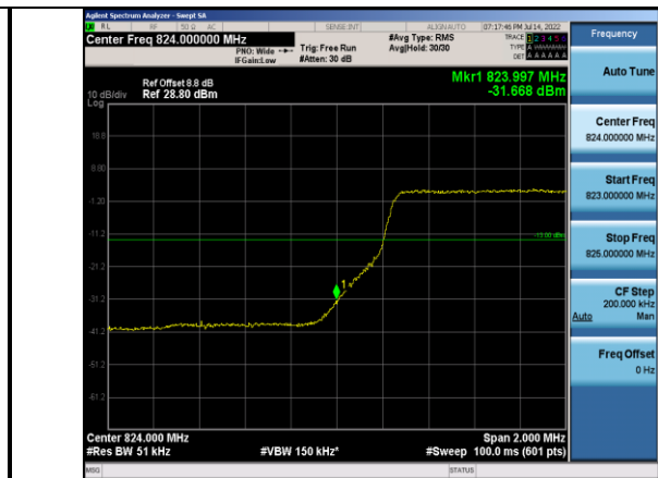
Band5-5MHz-16QAM-20425-25RB#0
