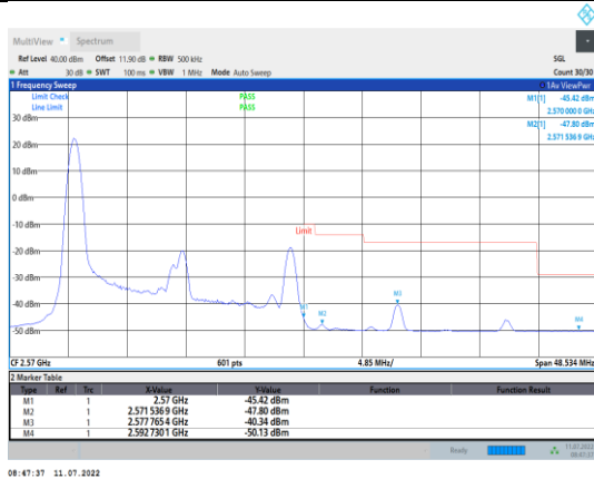
Band7-20MHz-16QAM-21350-1RB#0
