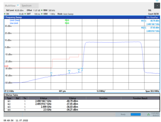
Band7-20MHz-QPSK-20850-100RB#0
