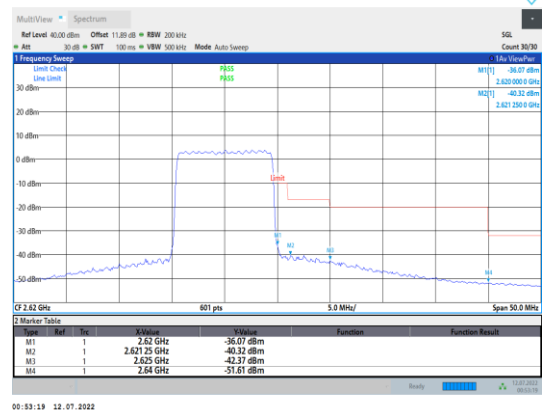
Band38-10MHz-16QAM-38200-50RB#0
