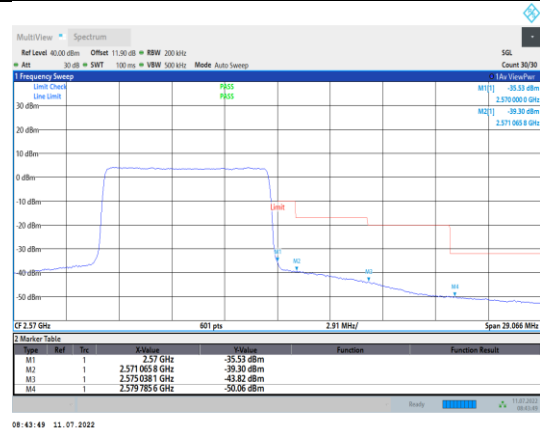
Band7-10MHz-16QAM-21400-50RB#0
