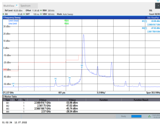
Band38-10MHz-16QAM-37800-1RB#0
