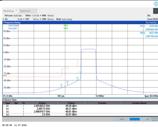
Band7-5MHz-16QAM-20775-25RB#0
