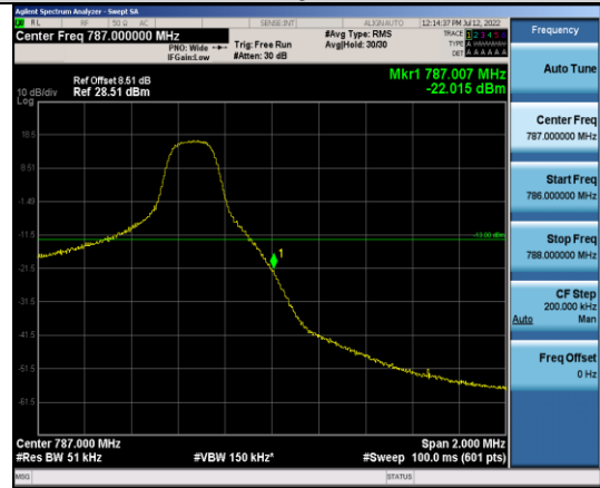
Band13-5MHz-16QAM-23255-1RB#24
