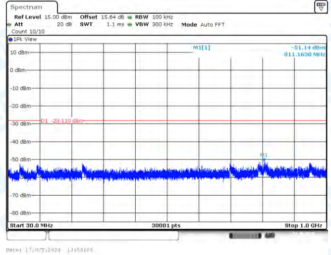
11AX20SISO-Ant1-2462-30~1000-PASS
