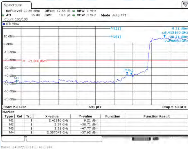
11AX40ISO-Ant1-2422-PASS
