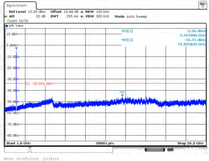
11N40SISO-Ant1-2422-1000~26500-PASS
