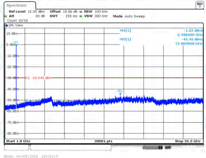
11AX20SISO-Ant1-2437-1000~26500-PASS
