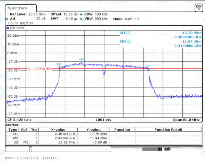
11N40SISO-Ant1-2422-PASS
