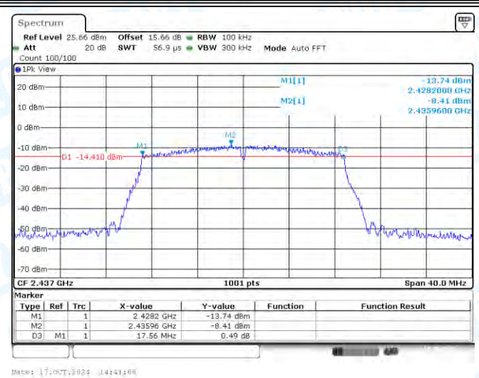
11N20SISO-Ant1-2437-PASS
