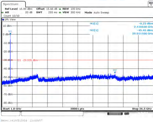
11N20SISO-Ant1-2412-1000~26500-PASS
