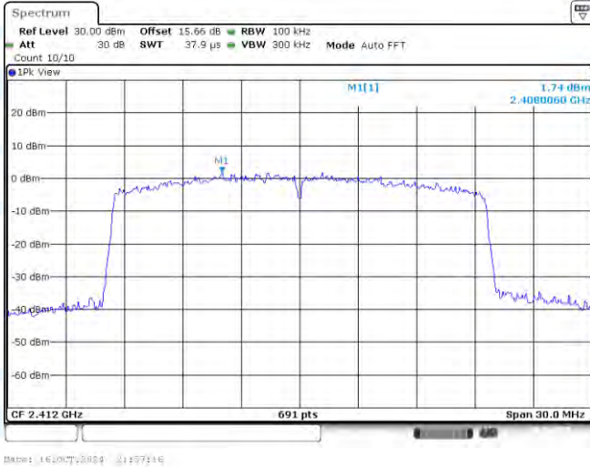
11AX20SISO-Ant1-2412-0~Reference-PASS
