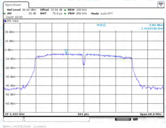
11N40SISO-Ant1-2422-0~Reference-PASS
