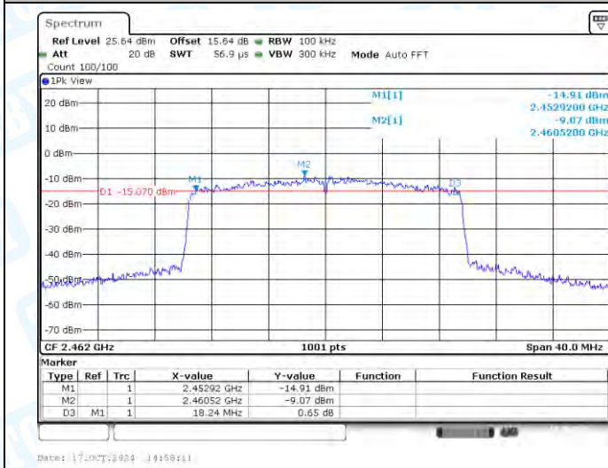
11AX20SISO-Ant1-2462-PASS
