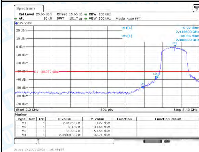
11N20SISO-Ant1-2412-PASS
