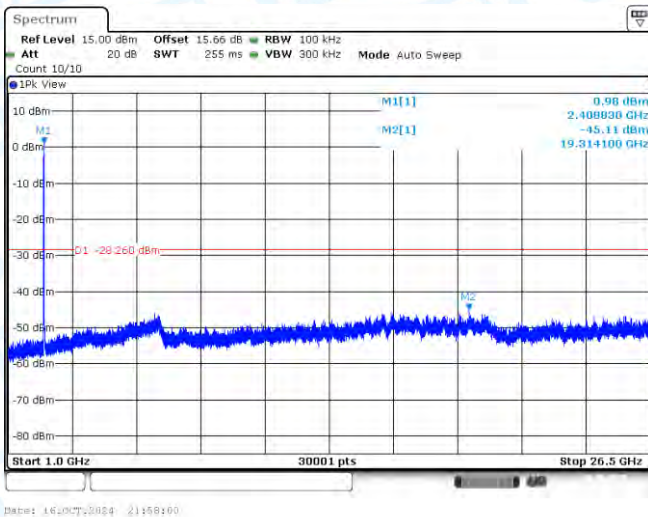
11AX20SISO-Ant1-2412-1000~26500-PASS
