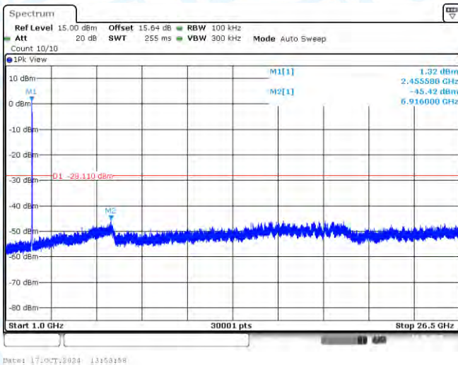
11AX20SISO-Ant1-2462-1000~26500-PASS
