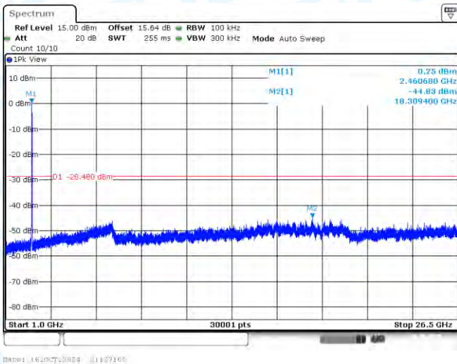
11N20SISO-Ant1-2462-1000~26500-PASS
