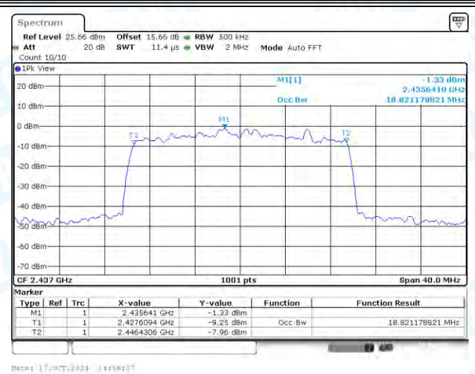
11AX20SISO-Ant1-2437
