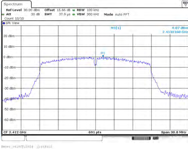
11N20SISO-Ant1-2412-0~Reference-PASS
