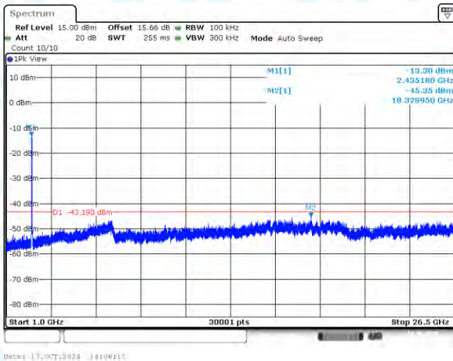
11AX40SISO-Ant1-2437-1000~26500-PASS
