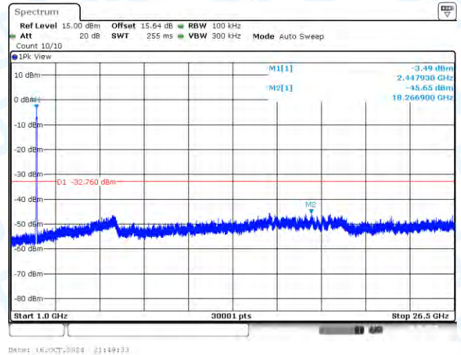
11N40SISO-Ant1-2452-1000~26500-PASS
