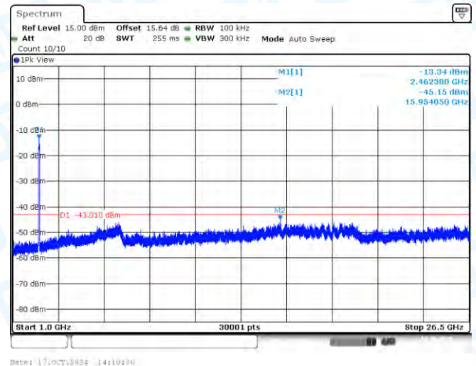
11AX40SISO-Ant1-2452-1000~26500-PASS
