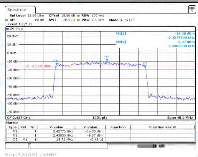
11AX20SISO-Ant1-2437-PASS
