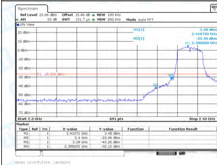
11G-Ant1-2412-PASS
