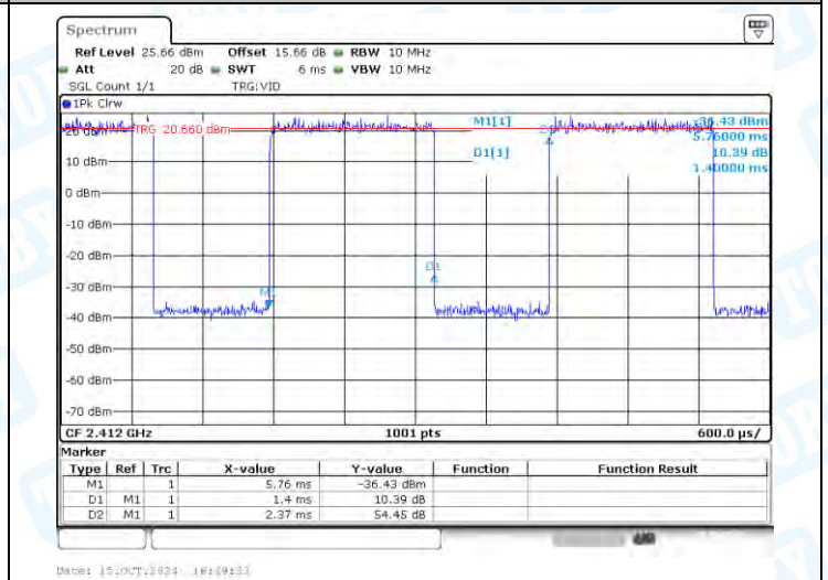
NTVN-11G-Ant1-2412
