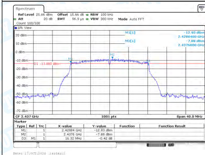
11G-Ant1-2437-PASS
