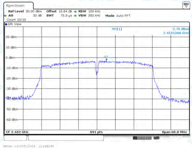
11N40SISO-Ant1-2452-0~Reference-PASS
