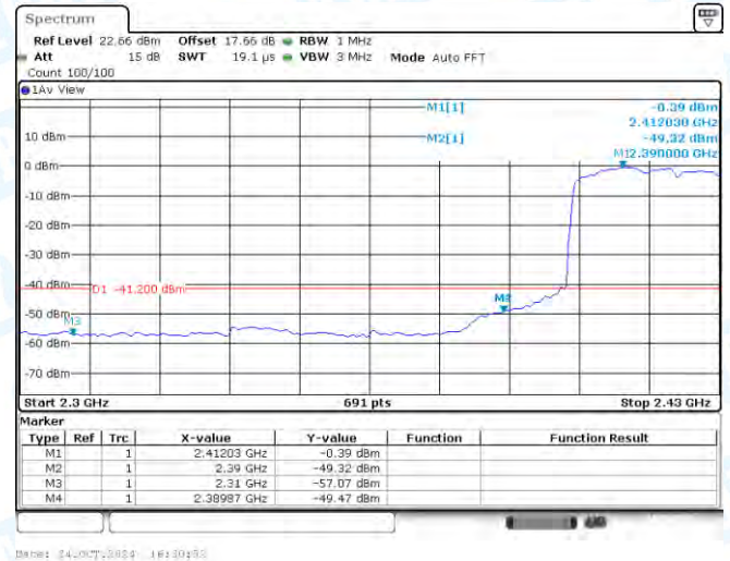
11AX40ISO-Ant1-2422-PASS
