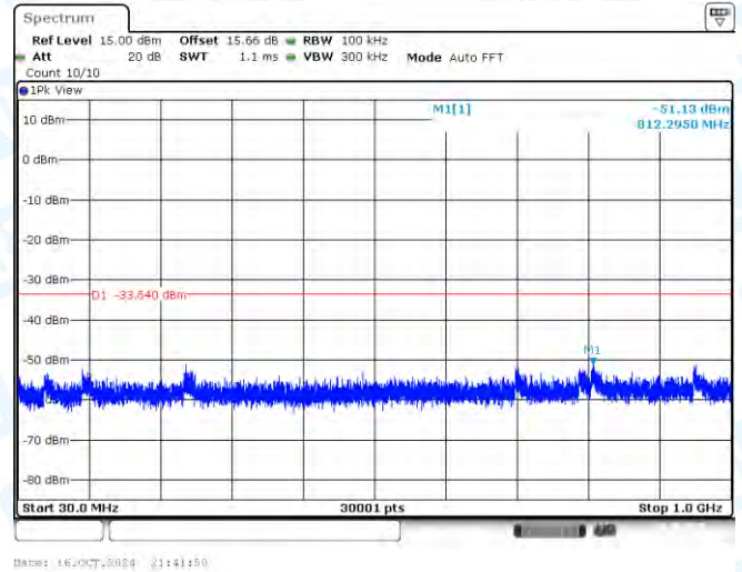
11N40SISO-Ant1-2437-30~1000-PASS
