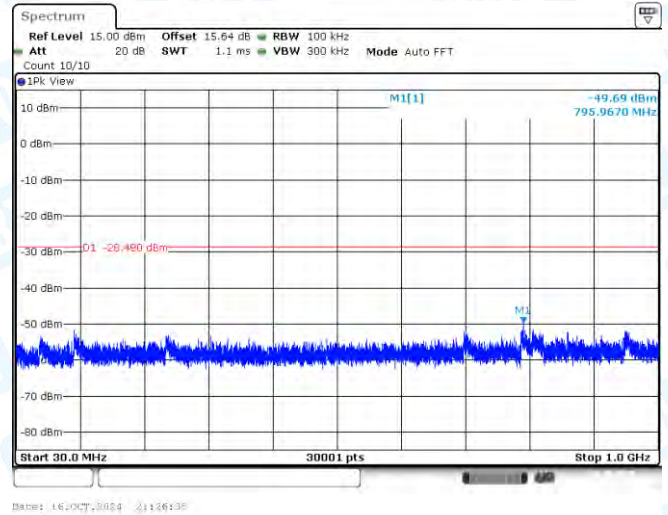
11N20SISO-Ant1-2462-30~1000-PASS
