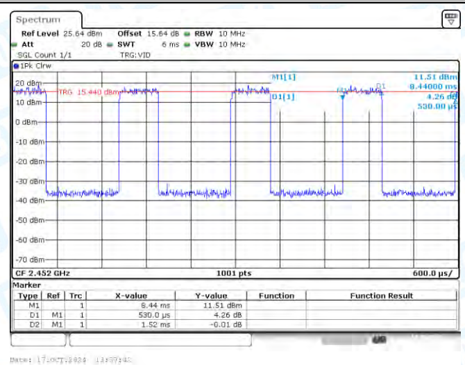
NTNV-11AX40SISO-Ant1-2452
