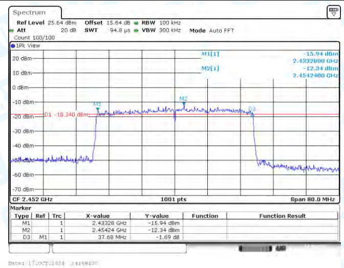
11AX40SISO-Ant1-2452-PASS
