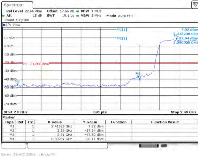
11N40SISO-Ant1-2422-PASS
