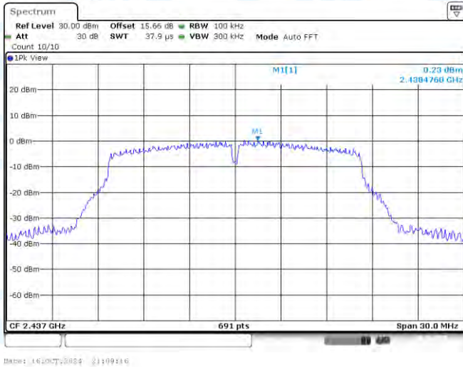
11G-Ant1-2437-0~Reference-PASS
