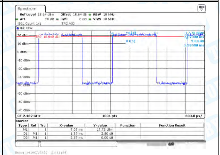
NTVN-11G-Ant1-2462
