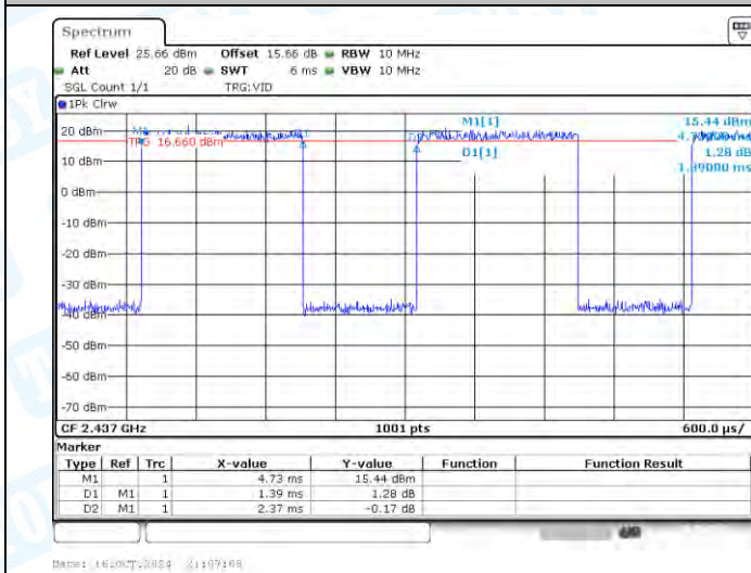
NTVN-11G-Ant1-2437
