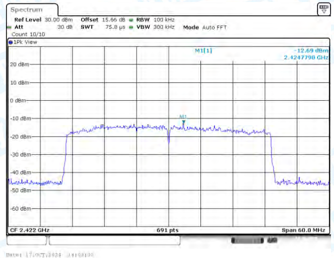
11AX40SISO-Ant1-2422-0~Reference-PASS
