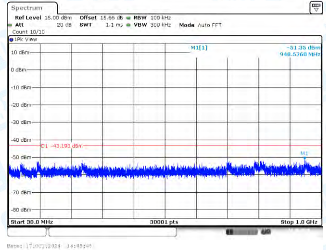
11AX40SISO-Ant1-2437-30~1000-PASS
