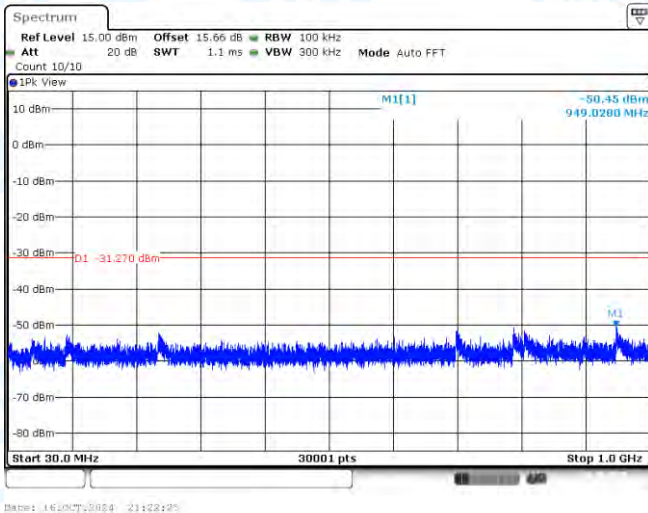
11N20SISO-Ant1-2437-30~1000-PASS
