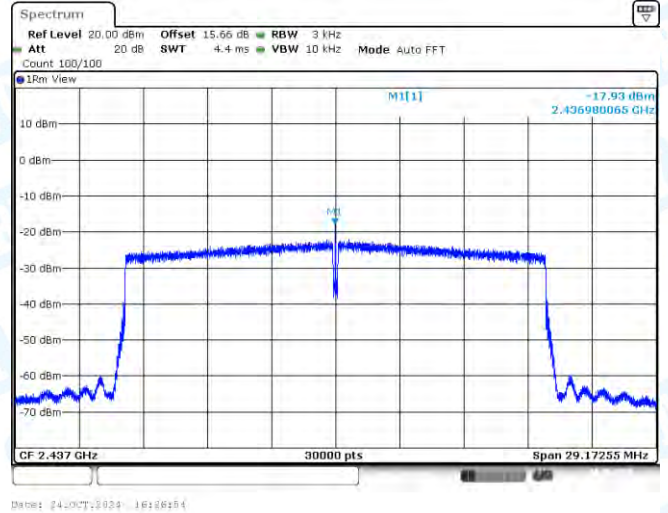
11AX20SISO-Ant1-2437-PASS
