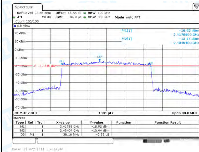
11AX40SISO-Ant1-2437-PASS
