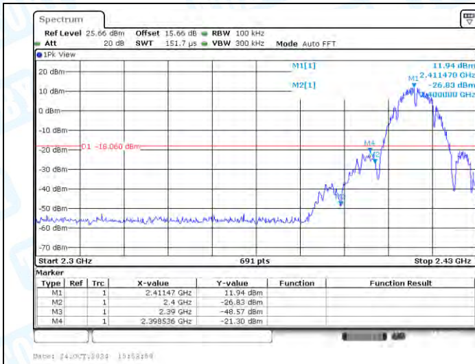
11B-Ant1-2412-PASS
