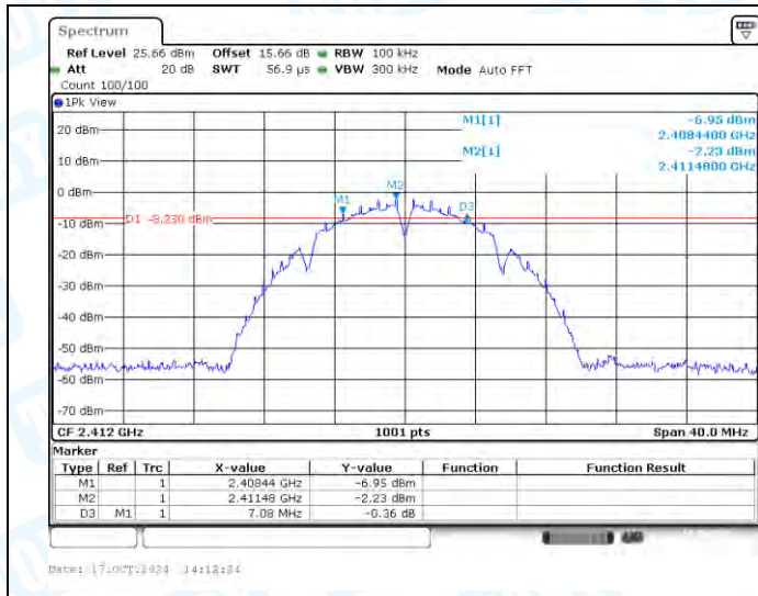
11B-Ant1-2412-PASS
