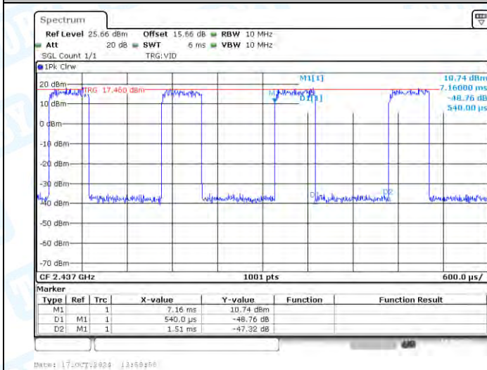
NTNV-11AX40SISO-Ant1-2437
