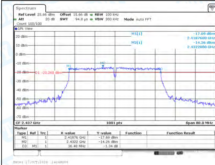
11N40SISO-Ant1-2437-PASS
