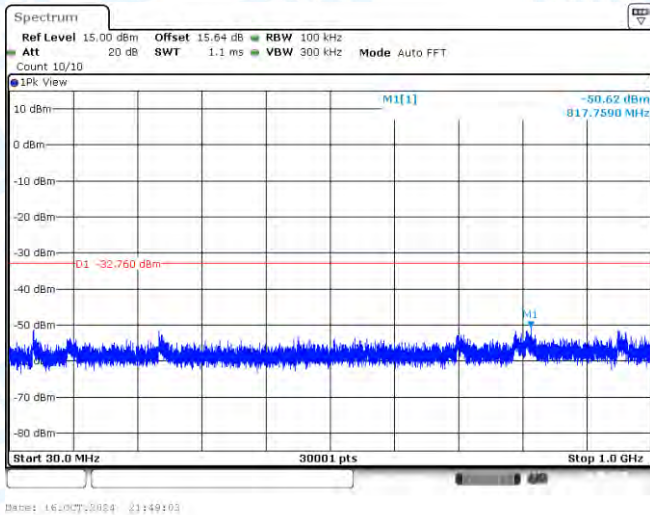
11N40SISO-Ant1-2452-30~1000-PASS
