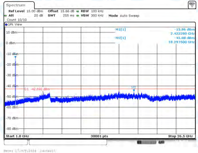
11AX40SISO-Ant1-2422-1000~26500-PASS
