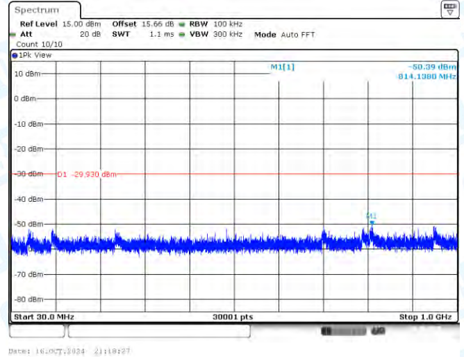
11N20SISO-Ant1-2412-30~1000-PASS
