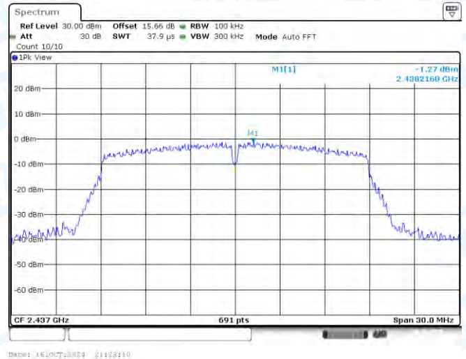
11N20SISO-Ant1-2437-0~Reference-PASS
