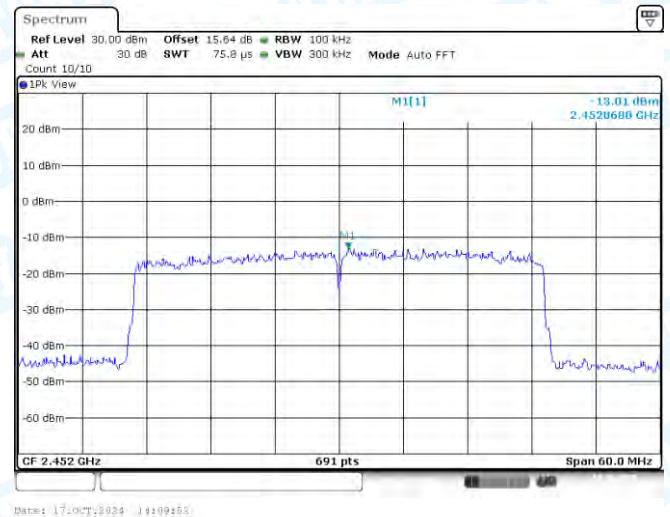
11AX40SISO-Ant1-2452-0~Reference-PASS
