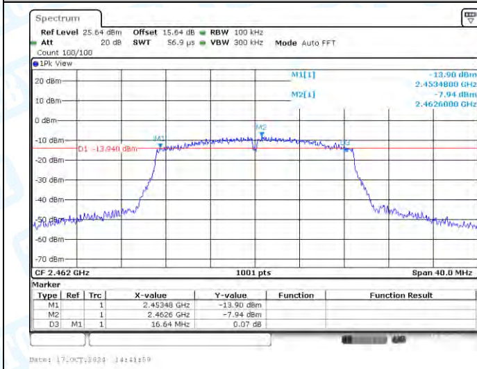
11N20SISO-Ant1-2462-PASS
