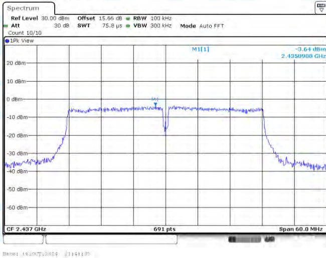
11N40SISO-Ant1-2437-0~Reference-PASS
