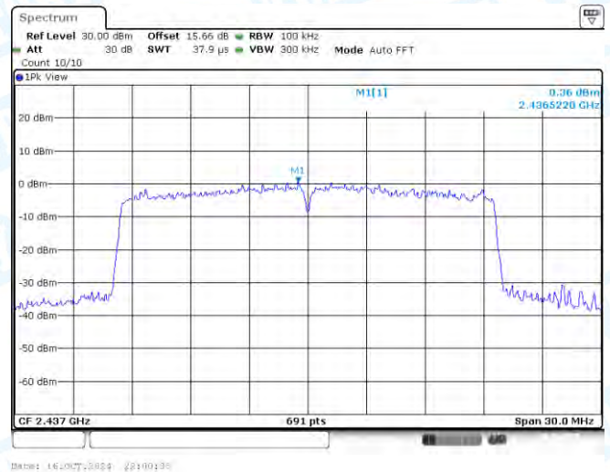
11AX20SISO-Ant1-2437-0~Reference-PASS
