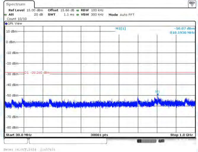
11AX20SISO-Ant1-2412-30~1000-PASS
