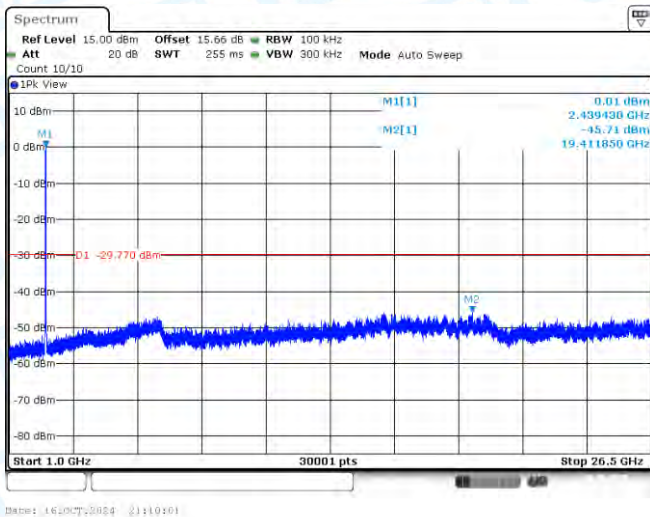
11G-Ant1-2437-1000~26500-PASS
