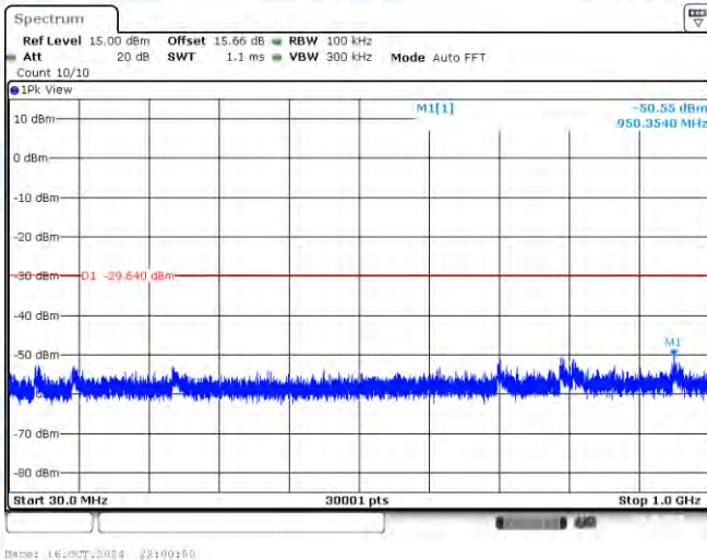
11AX20SISO-Ant1-2437-30~1000-PASS
