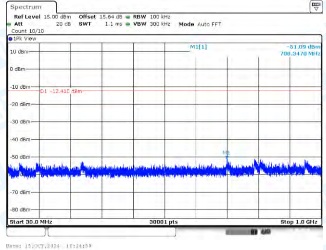
11B-Ant1-2462-30~1000-PASS
