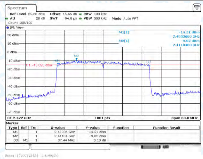
11AX40SISO-Ant1-2422-PASS
