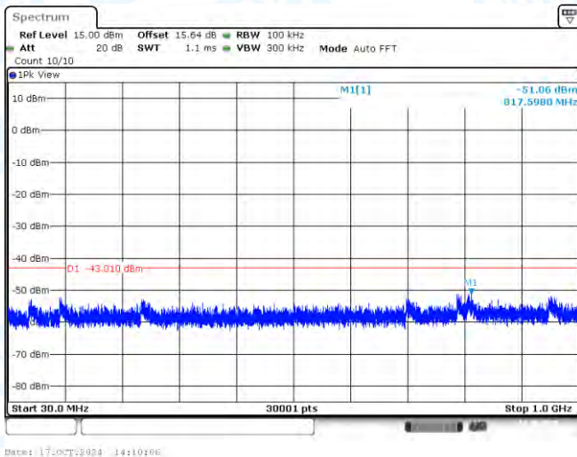
11AX40SISO-Ant1-2452-30~1000-PASS
