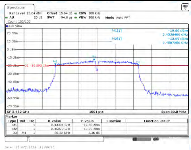
11N40SISO-Ant1-2452-PASS
