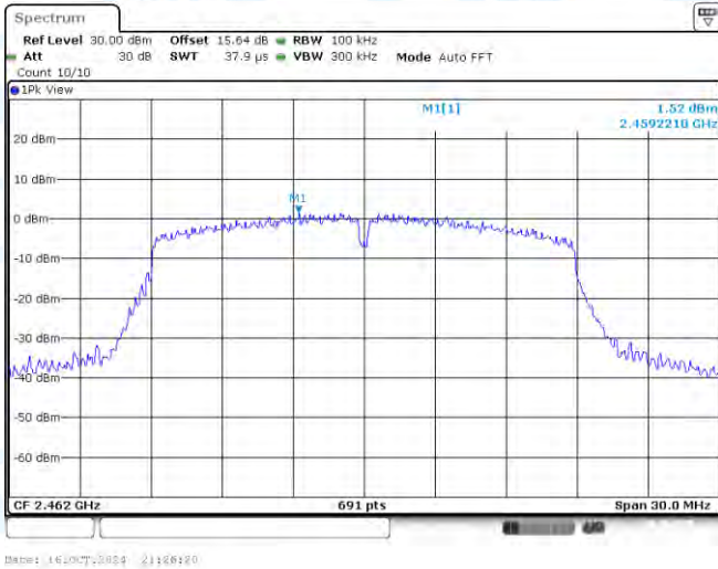
11N20SISO-Ant1-2462-0~Reference-PASS
