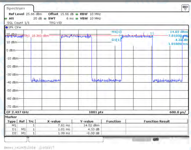
NTNV-11AX20SISO-Ant1-2437
