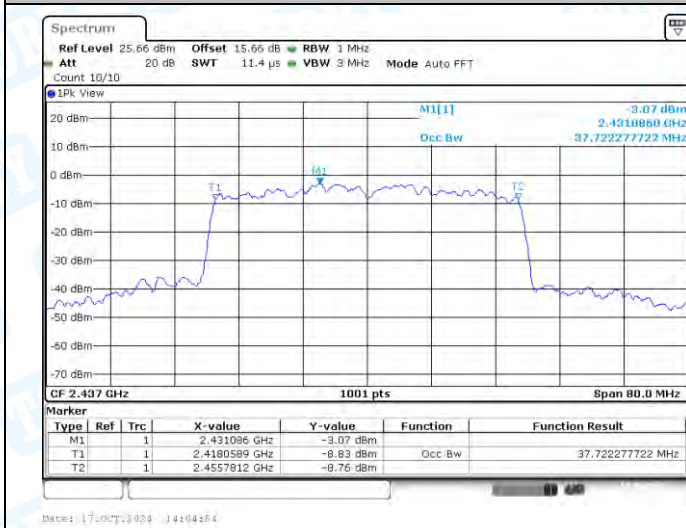
11AX40SISO-Ant1-2437
