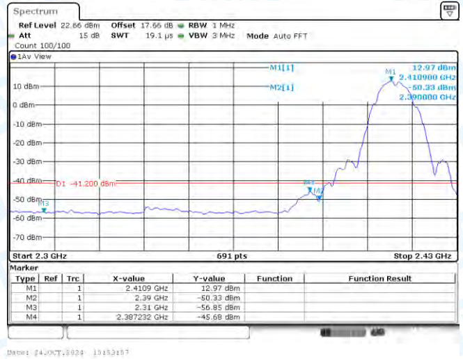
11B-Ant1-2412-PASS
