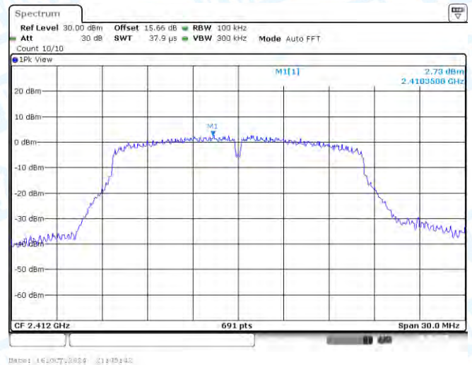
11G-Ant1-2412-0~Reference-PASS
