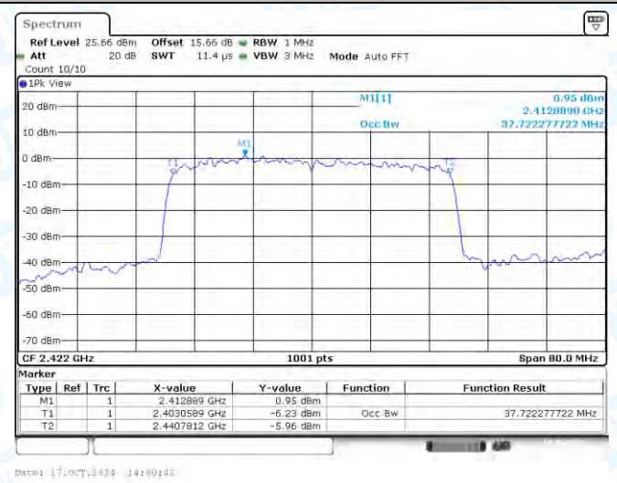
11AX40SISO-Ant1-2422
