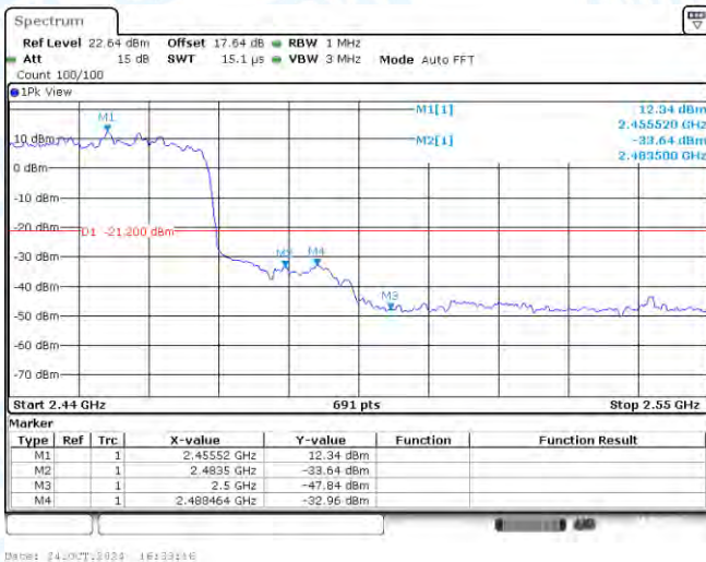
11AX40ISO-Ant1-2452-PASS
