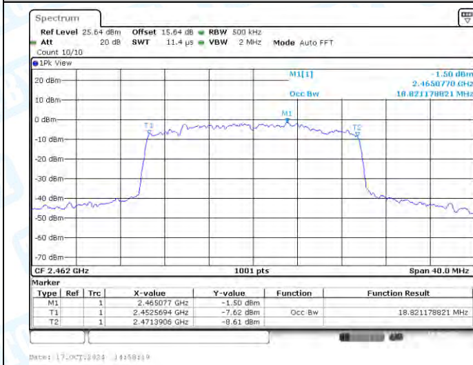
11AX20SISO-Ant1-2462
