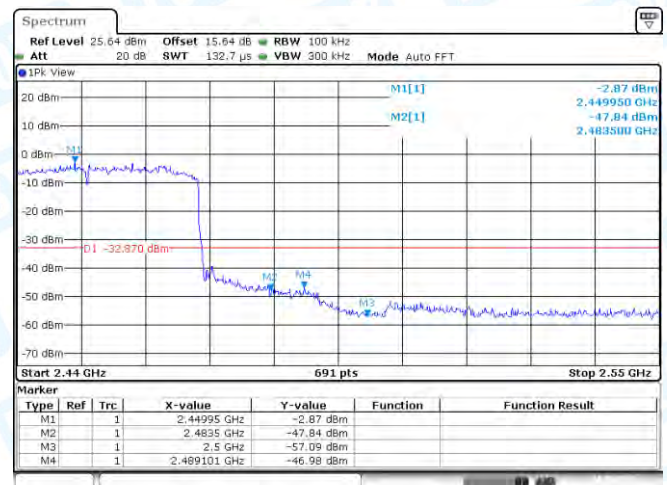
11AX20SISO-Ant1-2462-PASS
