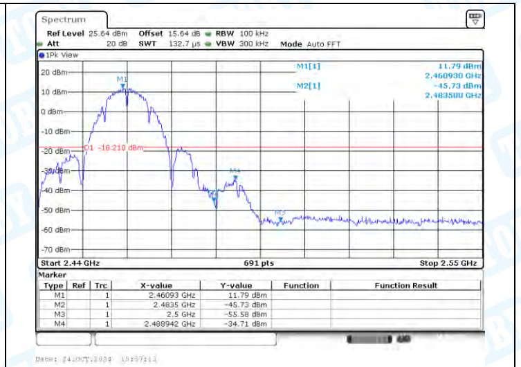
11B-Ant1-2462-PASS
