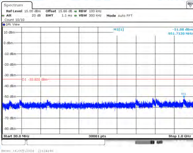
11N40SISO-Ant1-2422-30~1000-PASS
