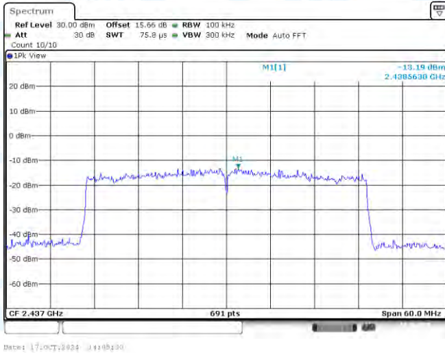
11AX40SISO-Ant1-2437-0~Reference-PASS
