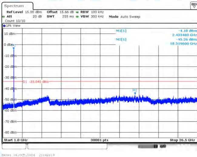
11N40SISO-Ant1-2437-1000~26500-PASS
