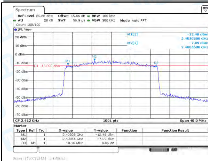
11AX20SISO-Ant1-2412-PASS
