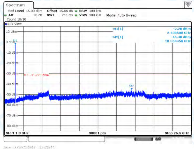
11N20SISO-Ant1-2437-1000~26500-PASS
