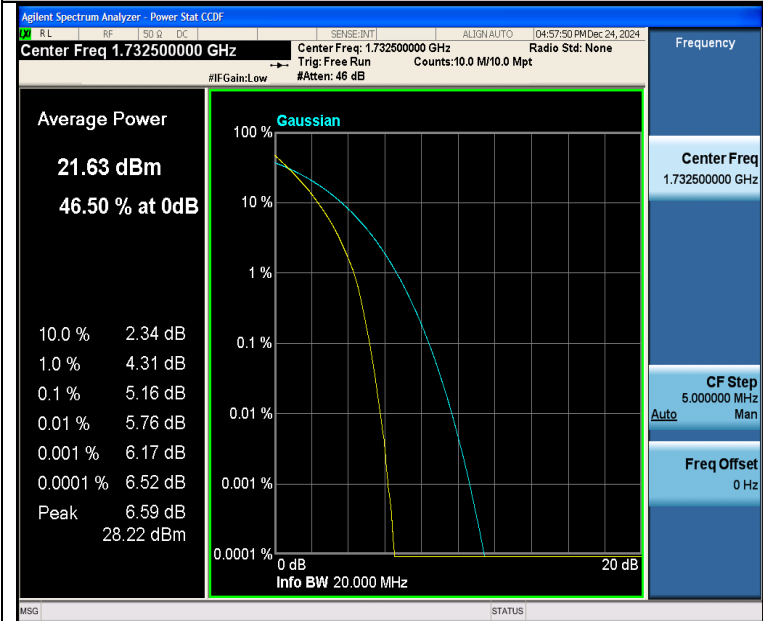
Band4-20MHz-QPSK-20175-100RB#0-PASS
