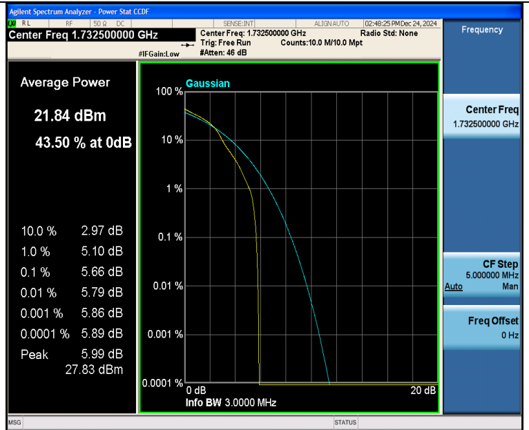
Band4-3MHz-16QAM-20175-1RB#0-PASS
