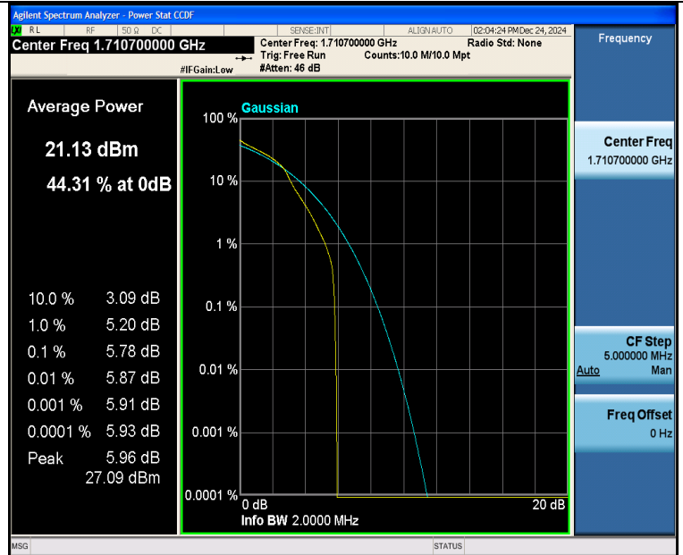
Band4-1.4MHz-16QAM-19957-1RB#0-PASS
