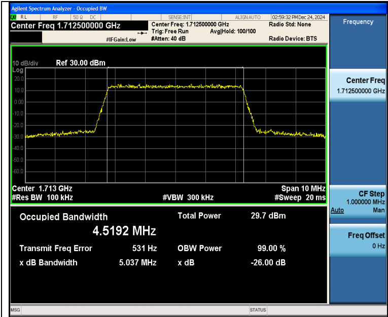
Band4-5MHz-QPSK-19975-25RB#0-PASS
