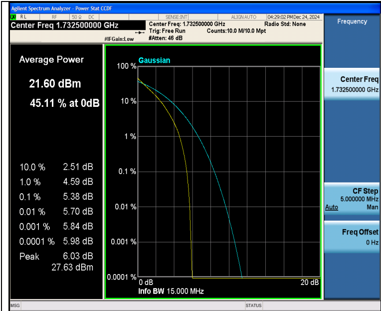
Band4-15MHz-QPSK-20175-75RB#0-PASS
