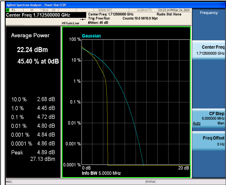
Band4-5MHz-QPSK-19975-1RB#0-PASS
