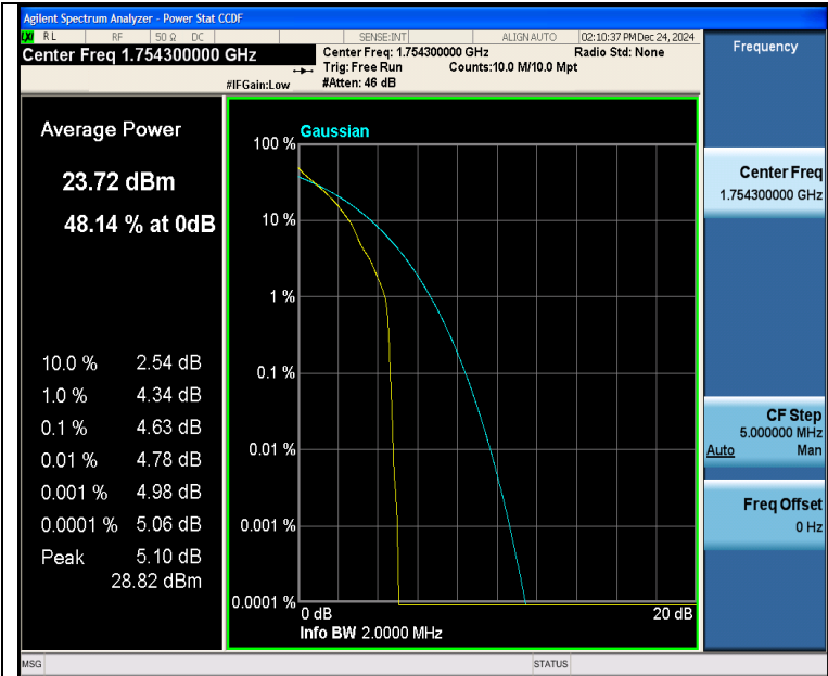
Band4-1.4MHz-QPSK-20393-1RB#0-PASS
