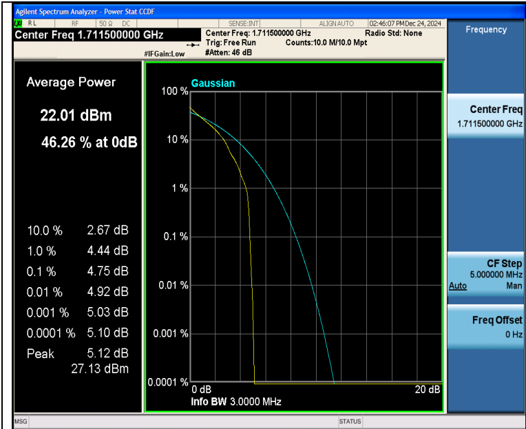
Band4-3MHz-QPSK-19965-1RB#0-PASS
