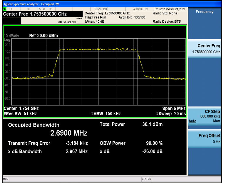
Band4-3MHz-16QAM-20385-15RB#0-PASS
