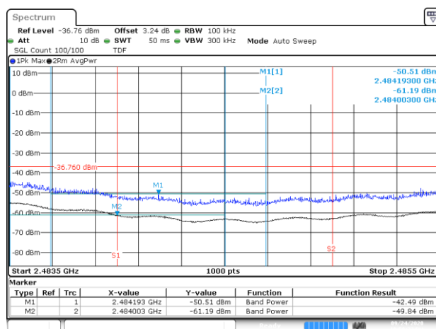
BE-R-HIGH-2MHz, MIMO-A, 802.11n40-HT0, Ch13
