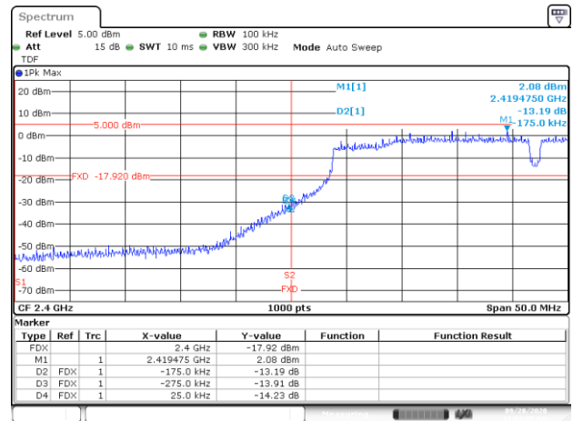
BE-NR, MIMO-B, 802.11n40- HT8, Ch1
