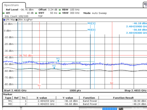
BE-R-HIGH-2MHz, MIMO-B, 802.11n40- HT8, Ch12
