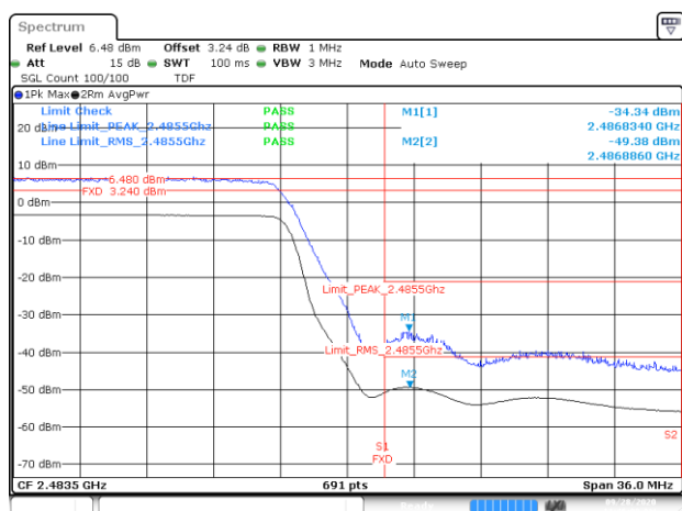
BE-R-HIGH, MIMO-B, 802.11n40- HT8, Ch13
