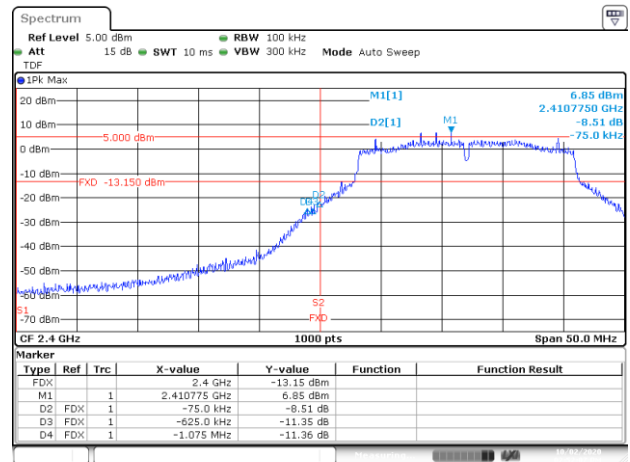
BE-NR, MIMO-A, 802.11n20-HT8, Ch1
