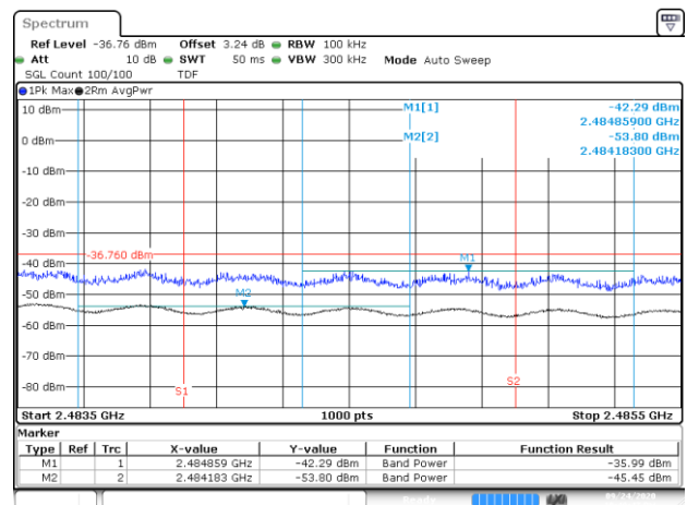
BE-R-HIGH-2MHz, MIMO-A, 802.11n20-HT8, Ch12
