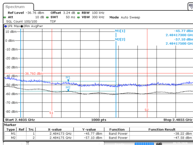
BE-R-HIGH-2MHz, SISO-B, 802.11n40-HT0, Ch13
