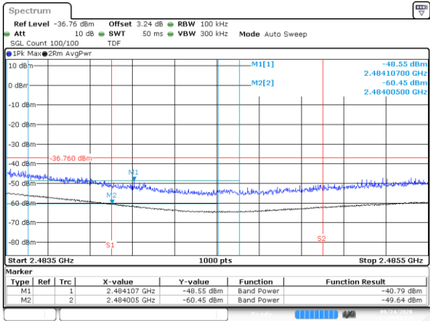
BE-R-HIGH-2MHz, MIMO-A, 802.11ax40-HE0, Ch13
