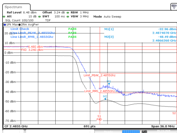
BE-R-HIGH, MIMO-A, 802.11n40-HT0, Ch13
