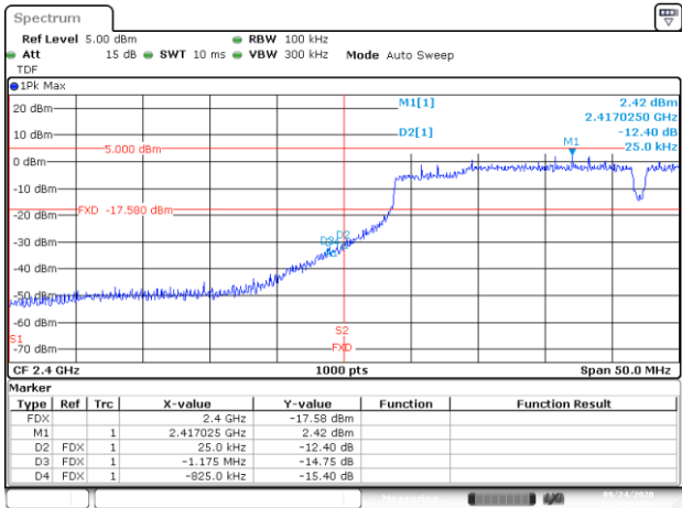
BE-NR, MIMO-A, 802.11n40- HT8, Ch1
