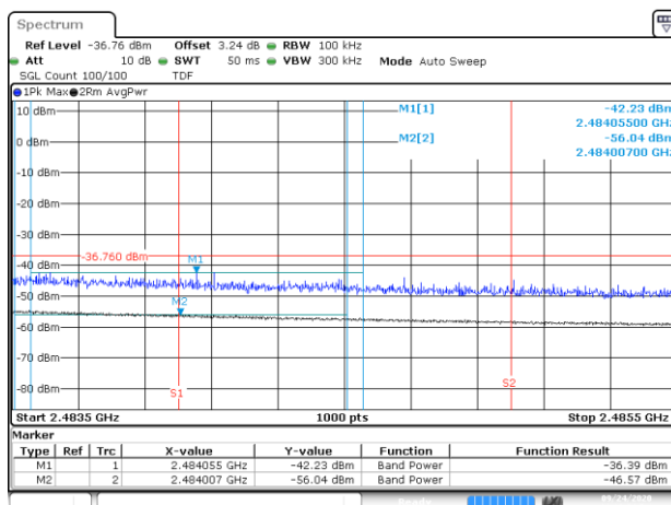
BE-R-HIGH-2MHz, MIMO-A, 802.11ax40-HE0, Ch12
