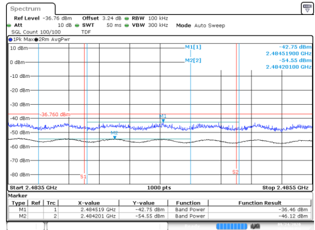
BE-R-HIGH-2MHz, MIMO-A, 802.11n20-HT8, Ch11
