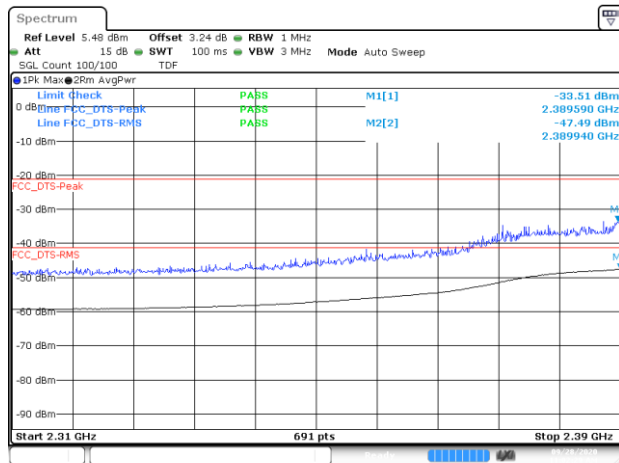
BE-R-LOW, MIMO-B, 802.11n40- HT8, Ch1
