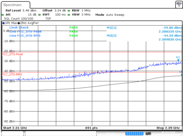
BE-R-LOW, MIMO-A, 802.11n40- HT8, Ch1
