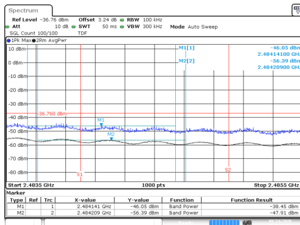
BE-R-HIGH-2MHz, MIMO-A, 802.11n40- HT8, Ch12
