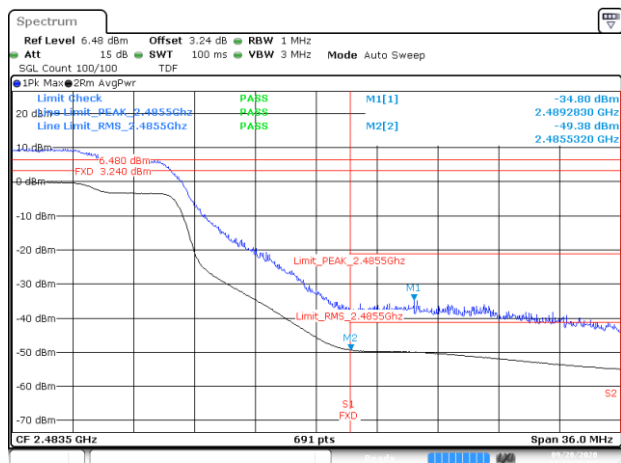
BE-R-HIGH, MIMO-B, 802.11n40- HT8, Ch12
