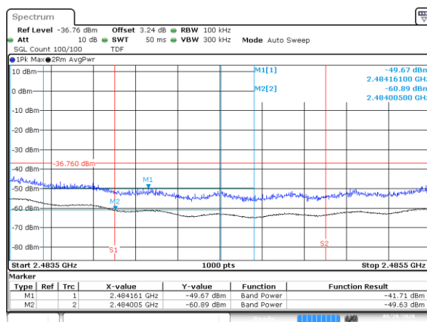
BE-R-HIGH-2MHz, MIMO-B, 802.11n40- HT8, Ch13
