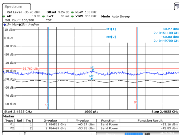
BE-R-HIGH-2MHz, SISO-B, 802.11n40-HT0, Ch12
