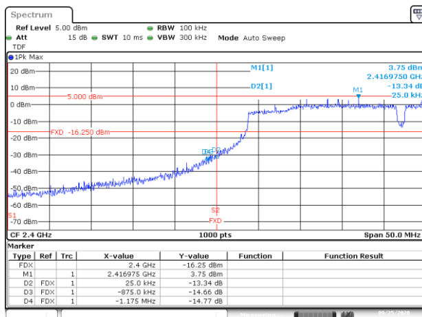
BE-NR, SISO-B, 802.11n40-HT0, Ch1
