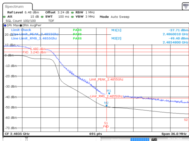
BE-R-HIGH, MIMO-A, 802.11n40- HT8, Ch12
