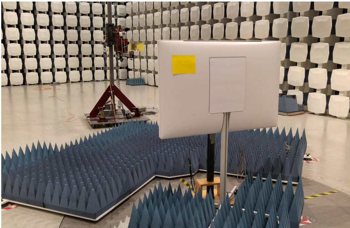
Radiated Emissions, 1 GHz – 8.5 GHz
