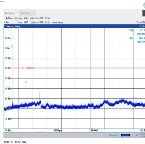
2DH5-Ant1-2441-1000~26500-0.62
