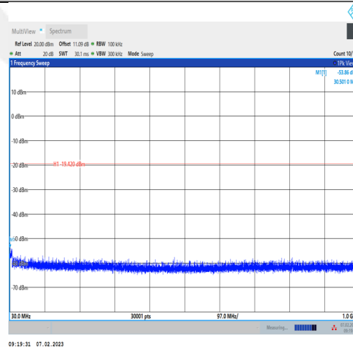
3DH5-Ant1-2441-30~1000-0.58
