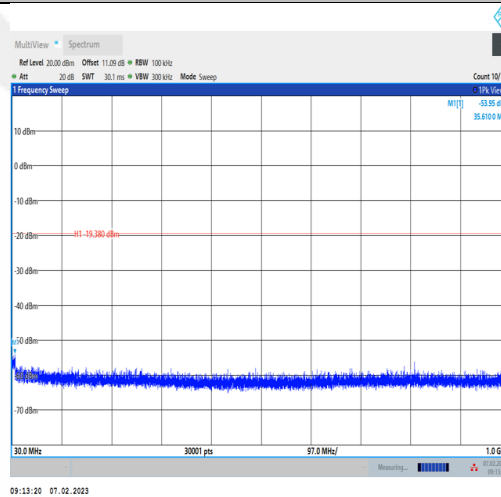
2DH5-Ant1-2441-30~1000-0.62
