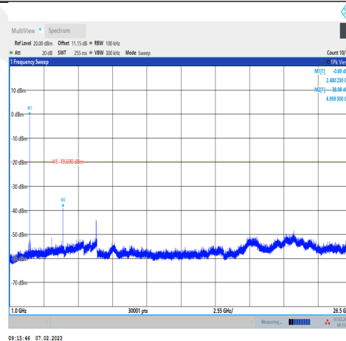
2DH5-Ant1-2480-1000~26500-0.31
