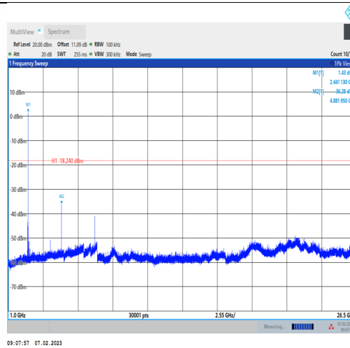
DH5-Ant1-2441-1000~26500-1.76
