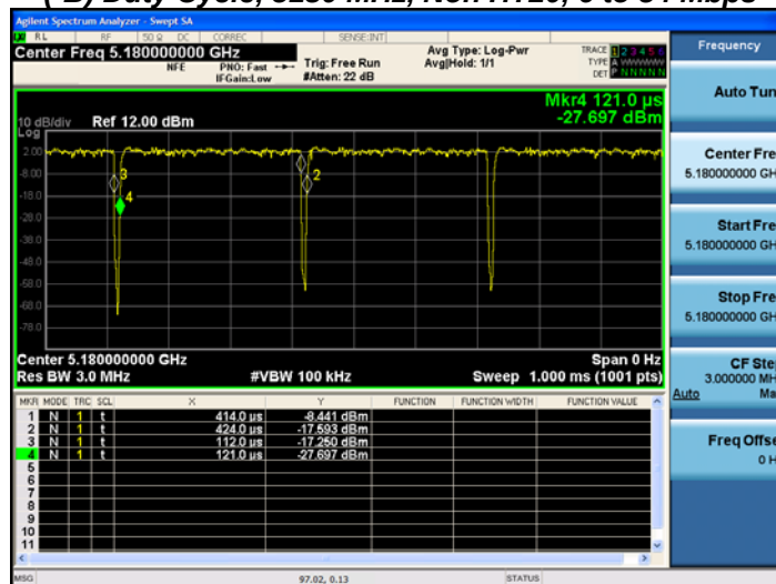
(-B) Duty Cycle, 5180 MHz, Non HT20, 6 to 54 Mbps
