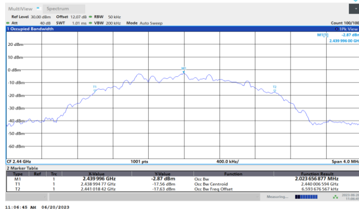
BLE_2M_Ant1_2440
