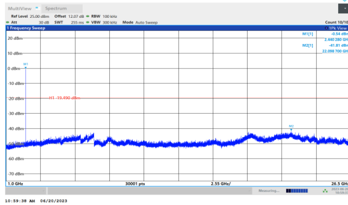
BLE_1M_Ant1_2440_1000~26500
