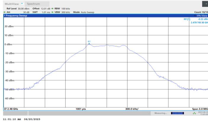
BLE_1M_Ant1_2480_0~Reference
