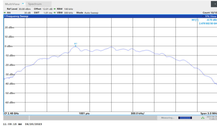
BLE_2M_Ant1_2480_0~Reference
