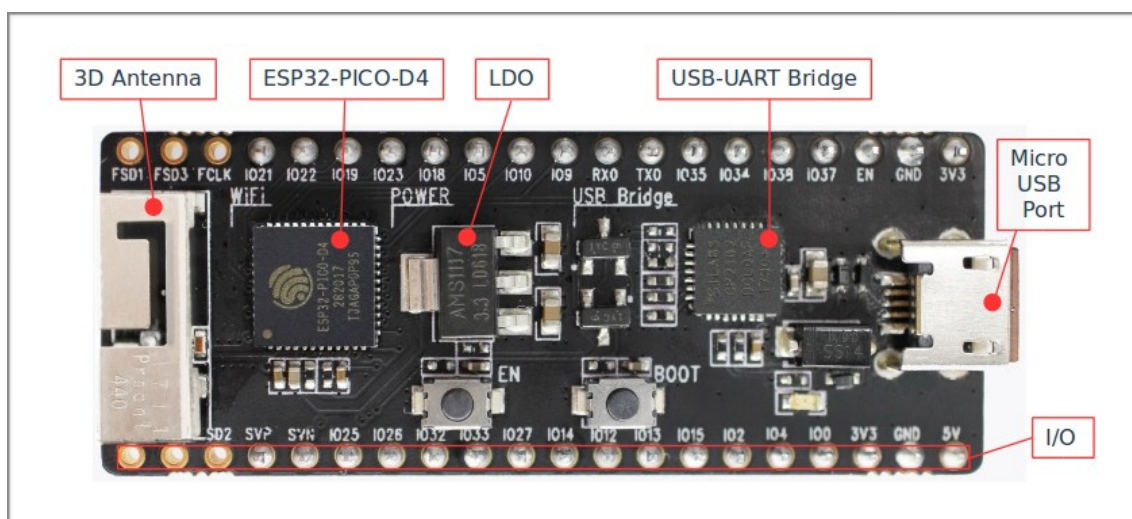
Figure 1-2. ESP32-PICO-KIT Board Layout
