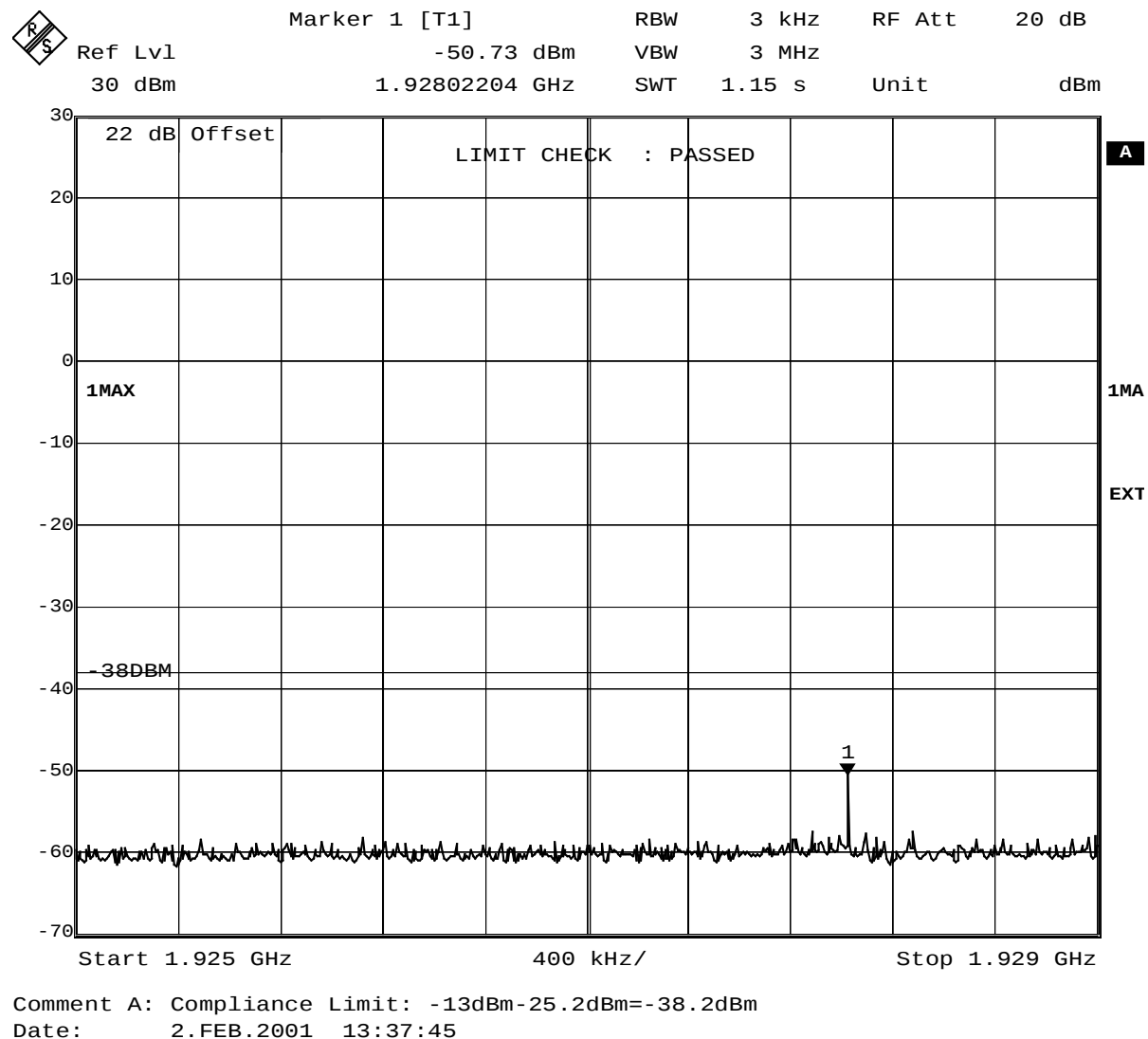
Fig. 17 – Spurious emissions in the frequency range 1925 MHz – 1929 MHz. Limit: -13dBm-25.2dB=-38.2dBm
