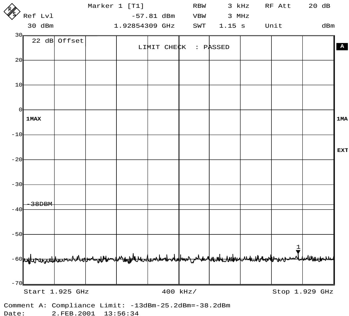
Fig. 24 – Spurious emissions in the frequency range 1925 MHz – 1929 MHz. Limit: -13dBm-25.2dB=-38.2dBm
