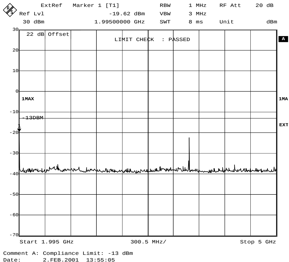
Fig. 28 – Spurious emissions in the frequency range 1995 MHz – 5000 MHz.
