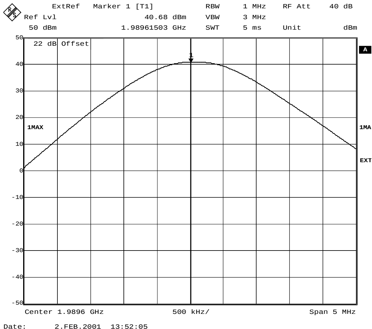
Fig. 5 – RF power at the antenna connector.
