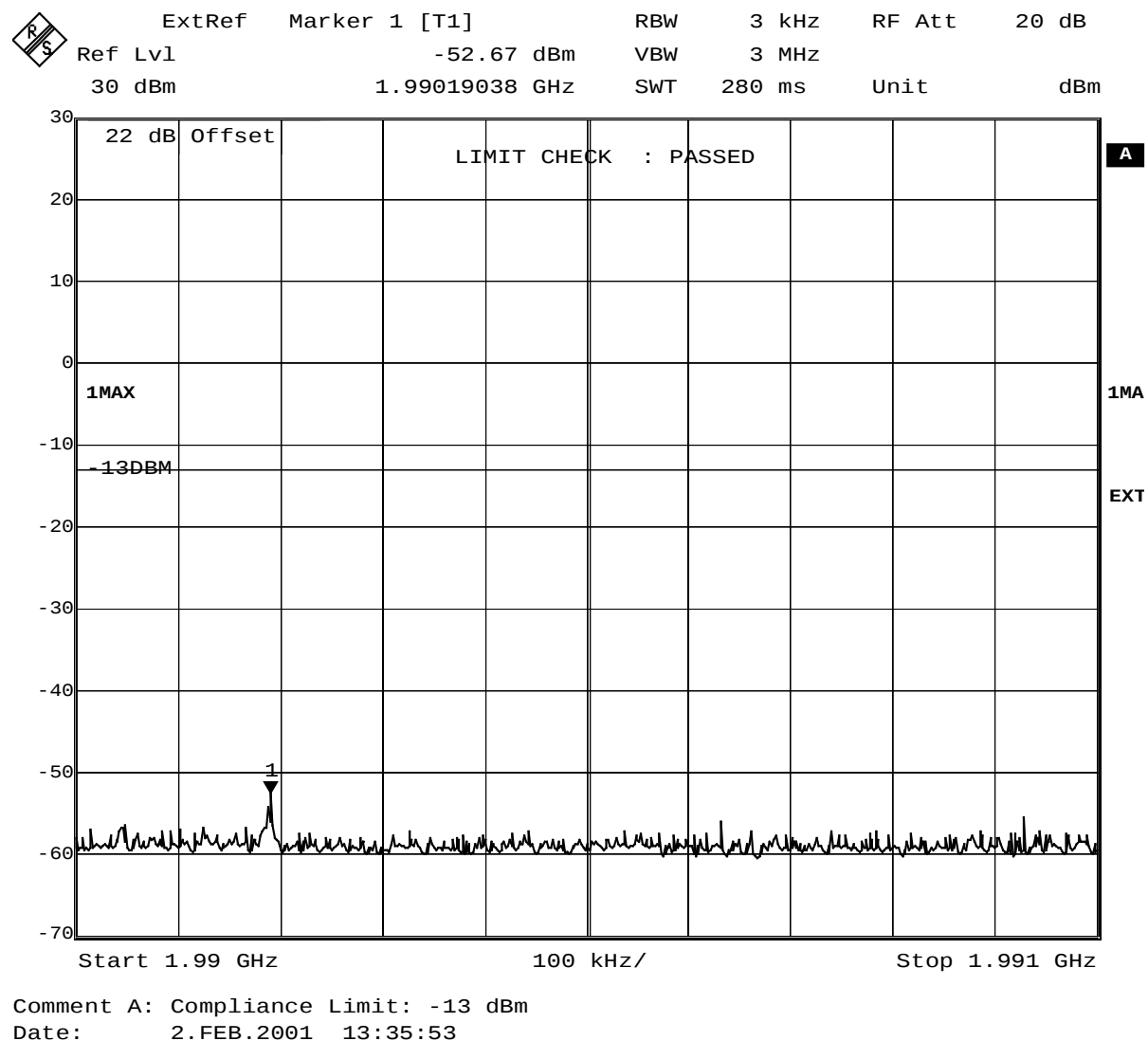
Fig. 19 – Spurious emissions in the frequency range 1990 MHz – 1991 MHz.
