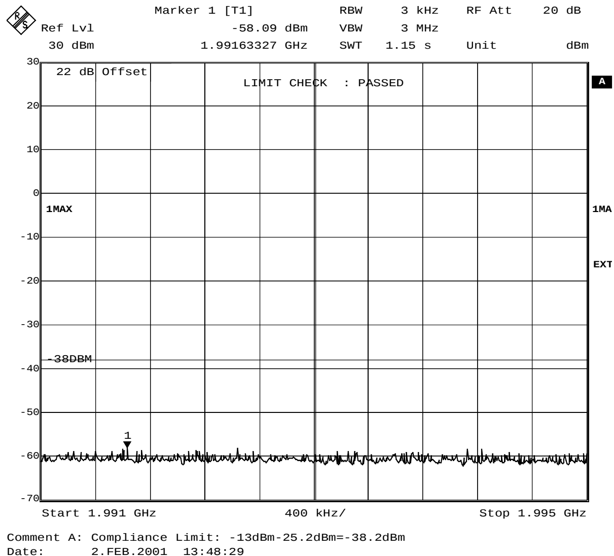
Fig. 13 – Spurious emissions in the frequency range 1991 MHz – 1995 MHz. Limit: -13dBm-25.2dB=-38.2dBm
