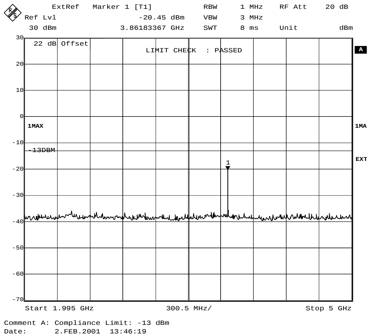
Fig. 14 – Spurious emissions in the frequency range 1995 MHz – 5000 MHz.
