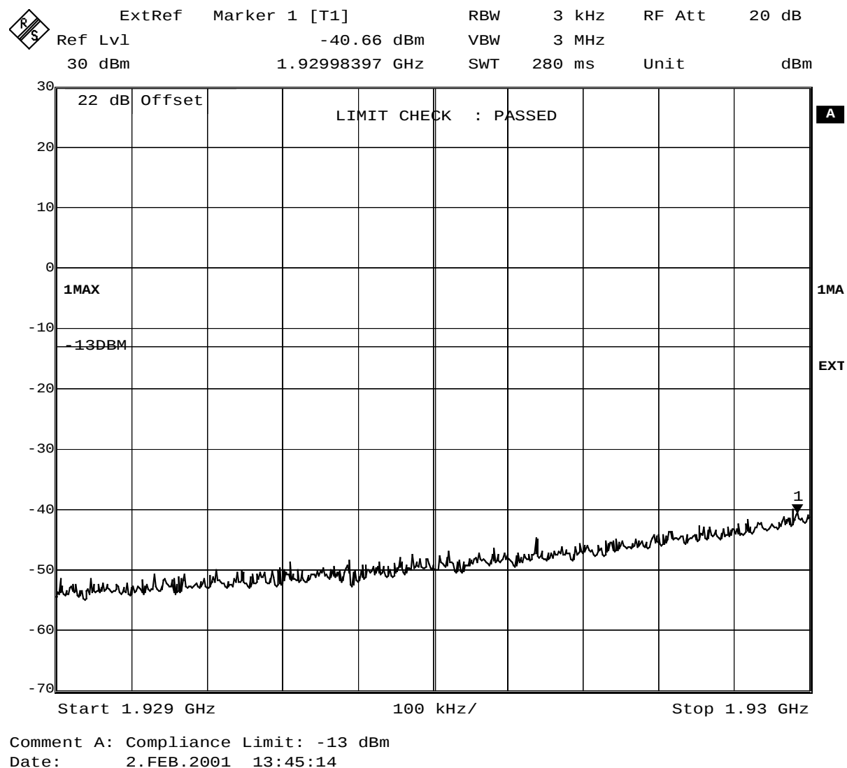
Fig. 11 – Spurious emissions in the frequency range 1929 MHz – 1930 MHz.
