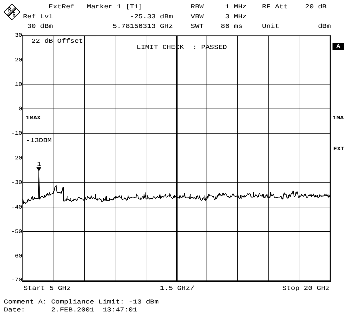
Fig. 15 – Spurious emissions in the frequency range 5000 MHz – 20000 MHz.
