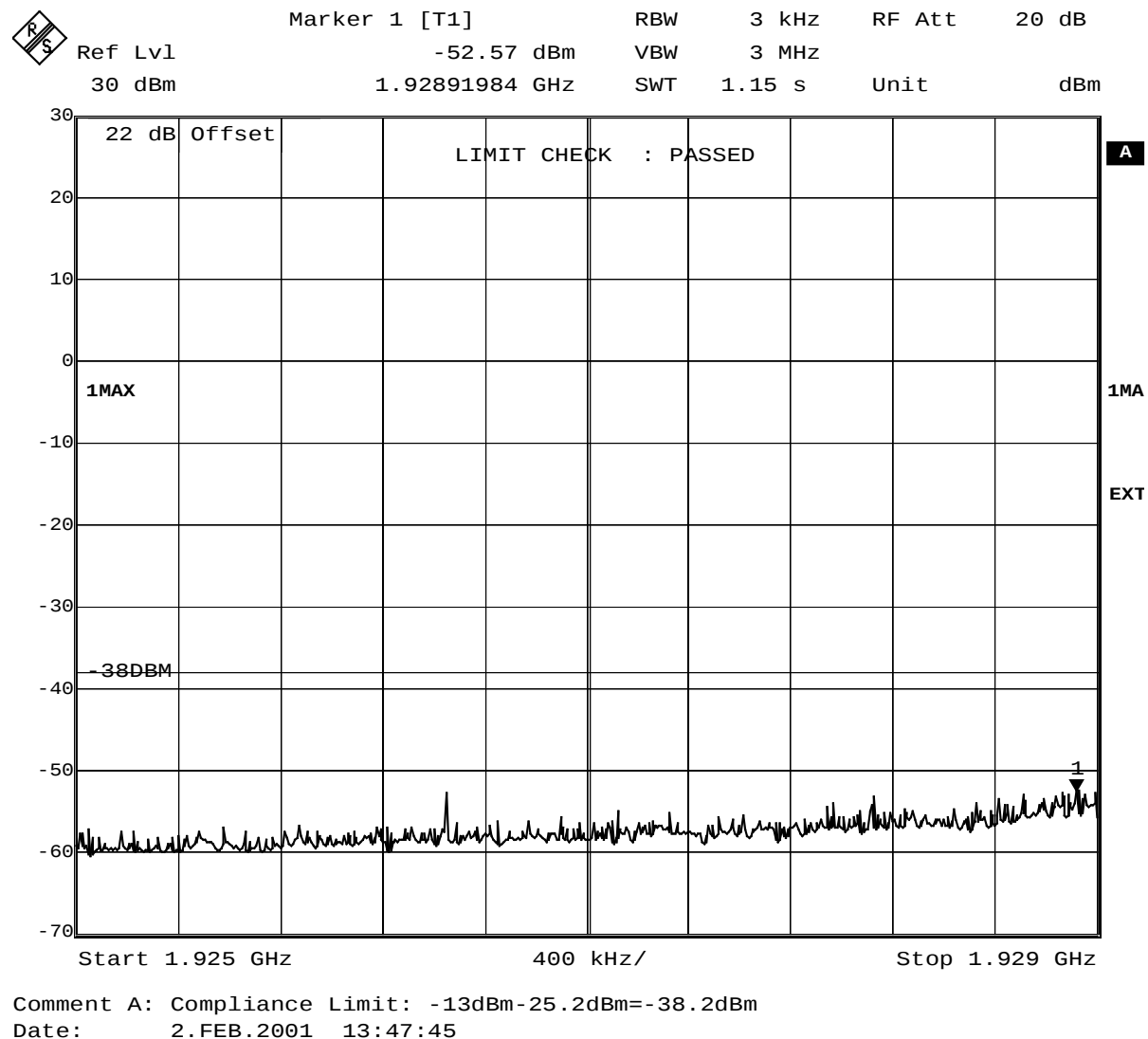
Fig. 10 – Spurious emissions in the frequency range 1925 MHz – 1929 MHz. Limit: -13\text{dBm} - 25.2\text{dB} = -38.2\text{dBm}
