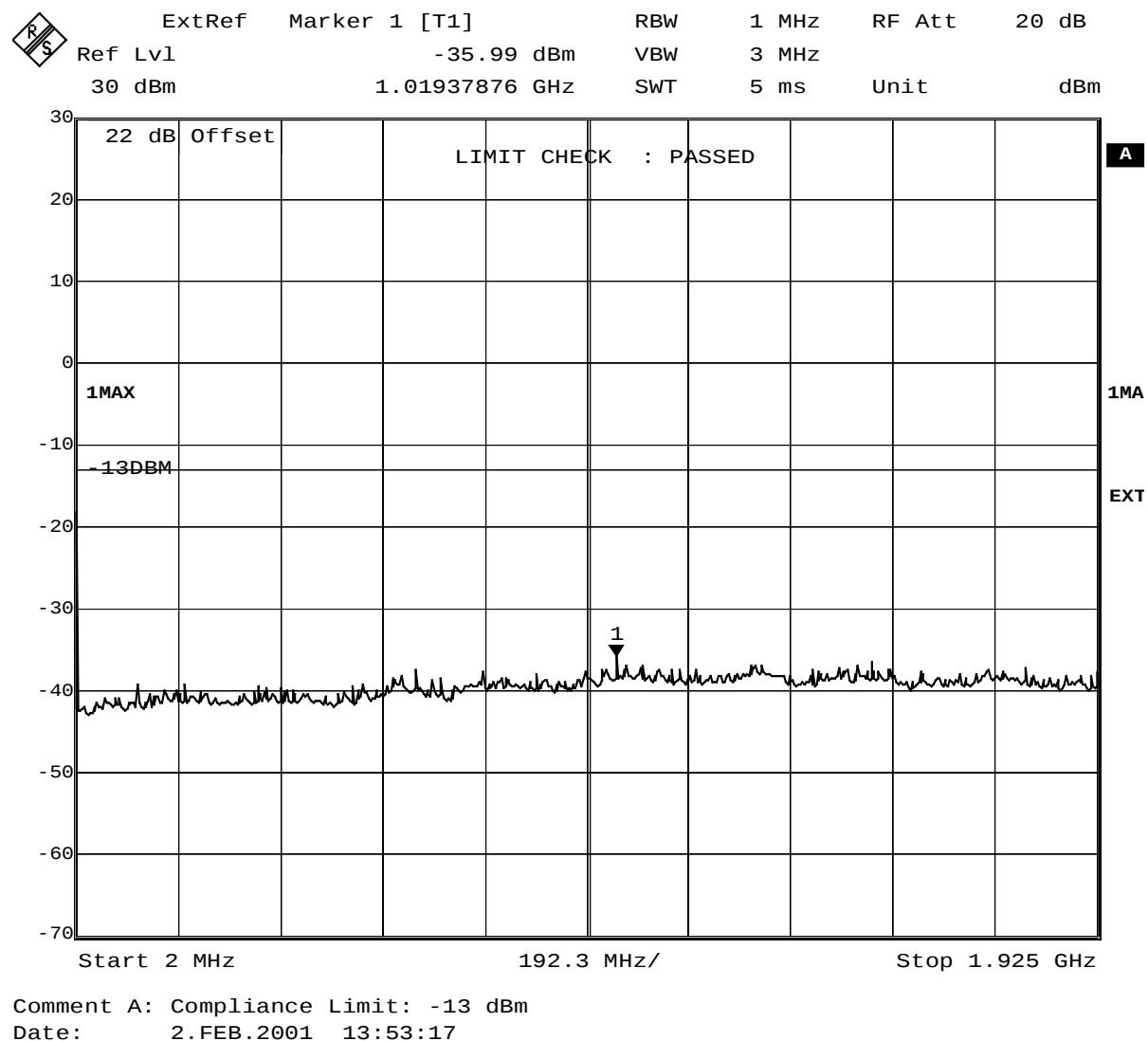
Fig. 23 – Spurious emissions in the frequency range 2 MHz – 1925 MHz.
