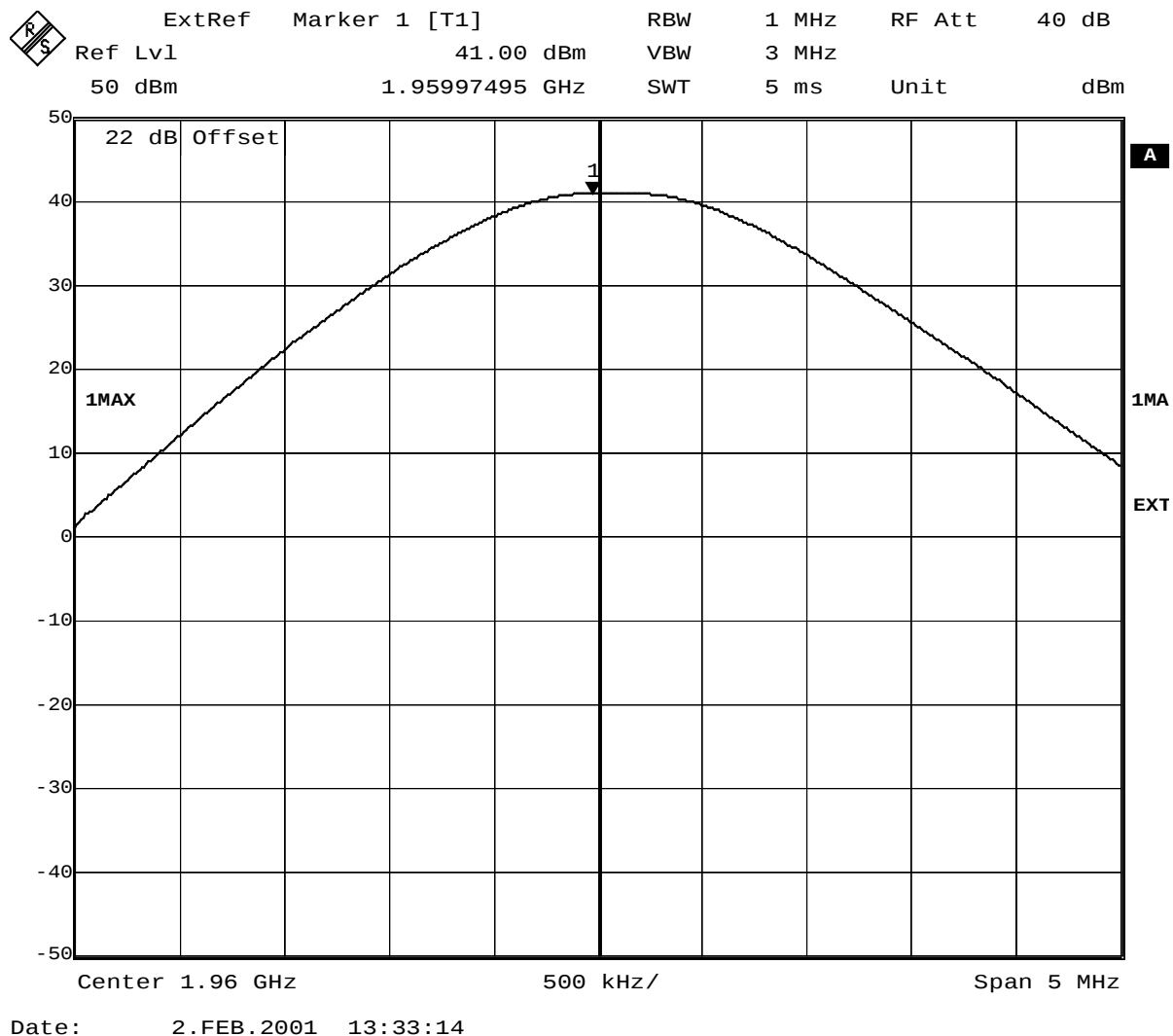
Fig. 4 – RF power at the antenna connector.
