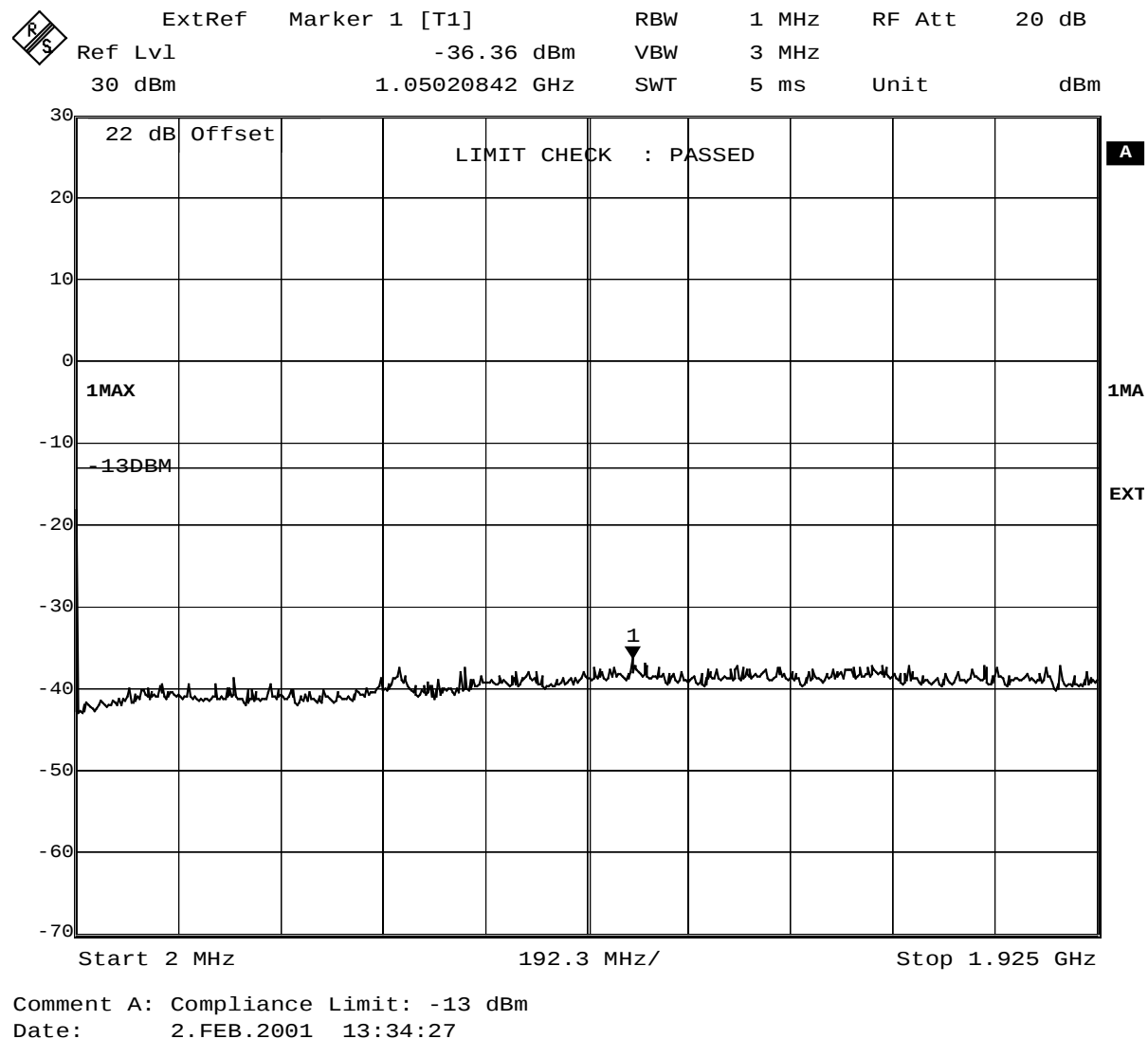
Fig. 16 – Spurious emissions in the frequency range 2 MHz – 1925 MHz.
