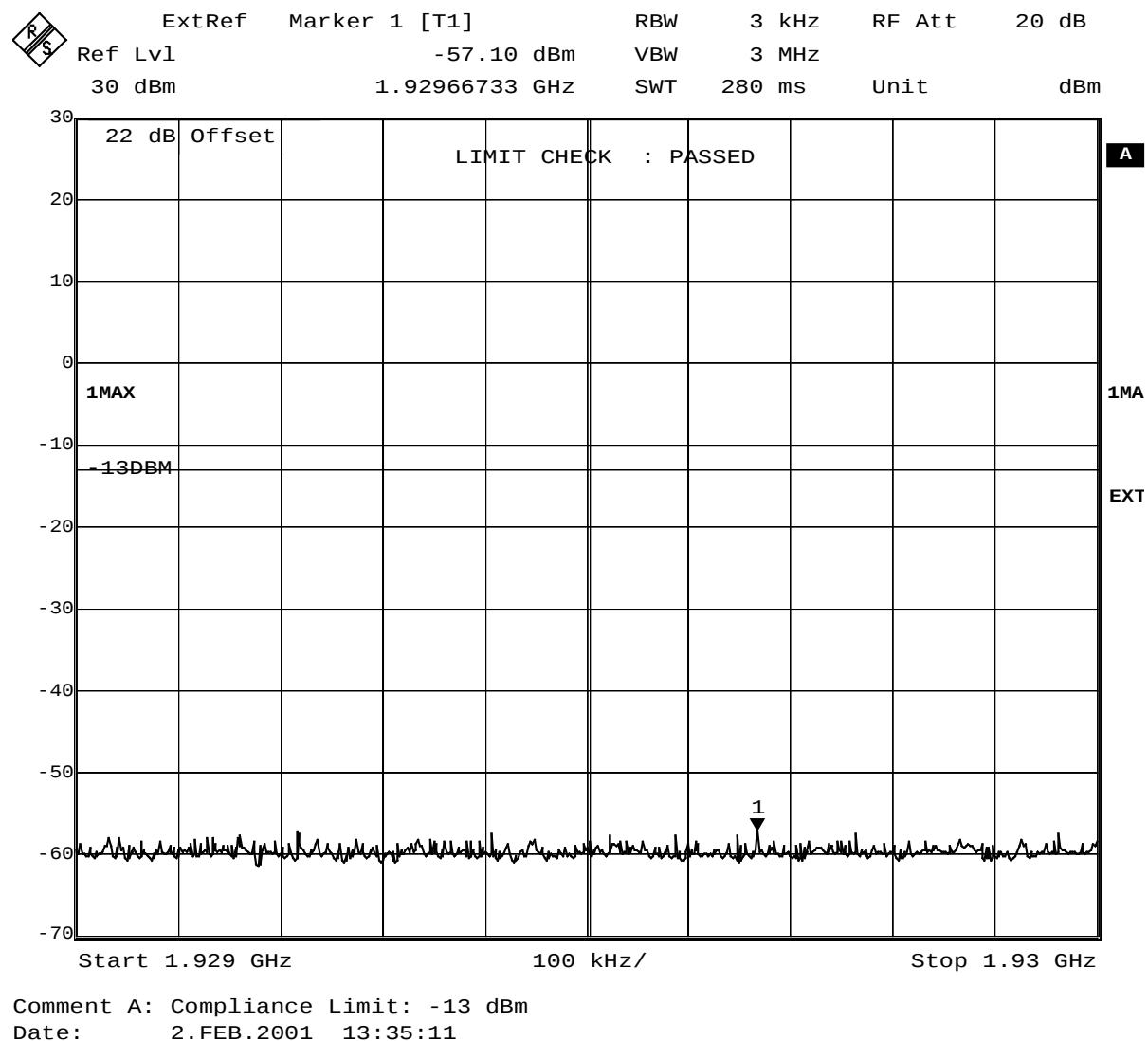
Fig. 18 – Spurious emissions in the frequency range 1929 MHz – 1930 MHz.
