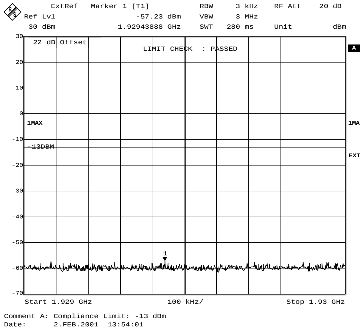
Fig. 25 – Spurious emissions in the frequency range 1929 MHz – 1930 MHz.
