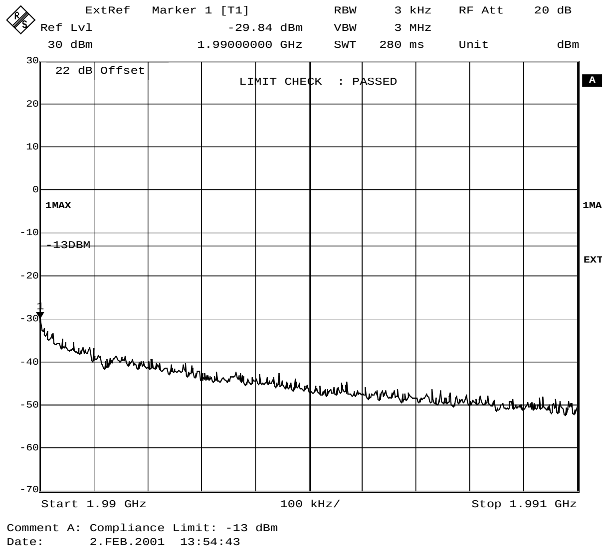
Fig. 26 – Spurious emissions in the frequency range 1990 MHz – 1991 MHz.
