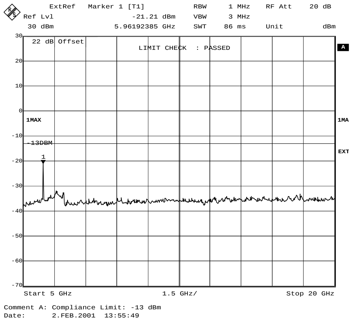
Fig. 29 – Spurious emissions in the frequency range 5000 MHz – 20000 MHz.
