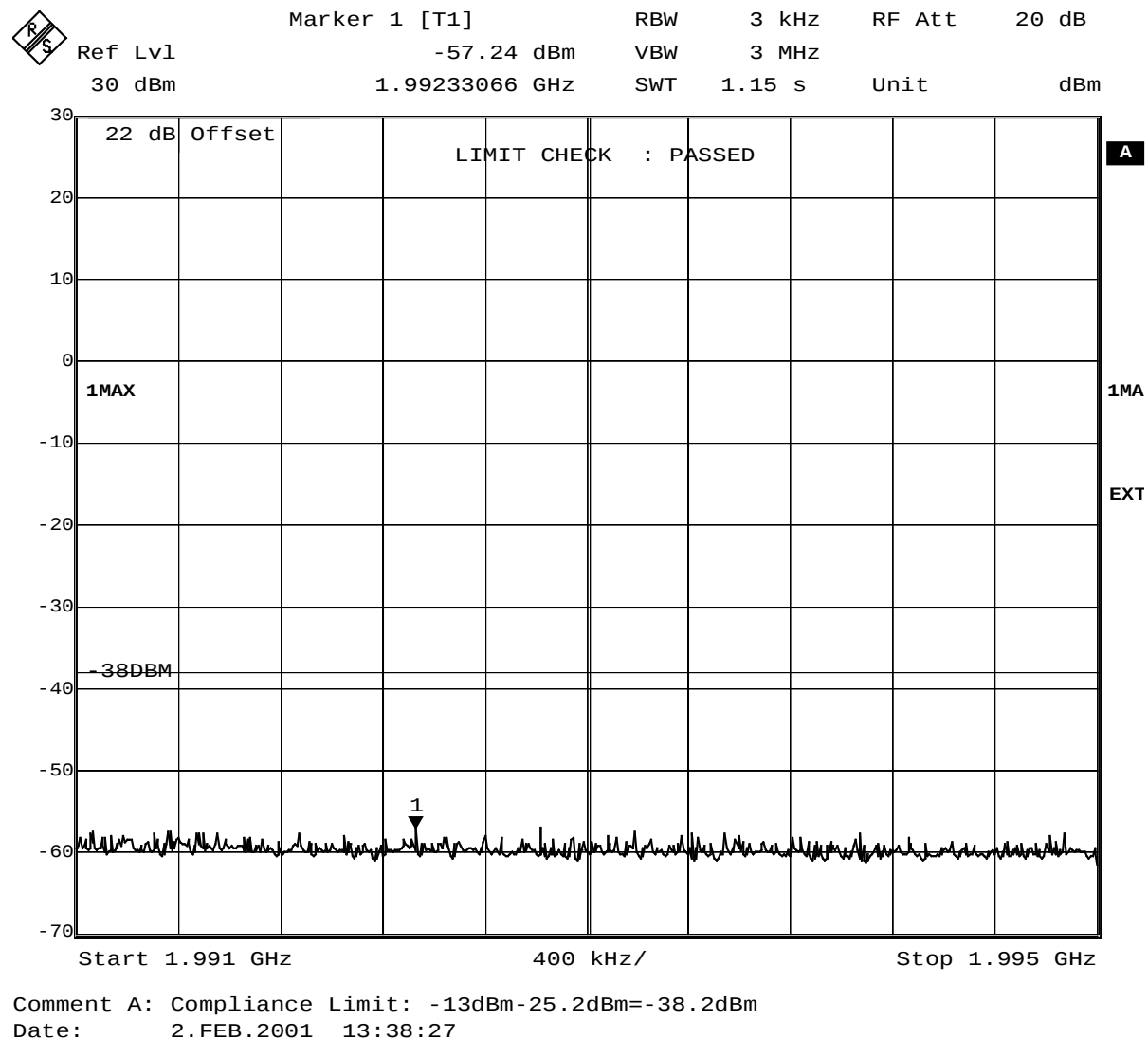
Fig. 20 – Spurious emissions in the frequency range 1991 MHz – 1995 MHz. Limit: -13dBm-25.2dB=-38.2dBm
