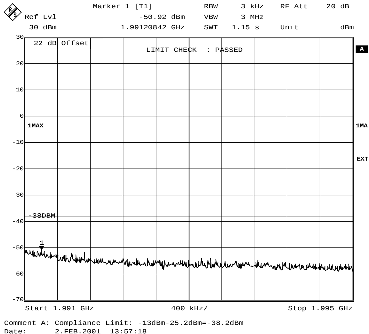
Fig. 27 – Spurious emissions in the frequency range 1991 MHz – 1995 MHz. Limit: -13dBm-25.2dB=-38.2dBm
