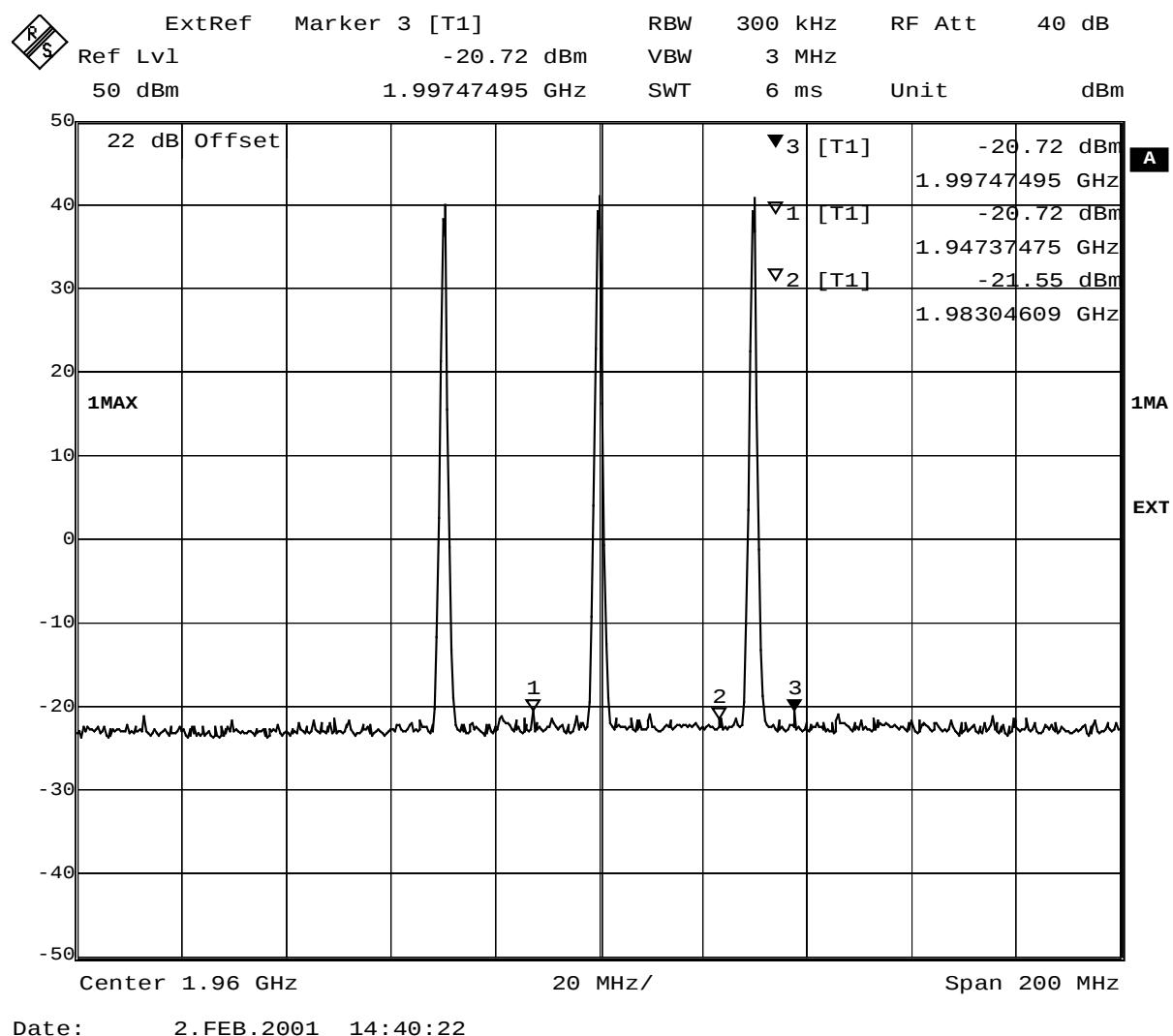
Fig. 41 – Slow frequency hopping – RBW = 300 kHz
