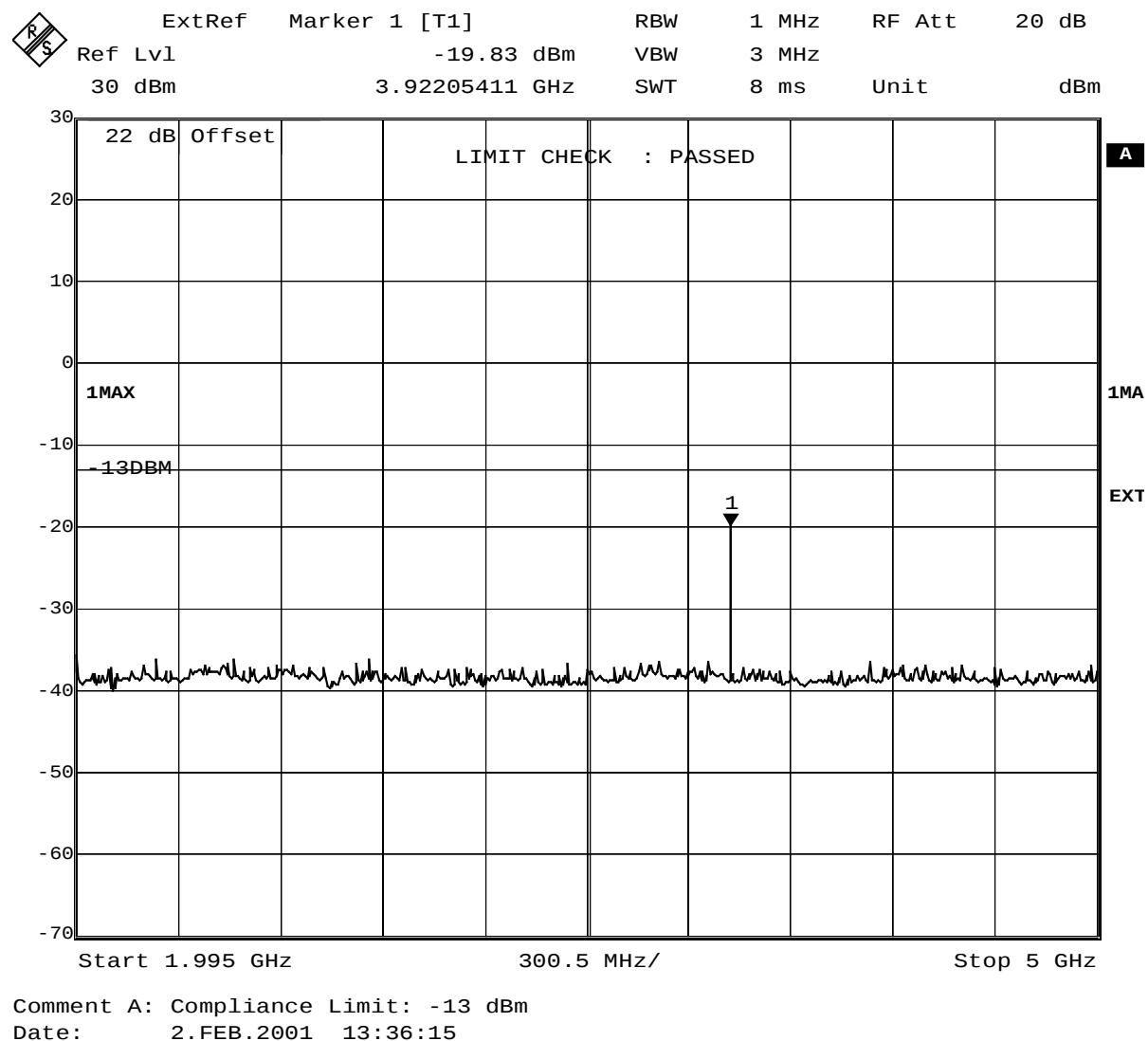
Fig. 21 – Spurious emissions in the frequency range 1995 MHz – 5000 MHz.
