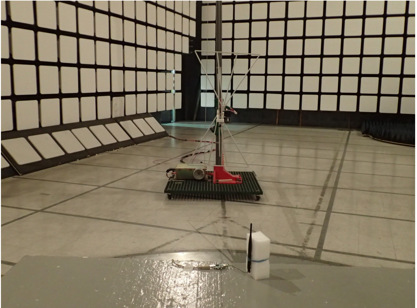
Radiated Emissions @ 3 m, Orthogonal Position 1
