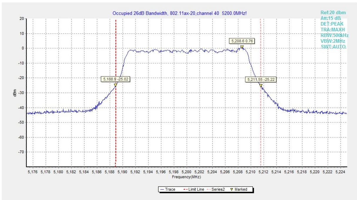
Fig.12 Occupied 26dB Bandwidth (802.11ax-HE20, 5200MHz)
