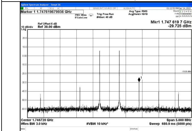
AWS Band Pre AGC, UL
