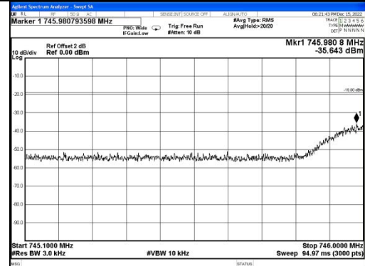
Upper 700MHz band2 GSM DL Right Side 10dB Above AGC
