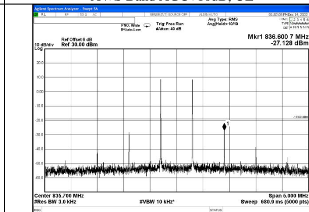
Cellular Band AGC+10dB, UL
