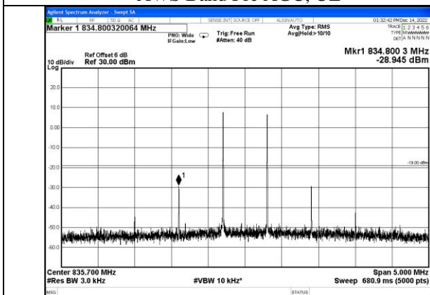
Cellular Band Pre AGC, UL
