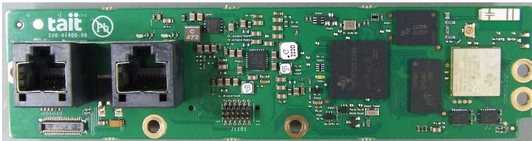
Photograph 03: UnifyVehicle PCB - top
