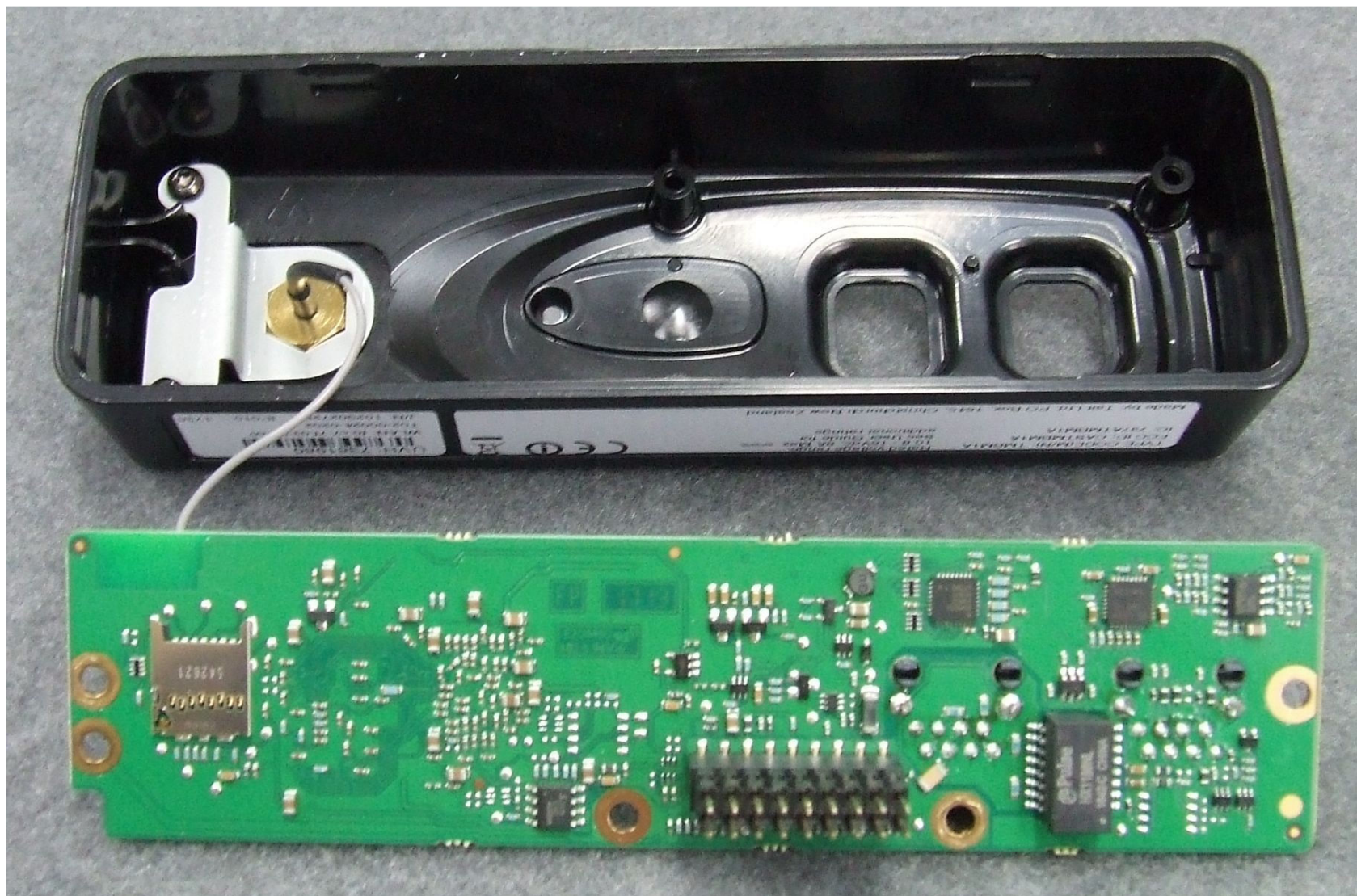
Photograph 02: UnifyVehicle PCB removed from casing
