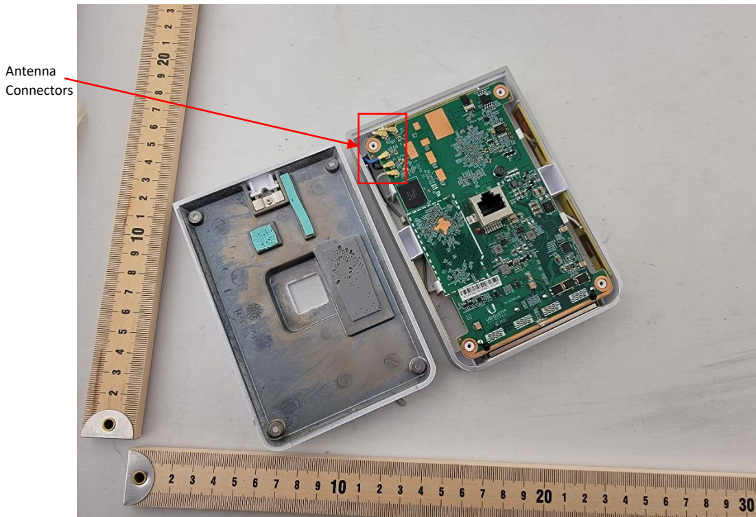
Photograph 1: Back View of Circuit Board Inside Case
