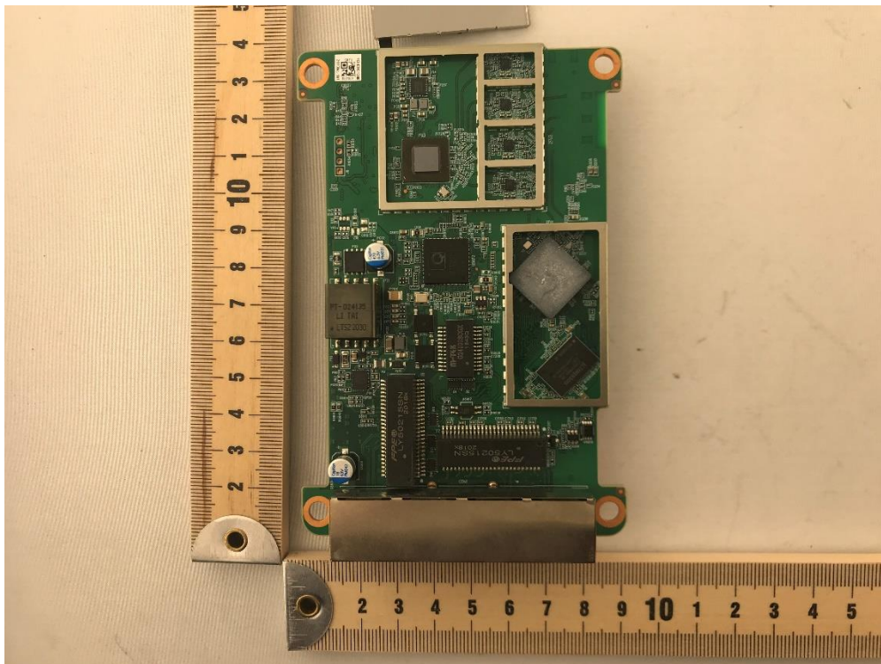
Photograph 4: Top View of Circuit Board
