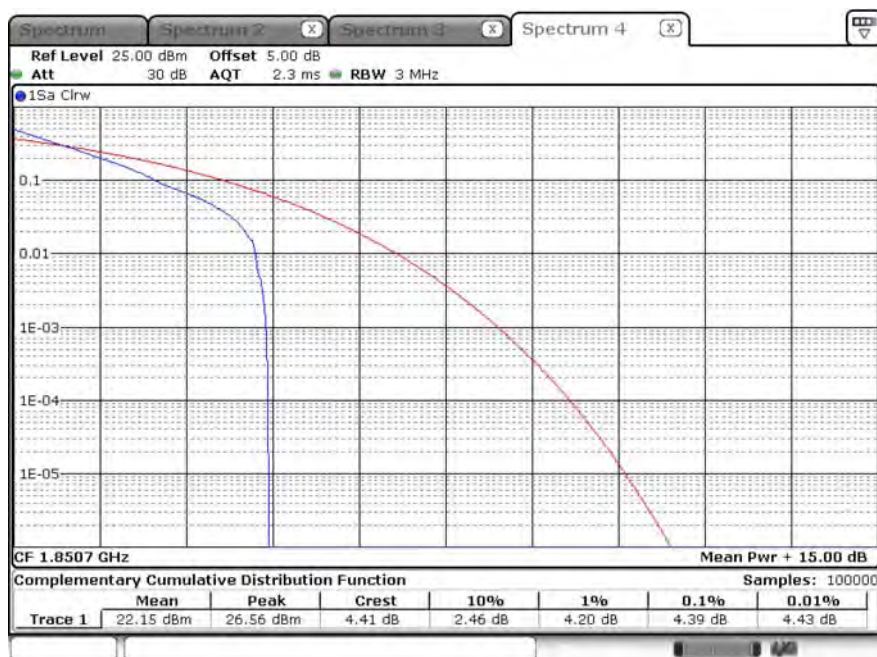
B25_CH26047_1.4M_1RB2_QPSK
