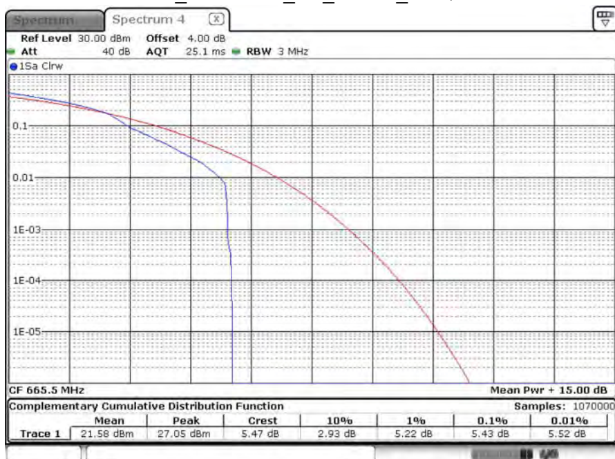
B71_CH133147_5M_1RB12_16-QAM
