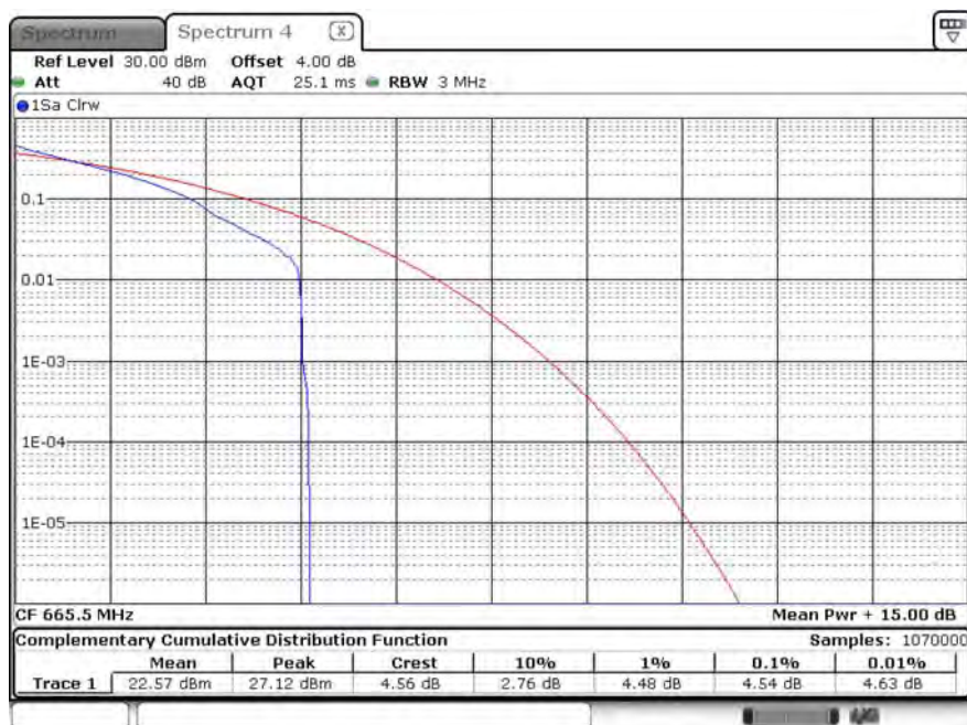
B71_CH133147_5M_1RB12_QPSK
