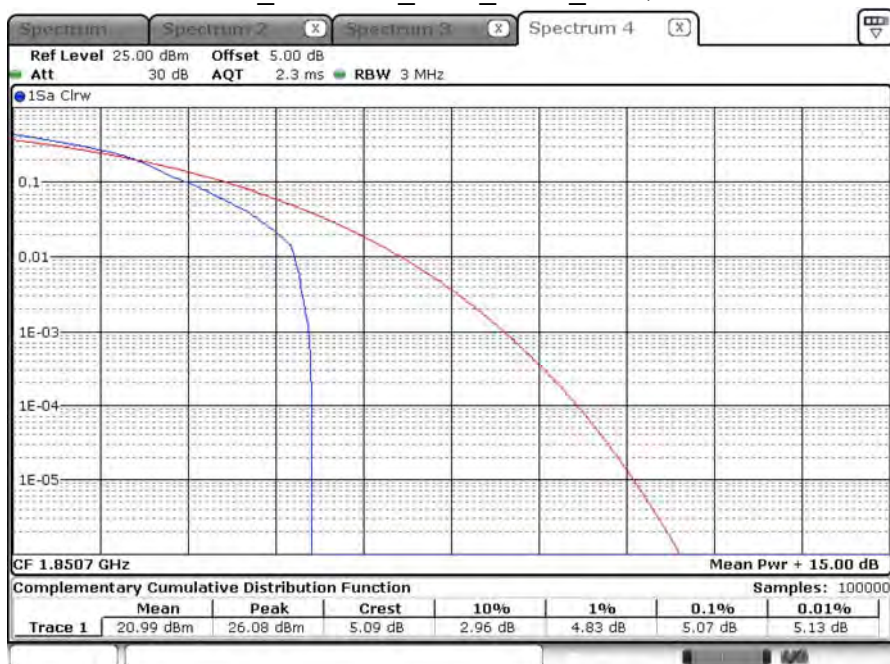
B25_CH26047_1.4M_1RB2_16-QAM
