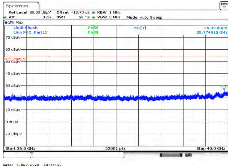
Plot 36: 26 GHz to 40 GHz; vertical & horizontal polarization; U-NII-2A; lowest channel
