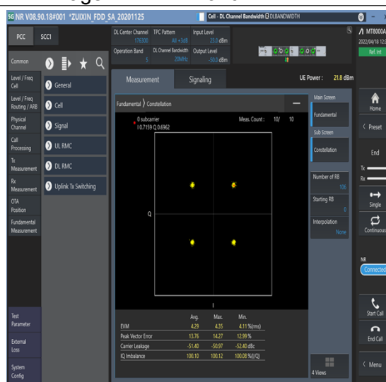
1-N5--15-20-M-6-CP-QPSK-Outer_Full-106@0-Ant1-see graph-PASS
