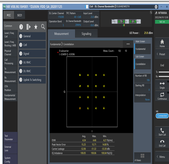
1-N5--15-20-M-7-CP-16QAM-Outer_Full-106@0-Ant1-see graph-PASS
