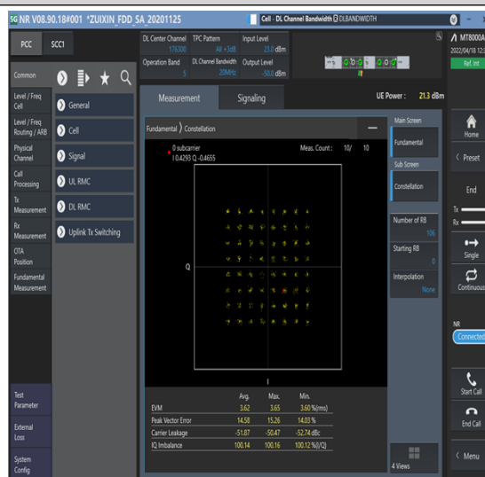
1-N5--15-20-M-8-CP-64QAM-Outer_Full-106@0-Ant1-see graph-PASS
