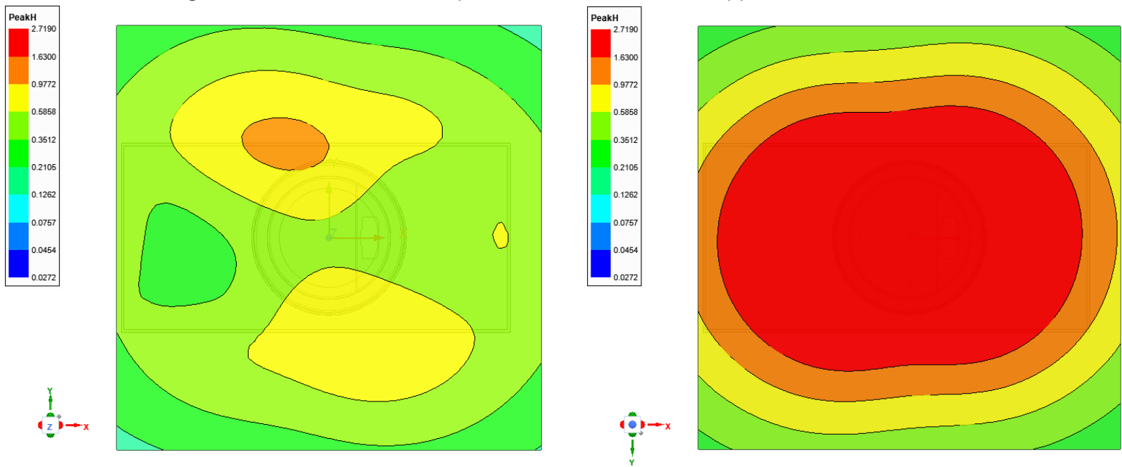
Figure 13: H-field on the two planes for case 505 from MagSafe simulation model.
