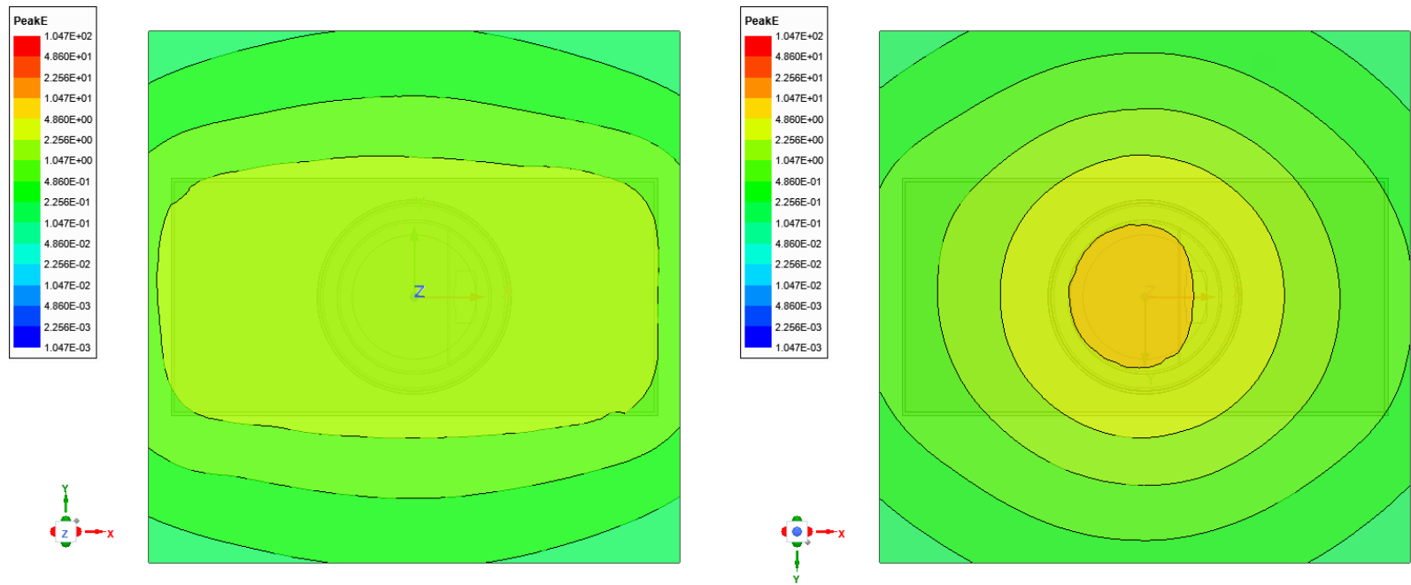
Figure 11: E-field on the two planes for case 000 from MagSafe simulation model.
