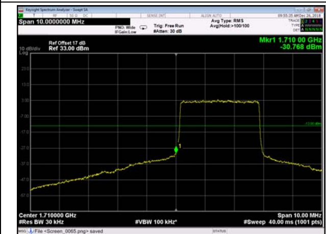
LowRange_FDD04_5MHz_1712.5_OneRB _low_Q16
