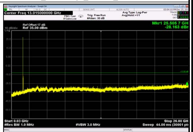
FDD66_LowRange_5MHz_30MHz~26GHz
