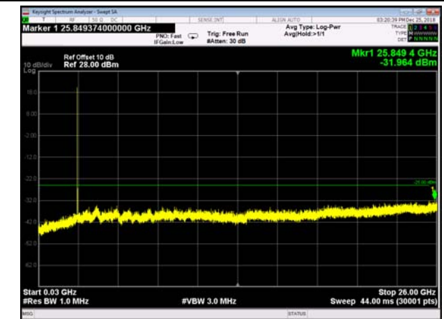
FDD07_HighRange_5MHz_30MHz~26GHz
