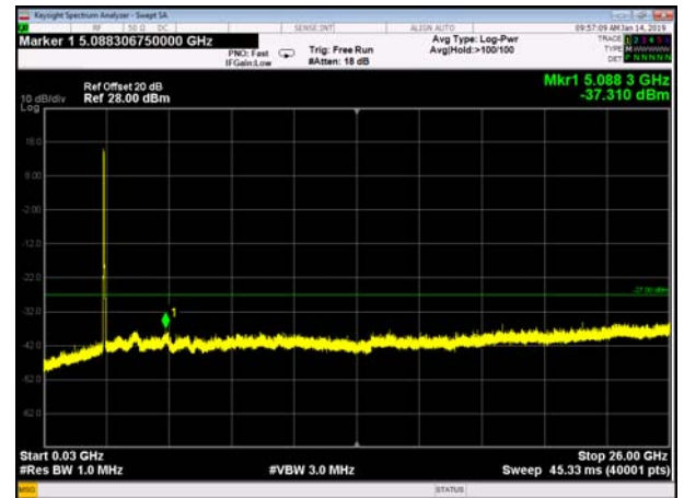
FDD7_LowRange_20+15MHz_30MHz~26GHz
