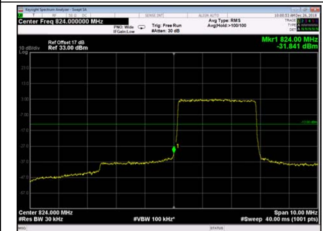
LowRange_FDD05_5MHz_826.5_OneRB _low_Q16
