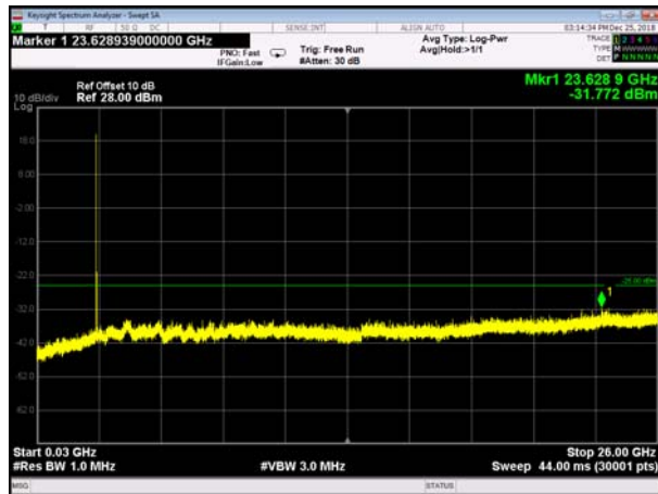
FDD07_MidRange_10MHz_30MHz~26GHz
