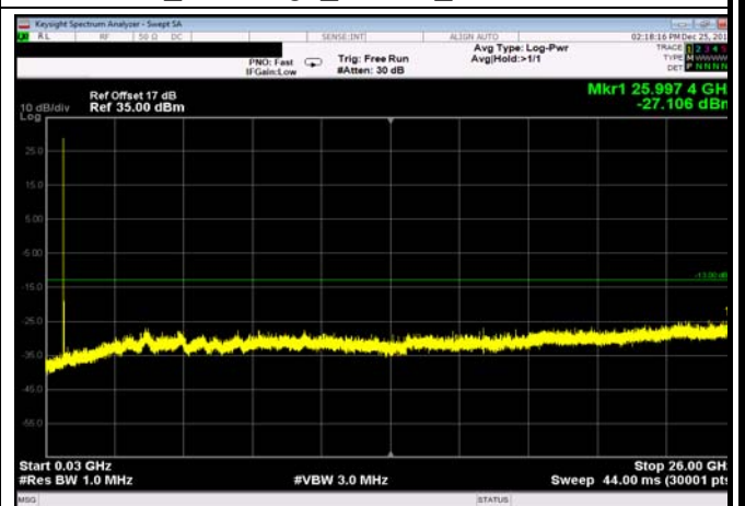
FDD12_MidRange_5MHz_30MHz~26GHz
