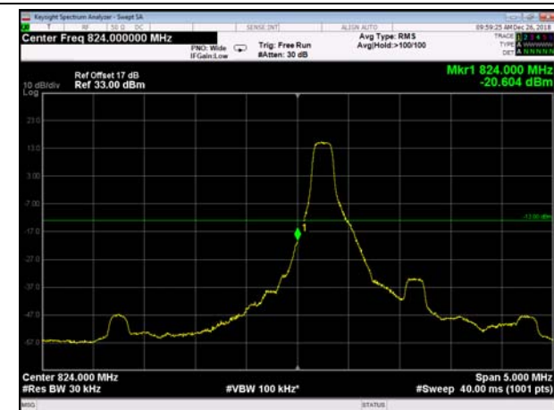
LowRange_FDD05_1.4MHz_824.7_fullRB _Low_QPSK
