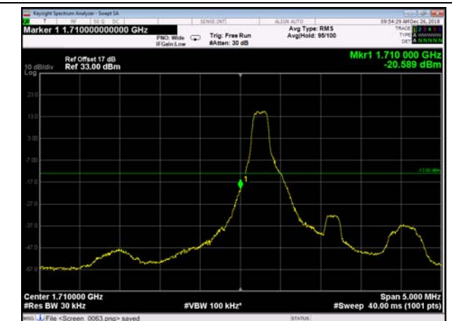
LowRange_FDD04_1.4MHz_1710.7_fullRB _Low_Q16
