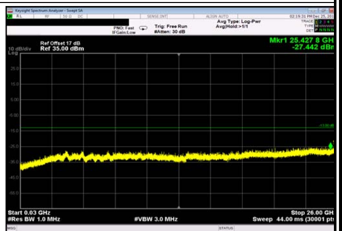
FDD66_LowRange_20MHz_30MHz~26GHz
