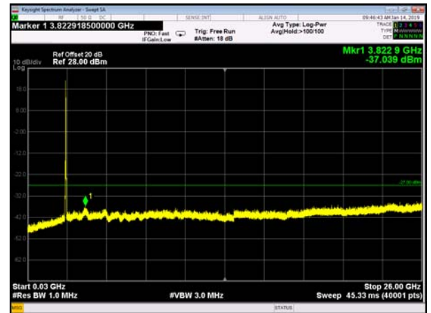
FDD7_LowRange_15+20MHz_30MHz~26GHz
