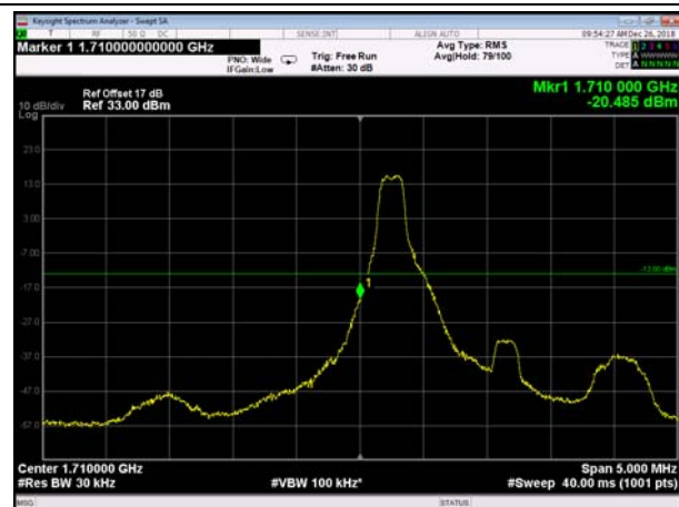
LowRange_FDD04_1.4MHz_1710.7_fullRB _Low_QPSK
