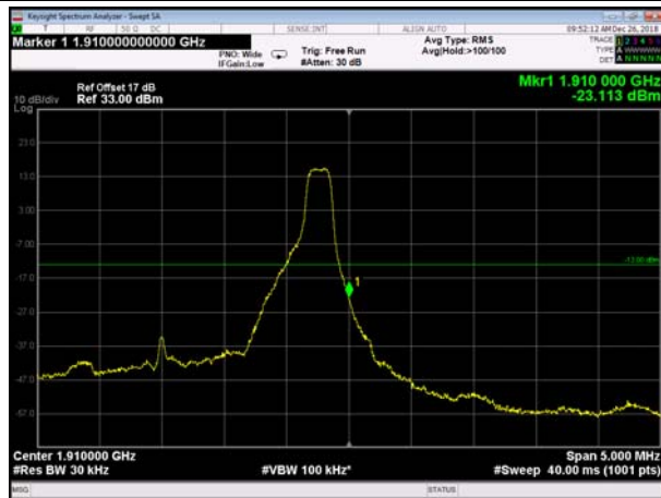
HighRange_FDD02_3MHz_1908.5_fullRB _High_QPSK
