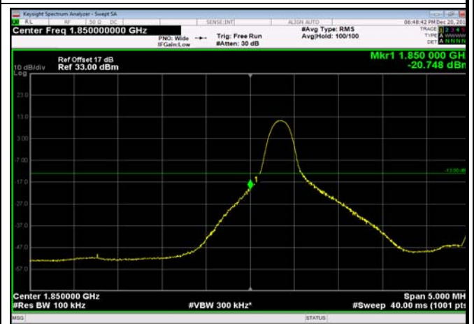
LowRange_FDD02_5MHz_1852.5_OneRB _low_Q16
