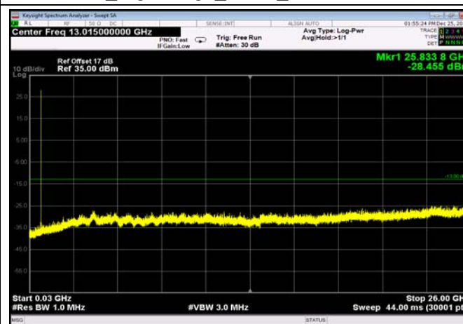
FDD12_LowRange_1.4MHz_30MHz~26GHz
