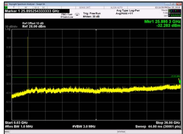
FDD07_MidRange_15MHz_30MHz~26GHz
