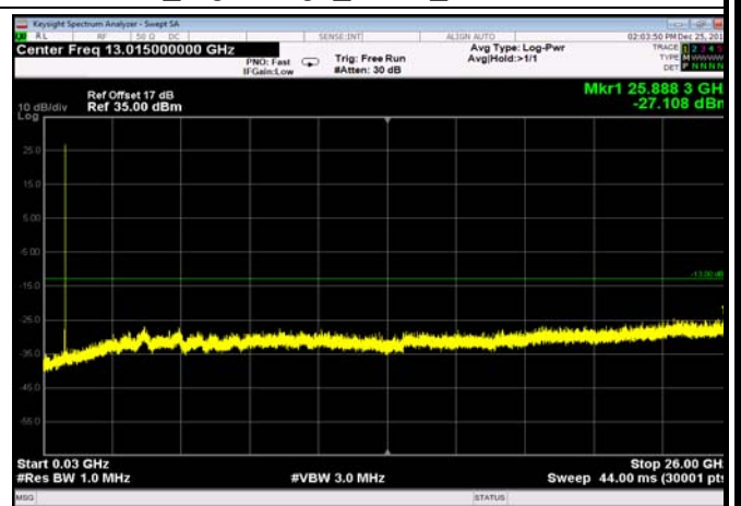
FDD05_LowRange_10MHz_30MHz~26GHz
