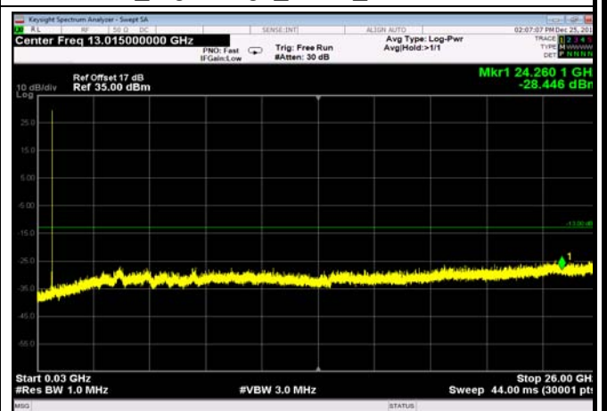
FDD12_LowRange_10MHz_30MHz~26GHz
