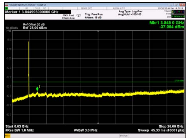
FDD7_HighRange_15+20MHz_30MHz~26GHz
