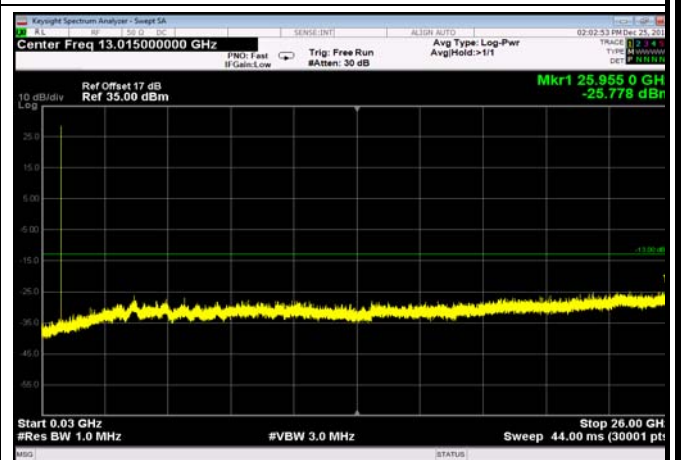
FDD05_MidRange_10MHz_30MHz~26GHz
