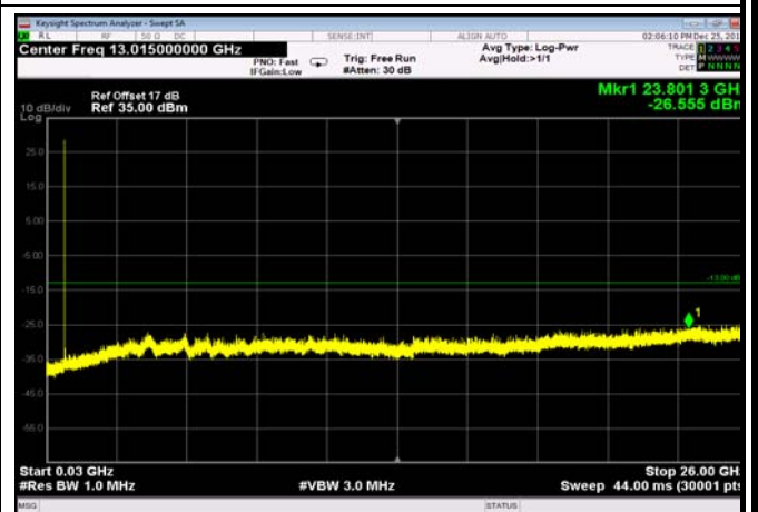
FDD12_MidRange_10MHz_30MHz~26GHz
