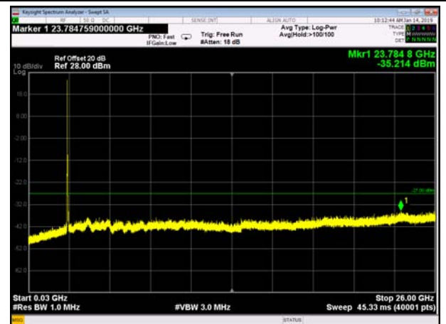
FDD7_HighRange_15+10MHz_30MHz~26GHz
