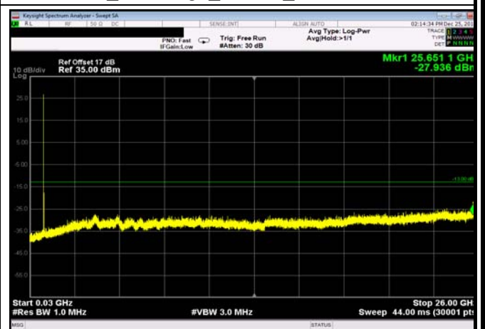
FDD05_MidRange_5MHz_30MHz~26GHz
