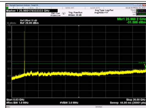
FDD07_LowRange_10MHz_30MHz~26GHz
