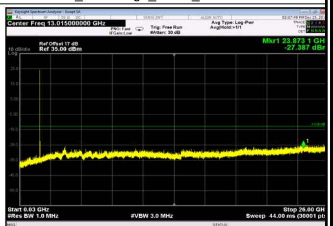
FDD66_LowRange_5MHz_30MHz~26GHz
