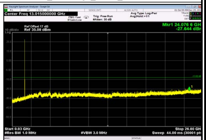
FDD66_MidRange_20MHz_30MHz~26GHz
