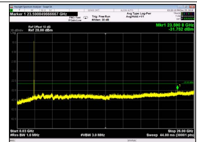
FDD07_LowRange_15MHz_30MHz~26GHz
