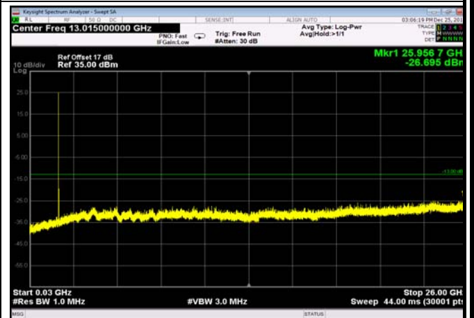
FDD66_HighRange_5MHz_30MHz~26GHz
