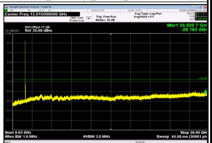
FDD66_MidRange_20MHz_30MHz~26GHz
