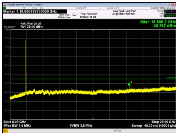
FDD7_HighRange_15+15MHz_30MHz~26GHz
