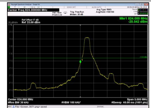
LowRange_FDD05_1.4MHz_824.7_fullRB _Low_Q16
