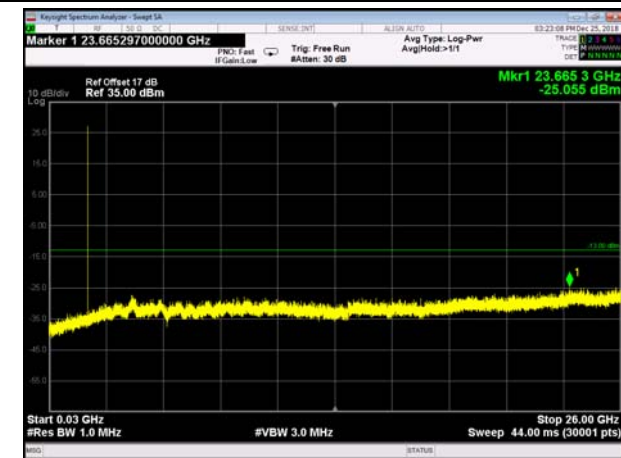
FDD66_HighRange_15MHz_30MHz~26GHz
