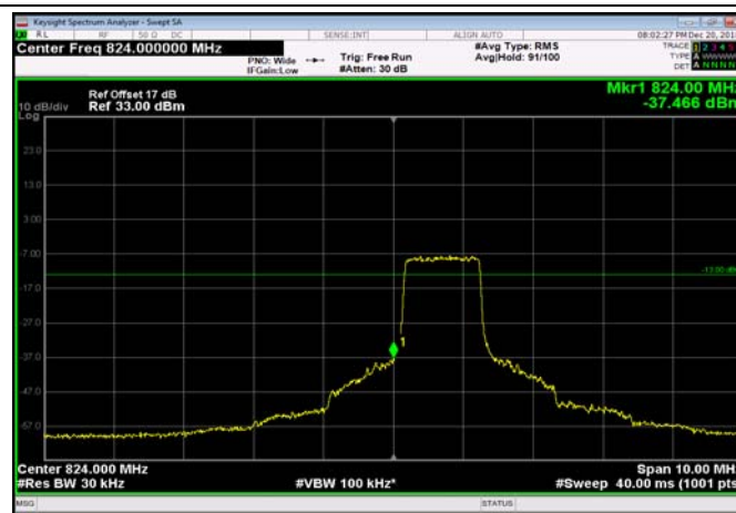
LowRange_FDD05_1.4MHz_824.7_fullRB _Low_QPSK
