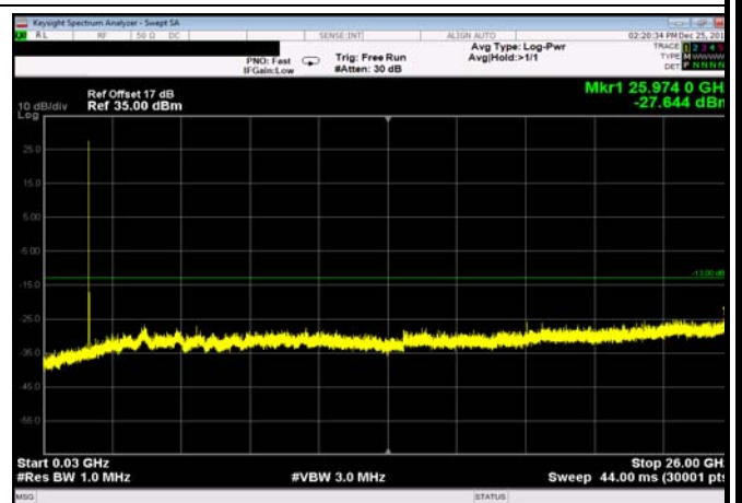
FDD66_MidRange_3MHz_30MHz~26GHz
