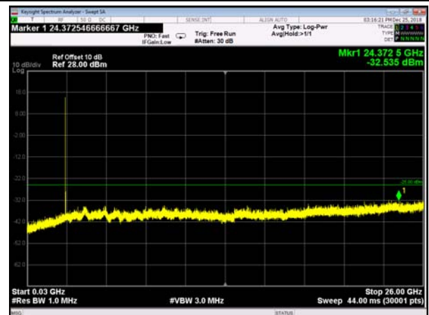
FDD07_MidRange_5MHz_30MHz~26GHz
