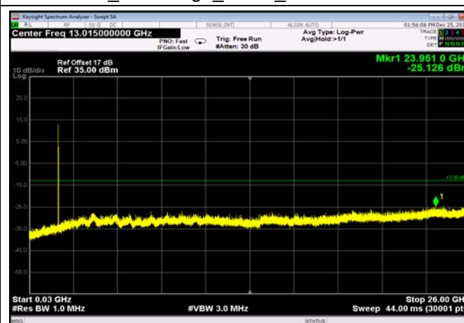
FDD66_LowRange_3MHz_30MHz~26GHz
