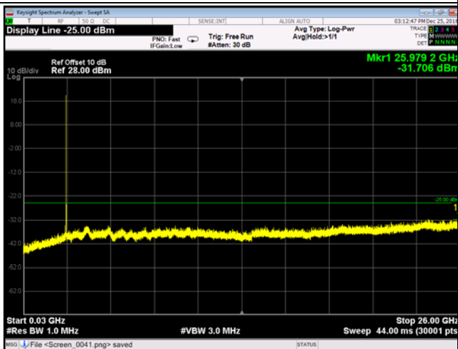
FDD07_LowRange_10MHz_30MHz~26GHz
