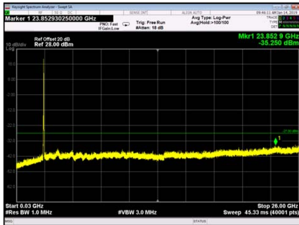
FDD7_HighRange_10+20MHz_30MHz~26GHz
