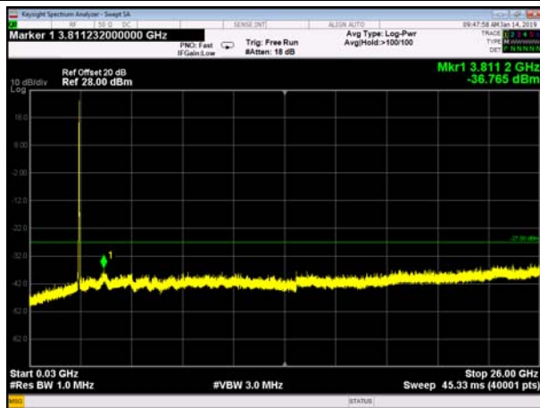
FDD7_MiddleRange_15+20MHz_30MHz~26GHz
