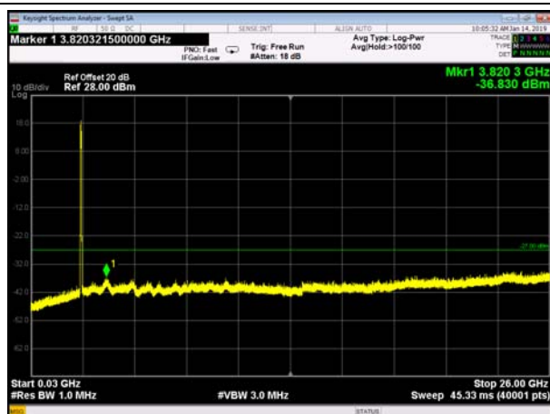
FDD7_MiddleRange_20+15MHz_30MHz~26GHz
