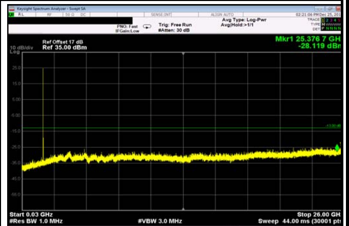
FDD66_HighRange_20MHz_30MHz~26GHz
