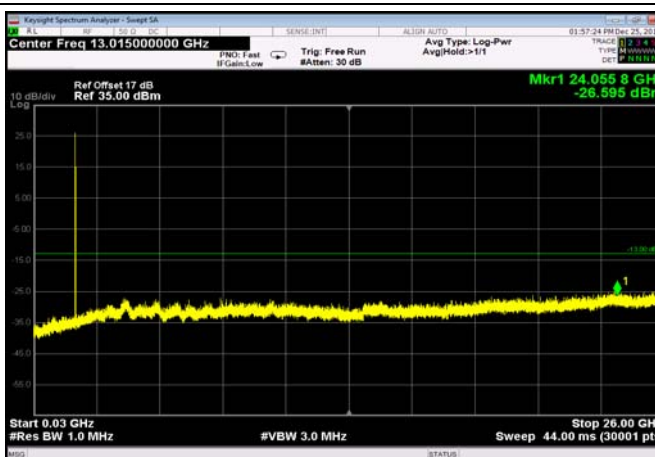
FDD66_HighRange_3MHz_30MHz~26GHz
