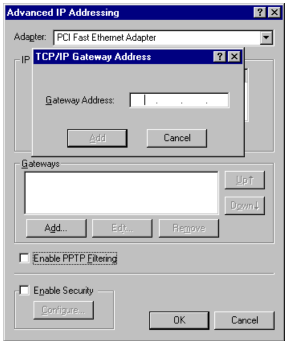
Figure 58 - Windows NT4.0 - Add Gateway
