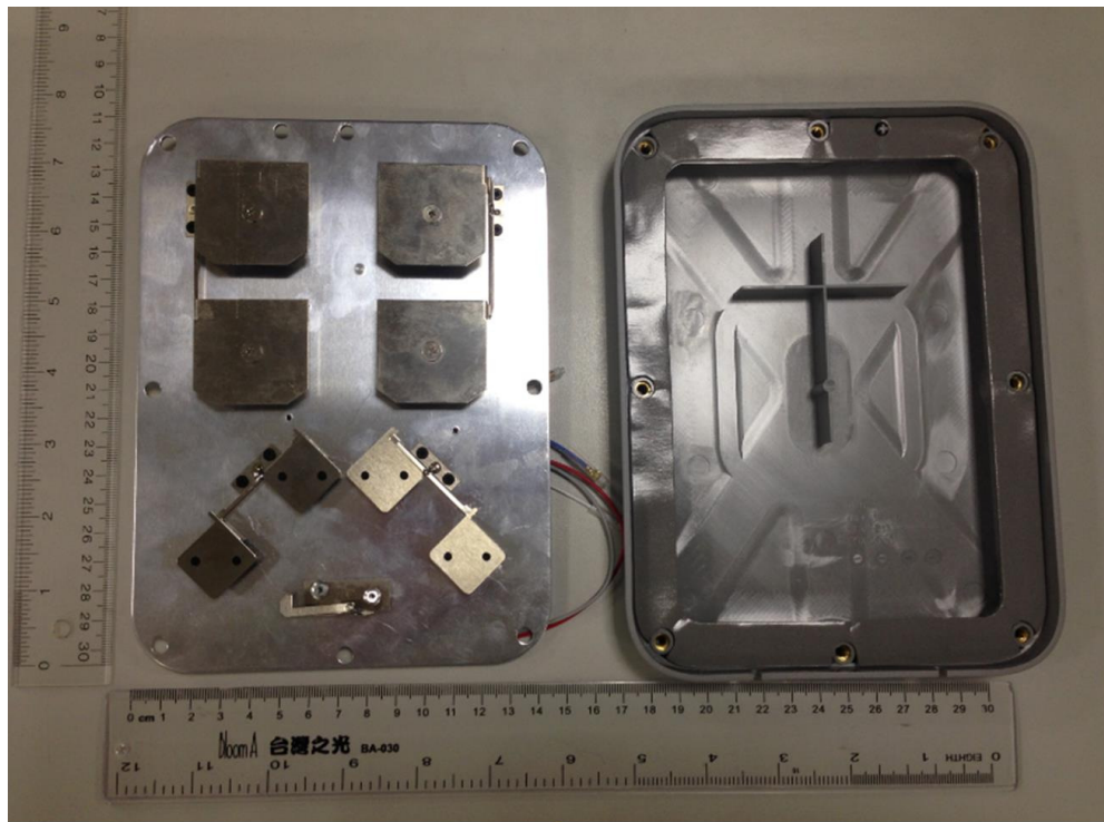
1542D antenna
