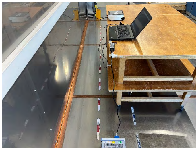
Photograph for AC Power Line Conducted Emissions (with Laptop)
