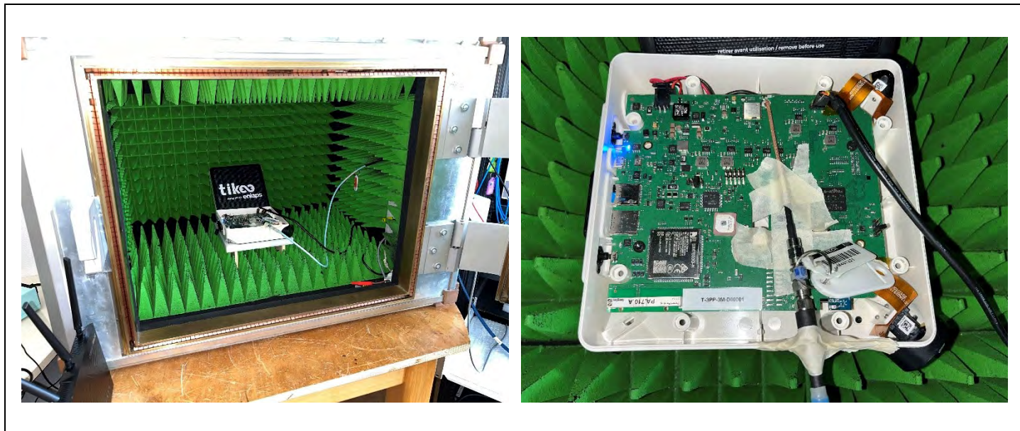
Photograph for Unwanted Emission into non-restricted frequency bands at the band edge
