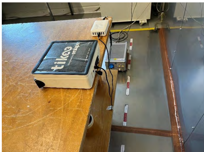
Photograph for AC Power Line Conducted Emissions (with AC/DC Adapter
