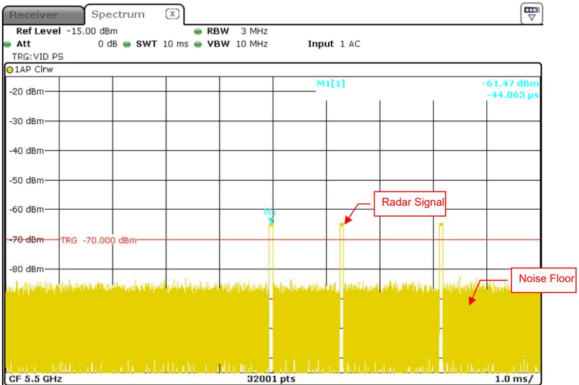
Single Burst of Radar Signal 5
