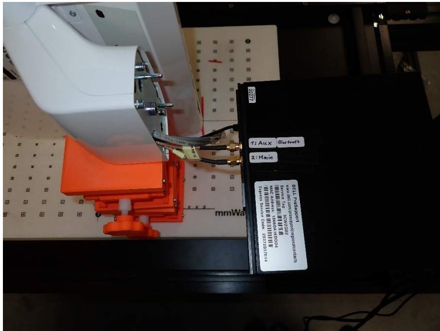
Figure D.3: DUT test set for left side.
