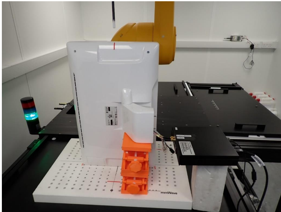
Figure D.1: DUT left side test setup.
