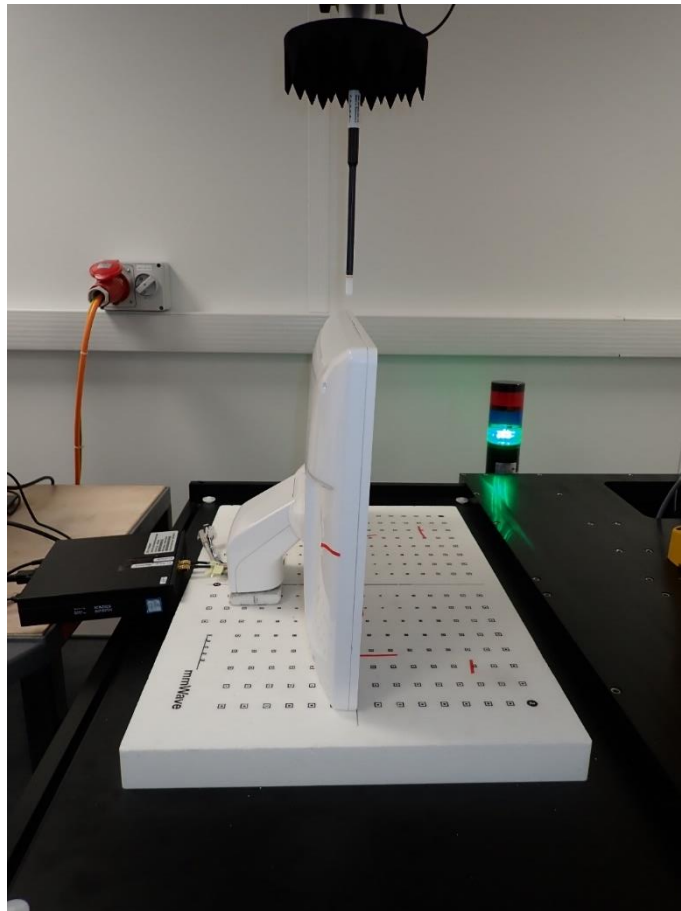
Figure D.5: DUT top side test setup.
