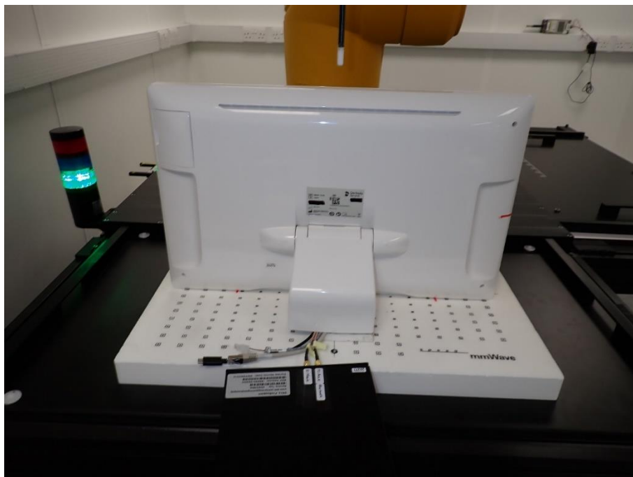
Figure D.4: DUT top side test setup.
