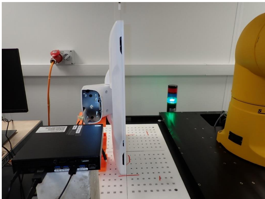
Figure D.2: DUT left side test setup.
