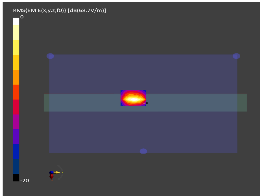
Figure C.1: SAR Testing Results for the Primescan 2 CART at 6025 MHz
