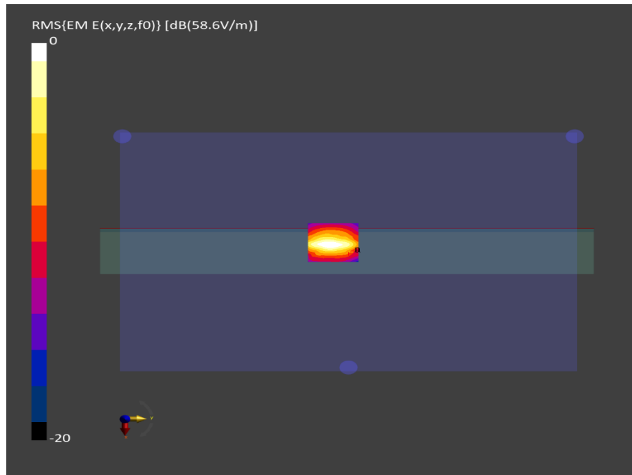
Figure C.2: SAR Testing Results for the Primescan 2 CART at 6025 MHz
