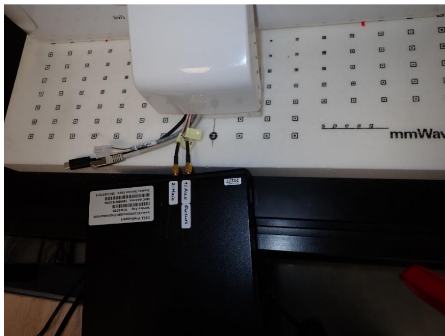
Figure D.6: DUT test set for top side.
