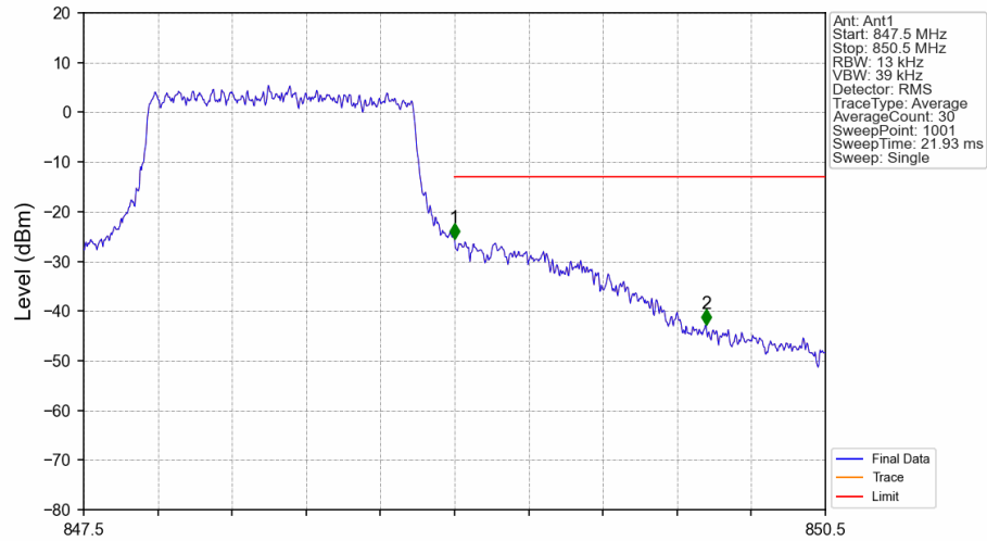
Band5_1.4MHz_16QAM_HCH_848.3MHz_RB_6_0_NTNV
