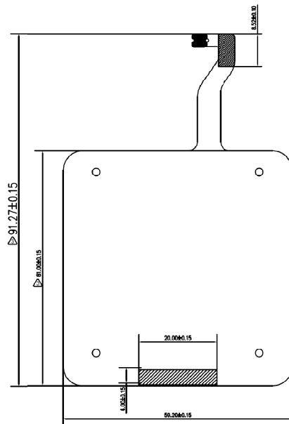
WPT Antenna (Configuration 2)
