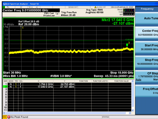
Band4 / 3MHz / Low CH / QPSK
