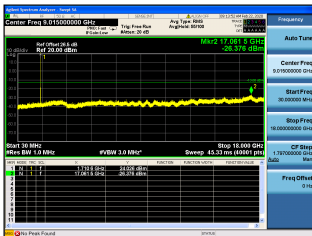
Band4 / 3MHz / Low CH / 64QAM
