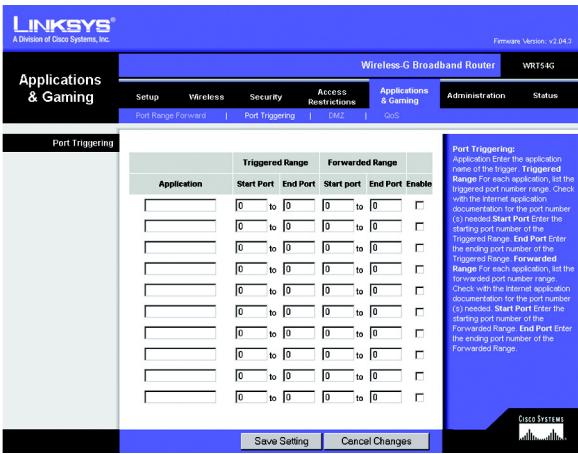
Figure 6-32: Applications and Gaming Tab - Port Triggering
