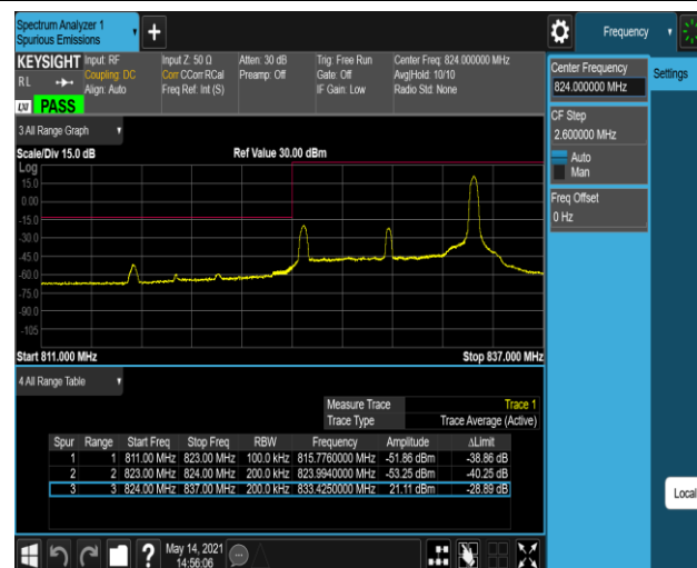
Band5-10MHz-16QAM-20600-1RB#0
