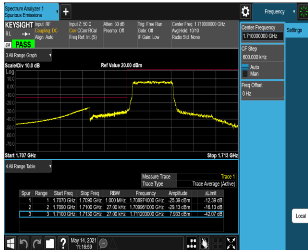
Band4-1.4MHz-16QAM-20393-1RB#5
