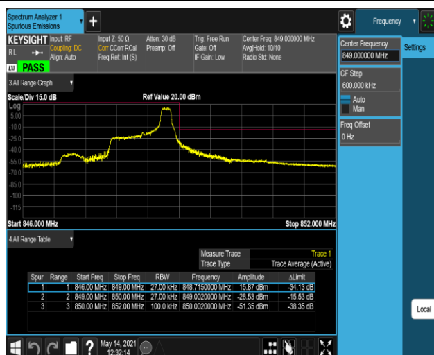
Band5-1.4MHz-QPSK-20643-1RB#5
