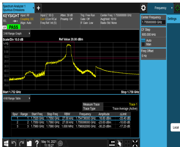
Band4-1.4MHz-16QAM-20393-1RB#5
