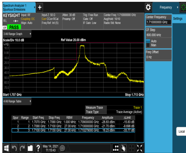
Band4-1.4MHz-16QAM-19957-6RB#0
