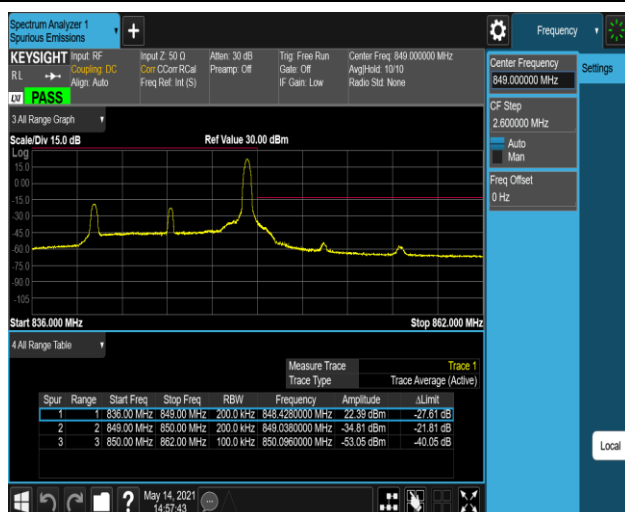
Band5-10MHz-QPSK-20600-1RB#49
