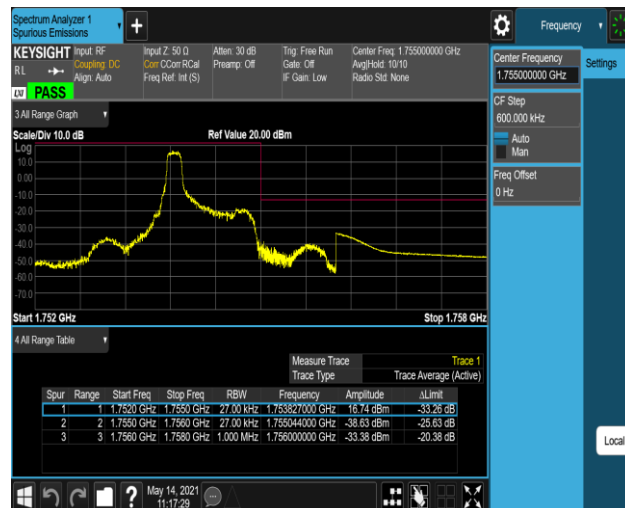
Band4-1.4MHz-QPSK-20393-6RB#0
