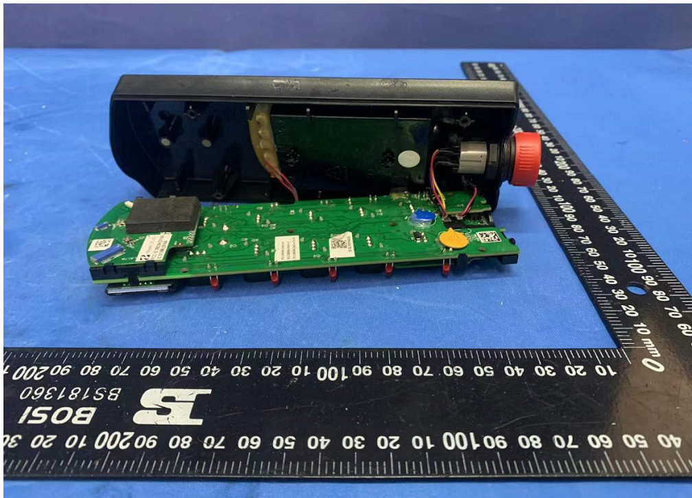
PCB view of AL022
