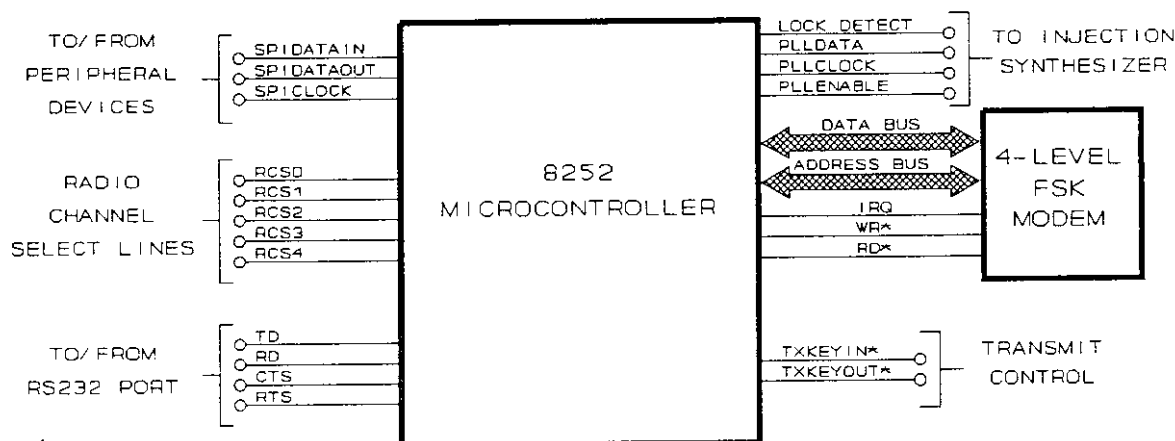
Figure 3. Microcontroller Functional Block Diagram
