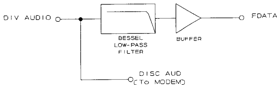
Figure 20. Receive Baseband Processing
