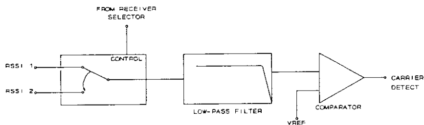
Figure 19. Carrier Detector Functional Diagram
