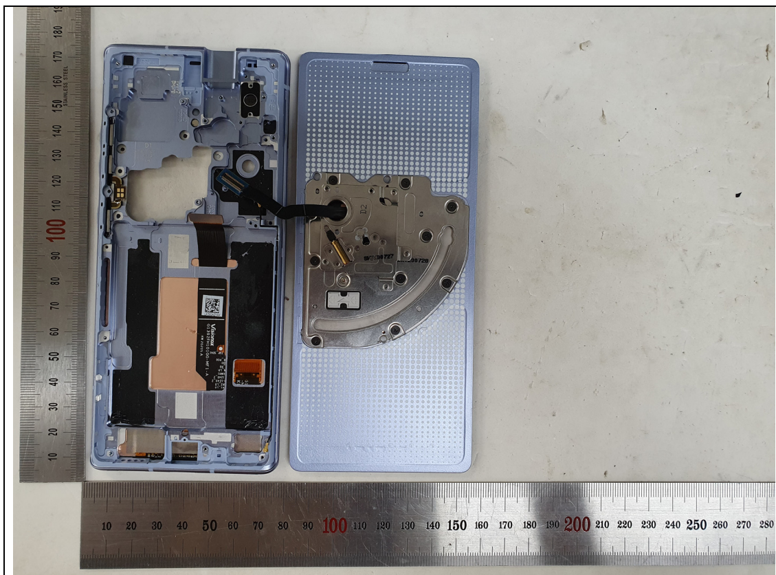
&lt;swivel display &amp; non-swivel display _ back view&gt;
