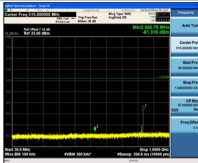
Band5-1.4MHz-QPSK-20525-1-0-Low-30-1000--61.32-PASS
