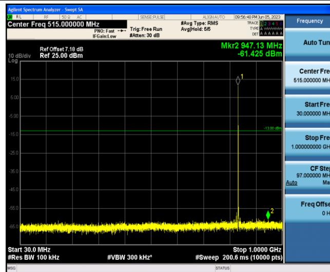
Band5-1.4MHz-16QAM-20525-1-0-Low-30-1000--61.43-PASS
