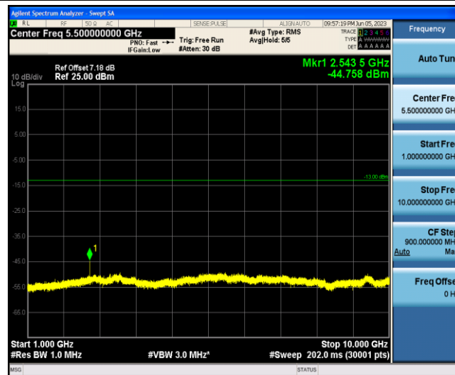
Band5-1.4MHz-QPSK-20643-1-0-Low-1000-10000--44.76-PASS
