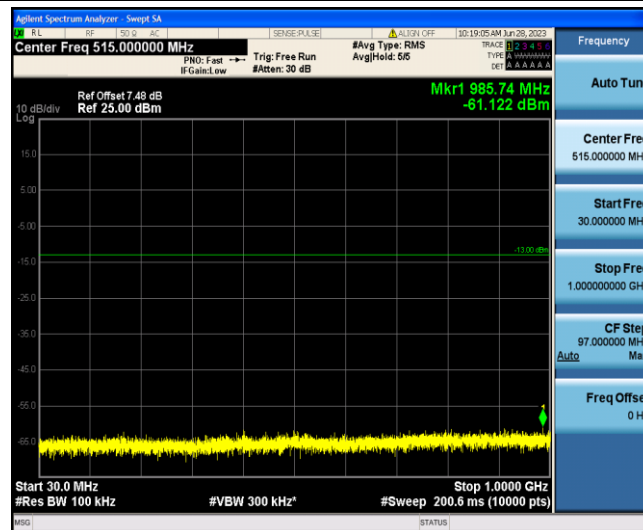
Band4-20MHz-16QAM-20175-1-0-Low-30-1000--61.12-PASS
