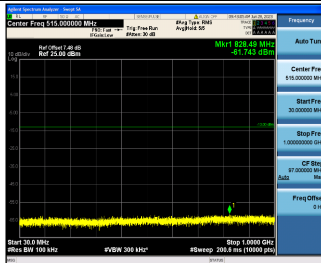
Band4-10MHz-QPSK-20175-1-0-Low-30-1000--61.74-PASS
