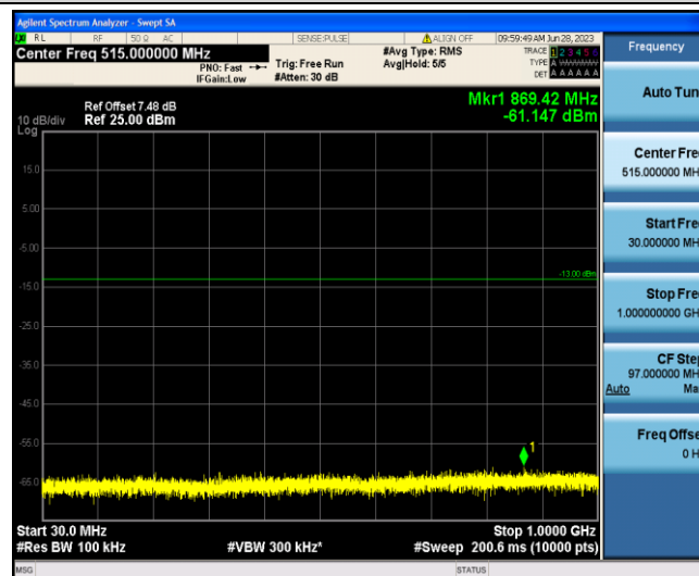
Band4-15MHz-QPSK-20175-1-0-Low-30-1000--61.15-PASS
