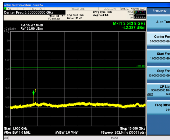
Band5-1.4MHz-16QAM-20643-1-0-Low-1000-10000--42.39-PASS
