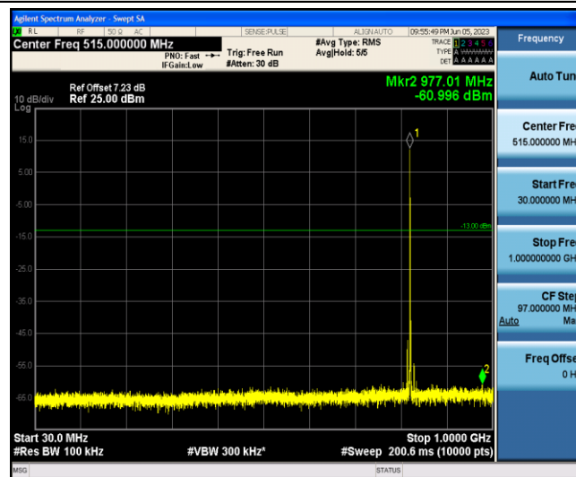
Band5-1.4MHz-QPSK-20407-1-0-Low-30-1000--61-PASS
