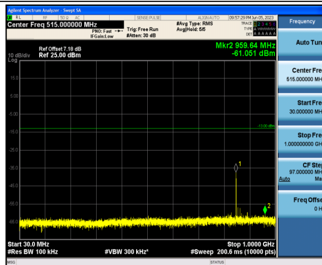
Band5-1.4MHz-16QAM-20643-1-0-Low-30-1000--61.05-PASS
