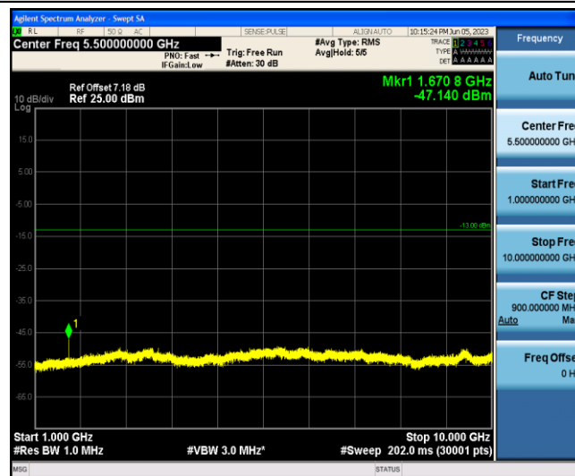
Band5-3MHz-QPSK-20525-1-0-Low-1000-10000--47.14-PASS
