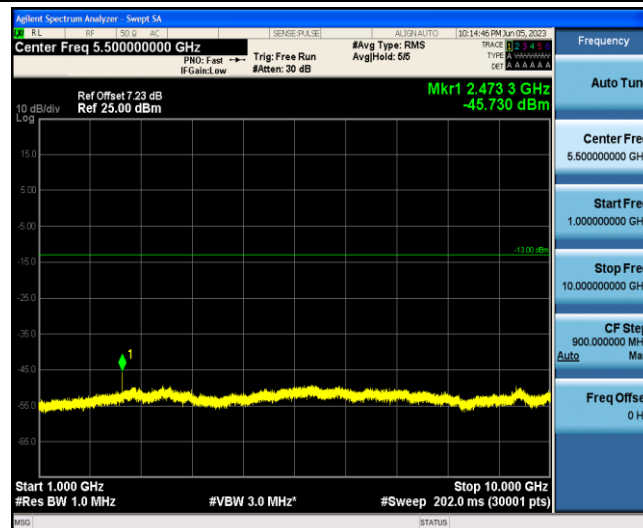
Band5-3MHz-QPSK-20415-1-0-Low-1000-10000--45.73-PASS
