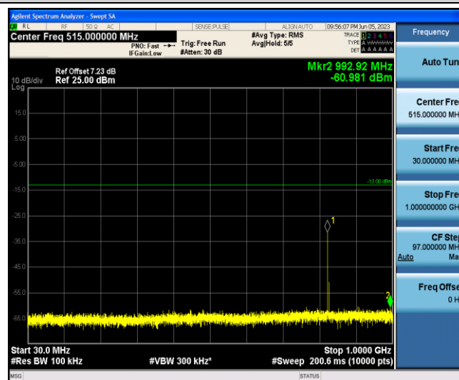
Band5-1.4MHz-16QAM-20407-1-0-Low-30-1000--60.98-PASS
