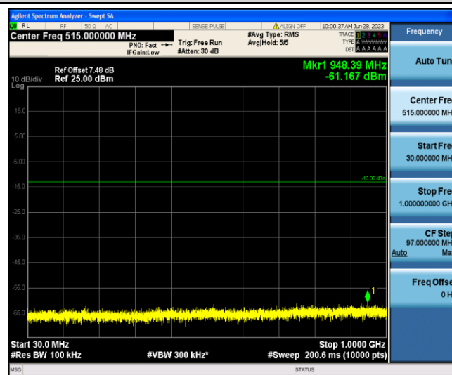
Band4-15MHz-QPSK-20325-1-0-Low-30-1000--61.17-PASS
