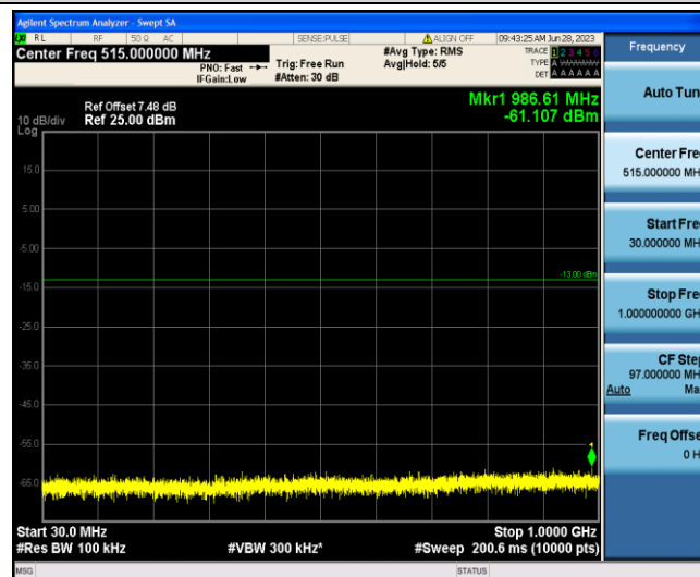
Band4-10MHz-16QAM-20175-1-0-Low-30-1000--61.11-PASS
