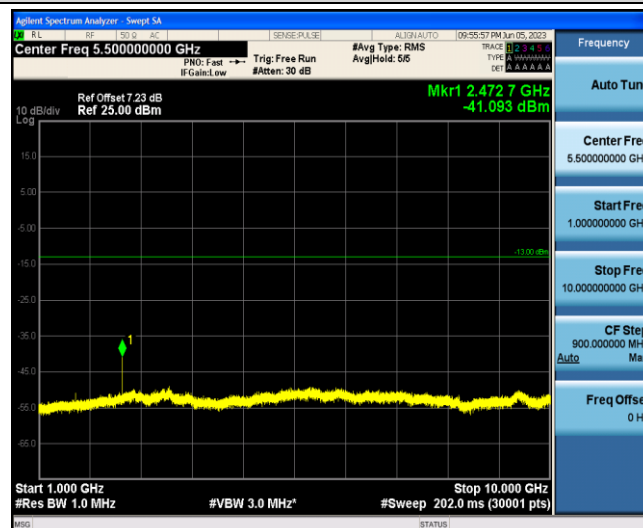
Band5-1.4MHz-QPSK-20407-1-0-Low-1000-10000--41.09-PASS
