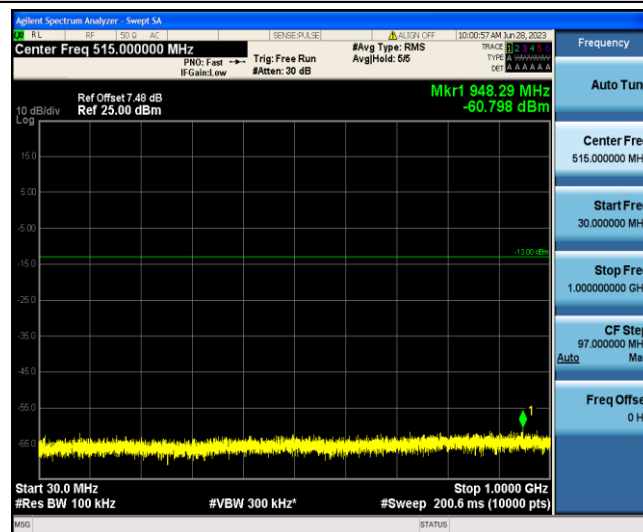
Band4-15MHz-16QAM-20325-1-0-Low-30-1000--60.8-PASS
