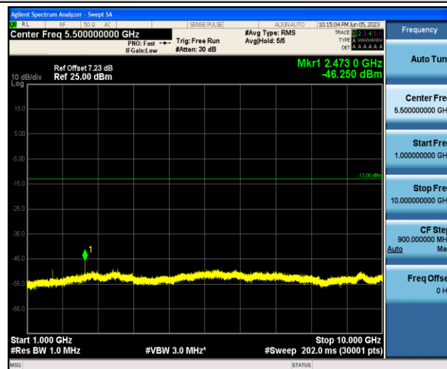
Band5-3MHz-16QAM-20415-1-0-Low-1000-10000--46.25-PASS
