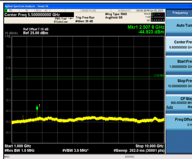
Band5-1.4MHz-QPSK-20525-1-0-Low-1000-10000--44.92-PASS
