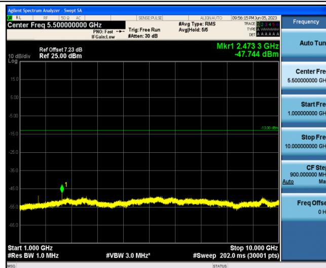
Band5-1.4MHz-16QAM-20407-1-0-Low-1000-10000--47.74-PASS
