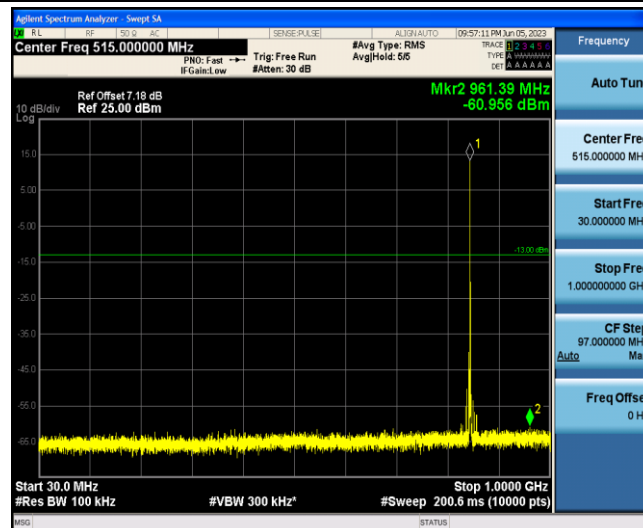
Band5-1.4MHz-QPSK-20643-1-0-Low-30-1000--60.96-PASS
