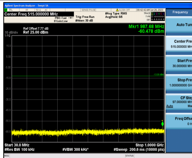
Band4-10MHz-16QAM-20000-1-0-Low-30-1000--60.48-PASS
