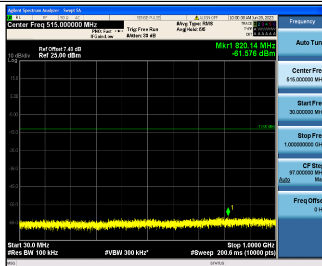
Band4-15MHz-16QAM-20175-1-0-Low-30-1000--61.58-PASS
