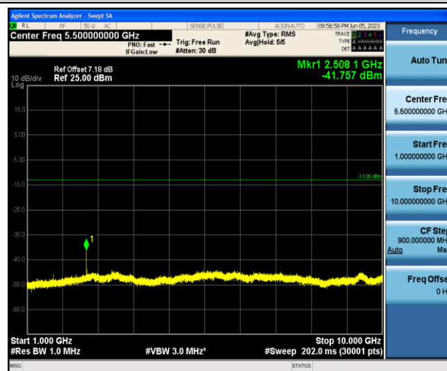
Band5-1.4MHz-16QAM-20525-1-0-Low-1000-10000--41.76-PASS
