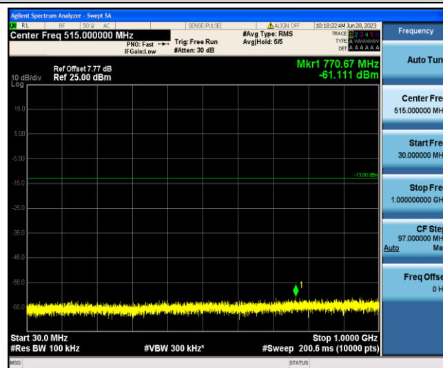
Band4-20MHz-16QAM-20050-1-0-Low-30-1000--61.11-PASS
