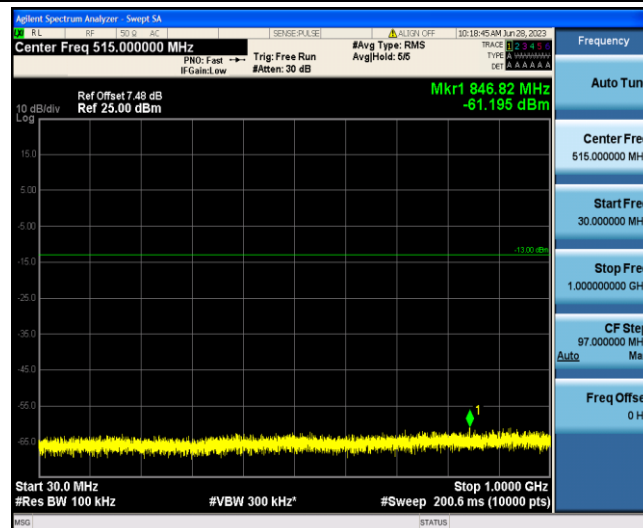
Band4-20MHz-QPSK-20175-1-0-Low-30-1000--61.2-PASS
