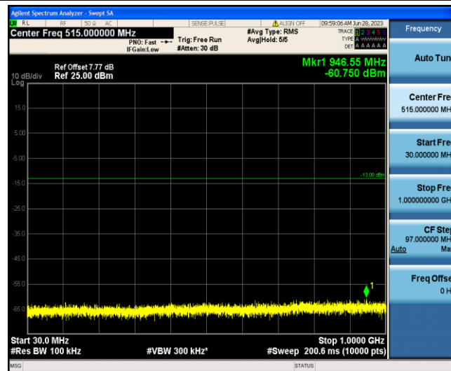
Band4-15MHz-QPSK-20025-1-0-Low-30-1000--60.75-PASS
