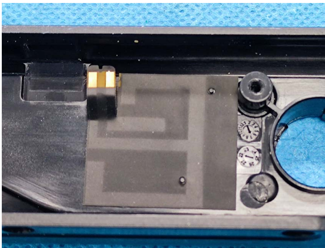
Bluetooth Antenna
