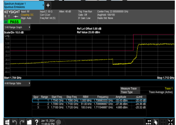
B4 5M QPSK 25@0 CH 19975
