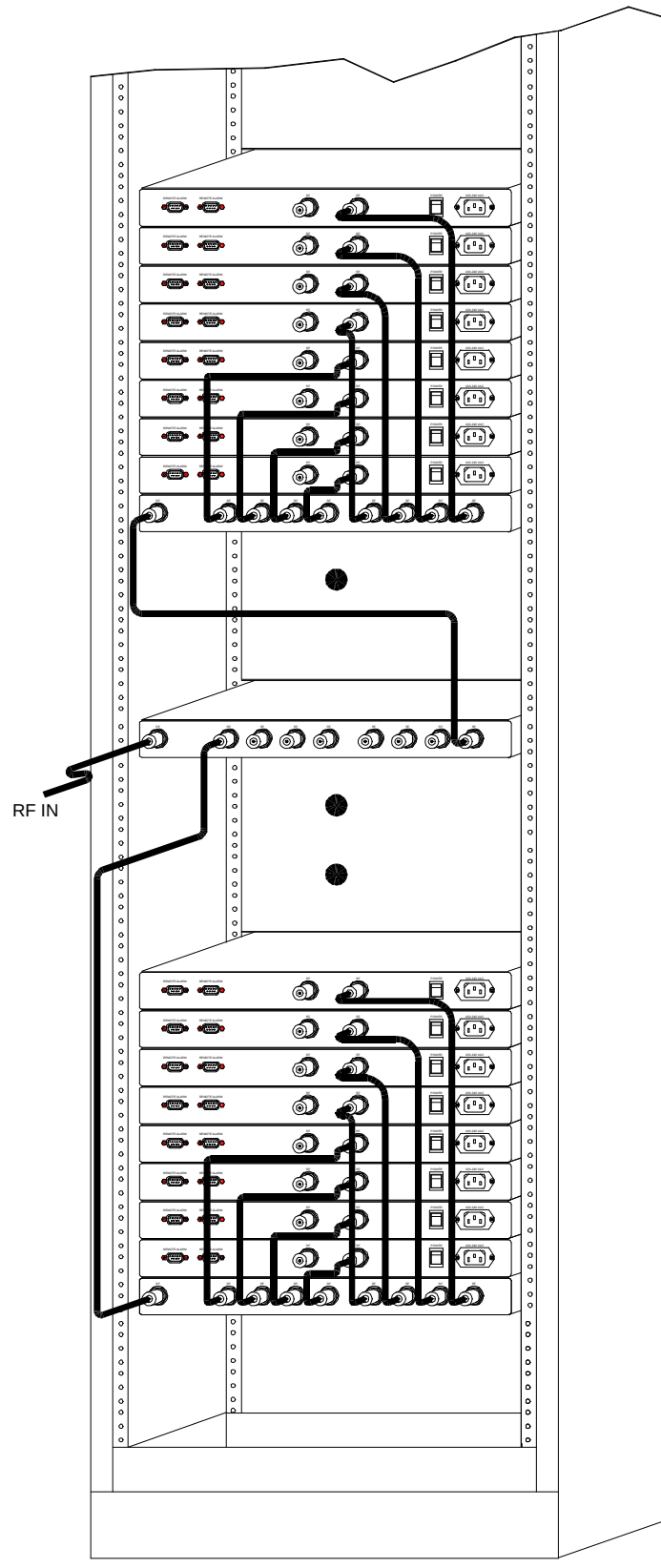
Figure 9. System Expandability to more than 48 RAUs
