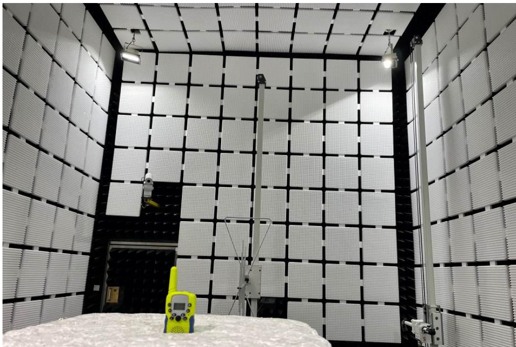
Below 1GHz
