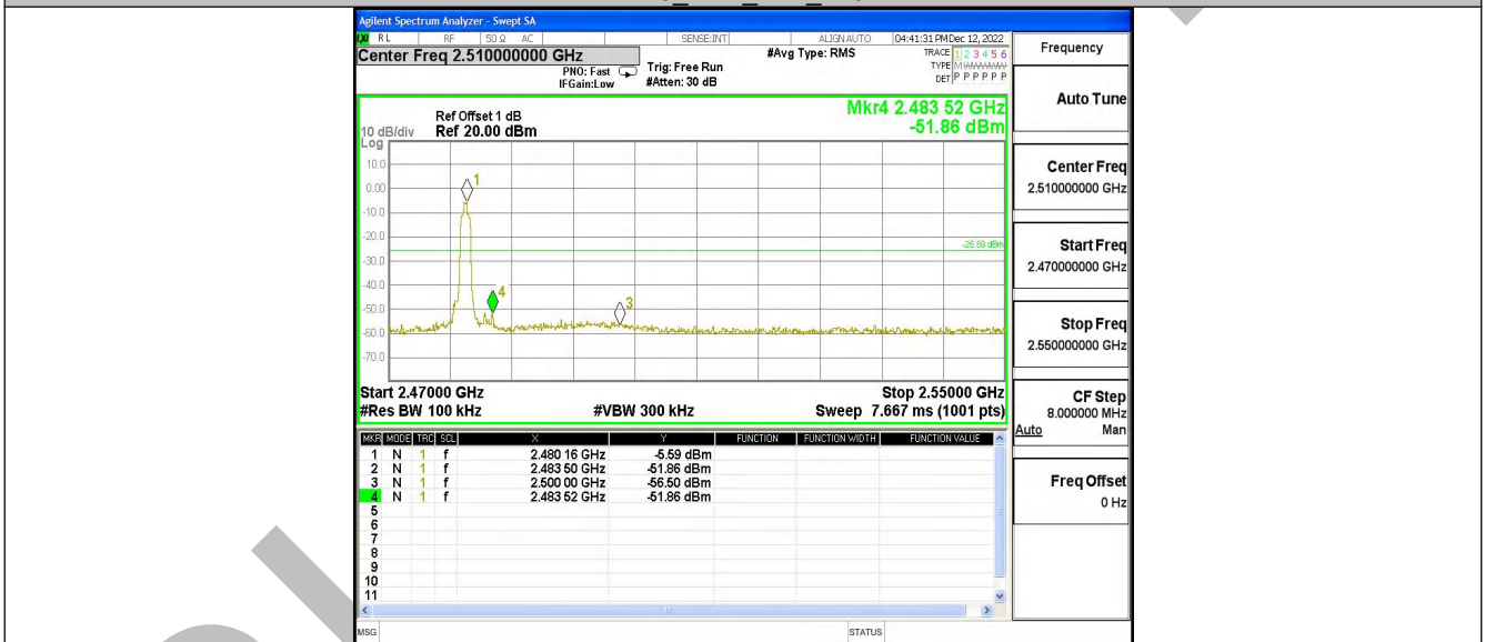
2DH5_Ant1_High_2480
