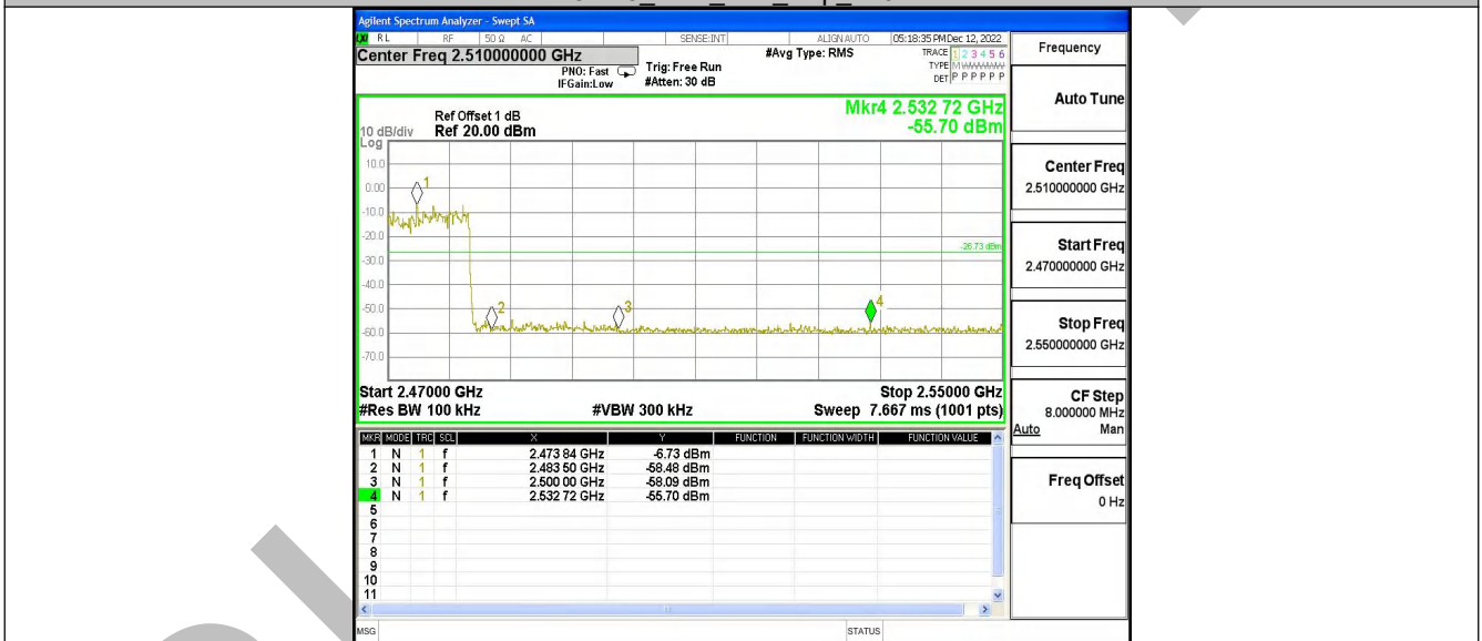
3DH5_Ant1_High_Hop_2480
