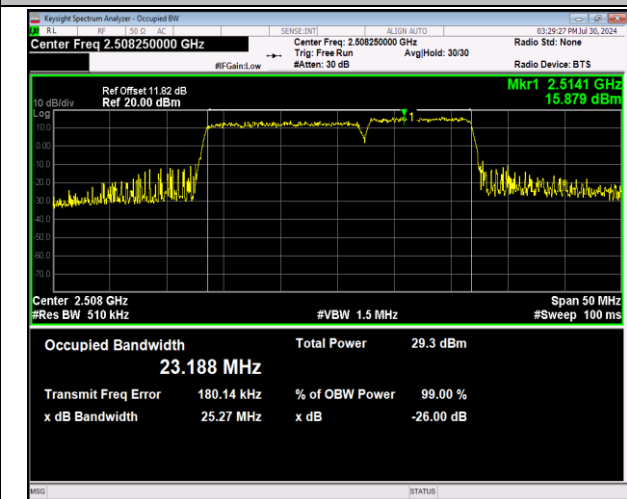
41-41-15MHz-10MHz-64QAM-64QAM-39725-39845-75RB#0 -50RB#0-PASS
