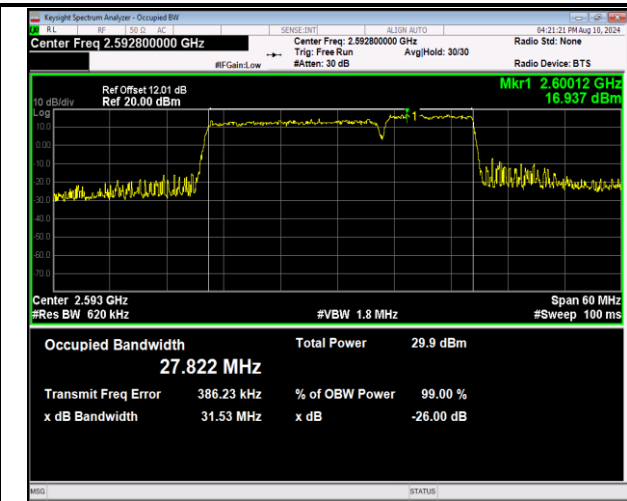
41-41-20MHz-10MHz-16QAM-16QAM-40571-40715-100RB#0-50RB#0-PASS
