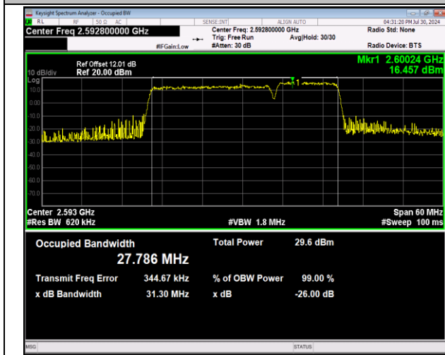
41-41-20MHz-10MHz-64QAM-64QAM-40571-40715-100RB#0-50RB#0-PASS
