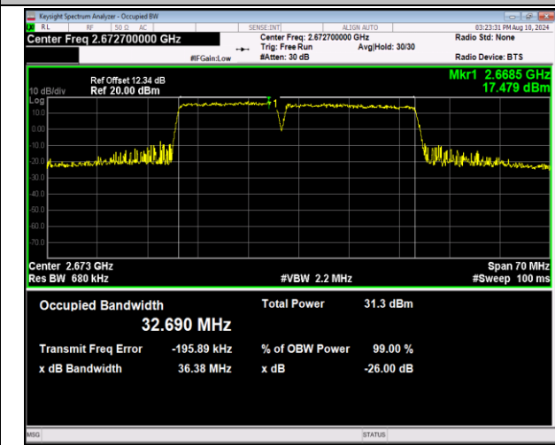
41-41-15MHz-20MHz-QPSK-QPSK-41319-41490-75RB#0 -100RB#0-PASS
