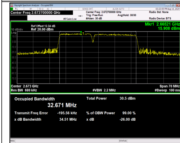
41-41-15MHz-20MHz-16QAM-16QAM-41319-41490-75RB #0-100RB#0-PASS
