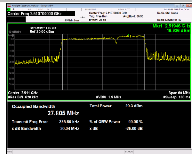
41-41-20MHz-10MHz-64QAM-64QAM-39750-39894-100RB#0-50RB#0-PASS
