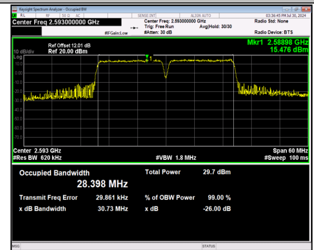
41-41-15MHz-15MHz-64QAM-64QAM-40545-40695-75RB #0-75RB#0-PASS
