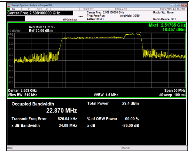
41-41-20MHz-5MHz-16QAM-16QAM-39750-39867-100RB #0-25RB#0-PASS
