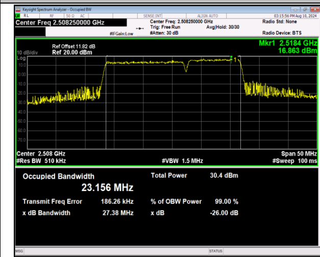
41-41-15MHz-10MHz-QPSK-QPSK-39725-39845-75RB#0 -50RB#0-PASS
