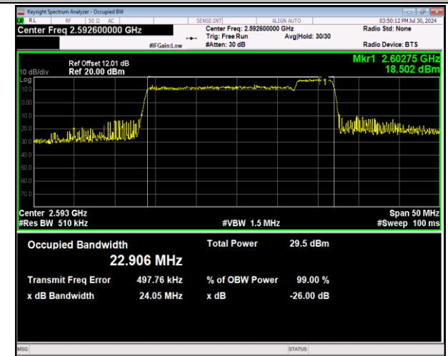
41-41-20MHz-5MHz-64QAM-64QAM-40595-40712-100RB #0-25RB#0-PASS
