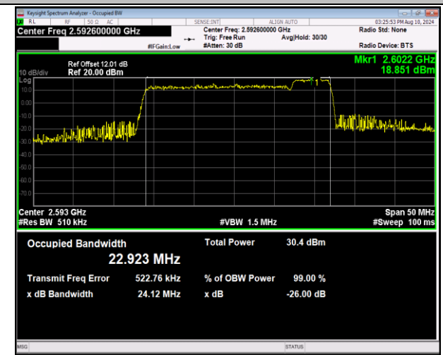
41-41-20MHz-5MHz-QPSK-QPSK-40595-40712-100RB#0 -25RB#0-PASS
