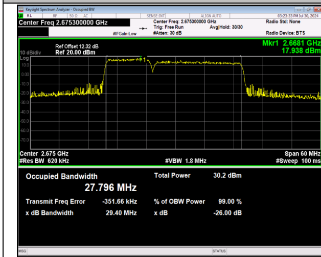
41-41-10MHz-20MHz-64QAM-64QAM-41346-41490-50RB#0 -100RB#0-PASS
