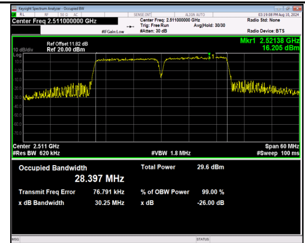
41-41-15MHz-15MHz-16QAM-16QAM-39725-39875-75RB #0-75RB#0-PASS
