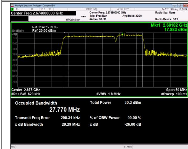
41-41-20MHz-10MHz-16QAM-16QAM-41391-41535-100RB#0-50RB#0-PASS
