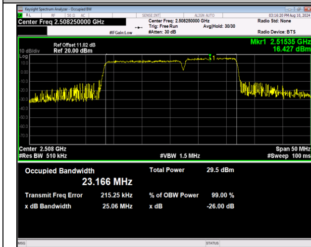
41-41-15MHz-10MHz-16QAM-16QAM-39725-39845-75RB#0 -50RB#0-PASS
