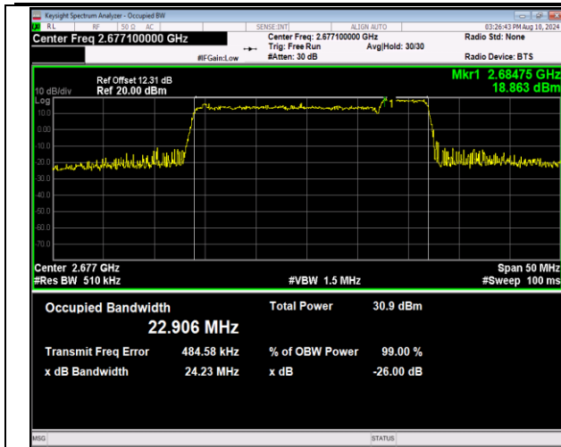
41-41-20MHz-5MHz-QPSK-QPSK-41440-41557-100RB#0-25RB#0-PASS
