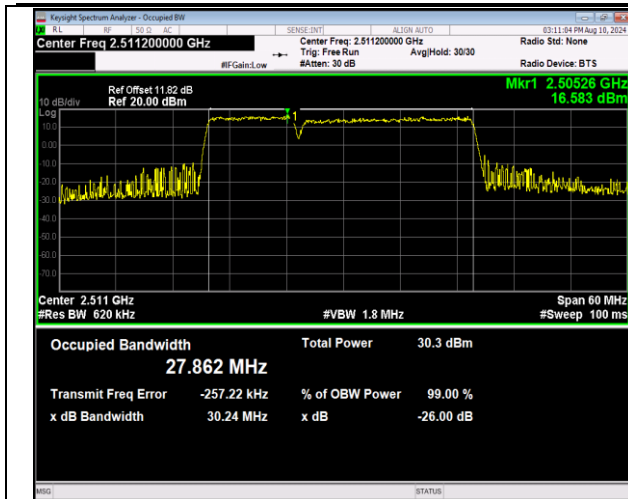
41-41-10MHz-20MHz-QPSK-QPSK-39705-39849-50RB#0 -100RB#0-PASS
