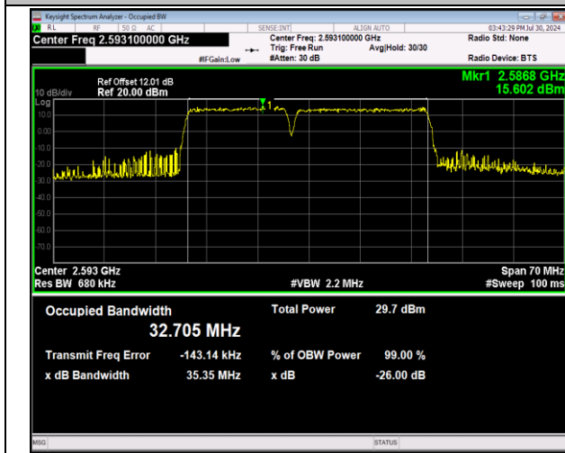
41-41-15MHz-20MHz-64QAM-64QAM-40523-40694-75RB #0-100RB#0-PASS
