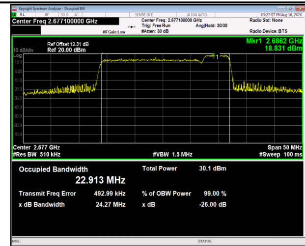
41-41-20MHz-5MHz-16QAM-16QAM-41440-41557-100RB#0-25RB#0-PASS
