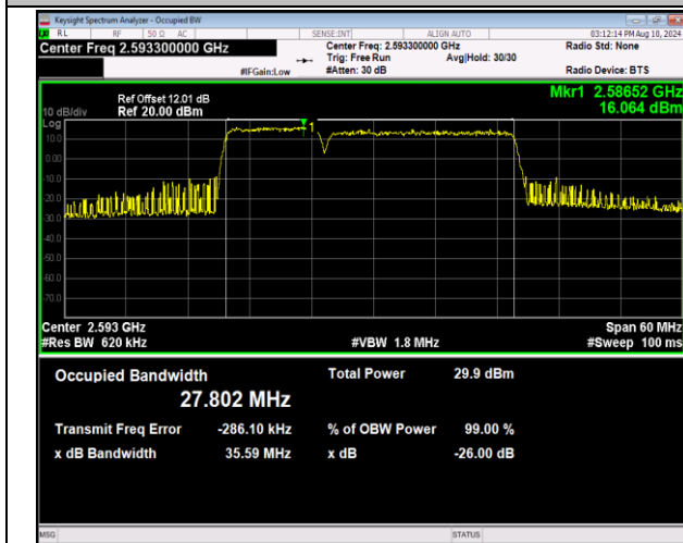
41-41-10MHz-20MHz-16QAM-16QAM-40526-40670-50RB #0-100RB#0-PASS
