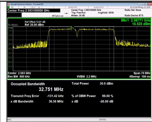
41-41-15MHz-20MHz-16QAM-16QAM-40523-40694-75RB #0-100RB#0-PASS
