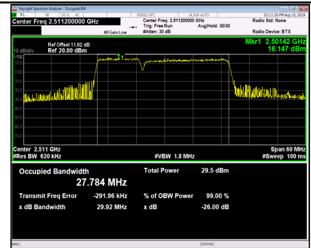
41-41-10MHz-20MHz-16QAM-16QAM-39705-39849-50RB #0-100RB#0-PASS
