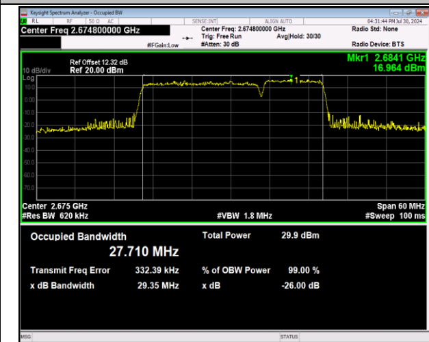
41-41-20MHz-10MHz-64QAM-64QAM-41391-41535-100RB#0-50RB#0-PASS
