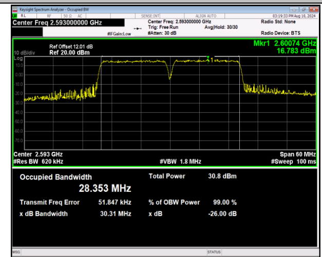
41-41-15MHz-15MHz-QPSK-QPSK-40545-40695-75RB#0 -75RB#0-PASS
