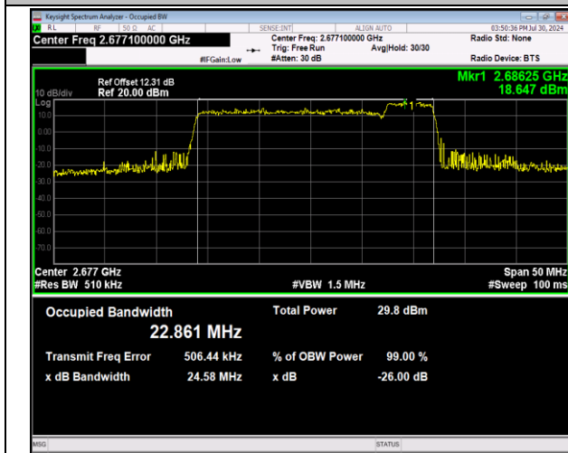
41-41-20MHz-5MHz-64QAM-64QAM-41440-41557-100RB#0-25RB#0-PASS
