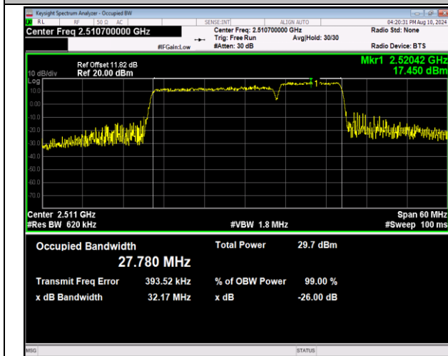
41-41-20MHz-10MHz-16QAM-16QAM-39750-39894-100RB#0-50RB#0-PASS
