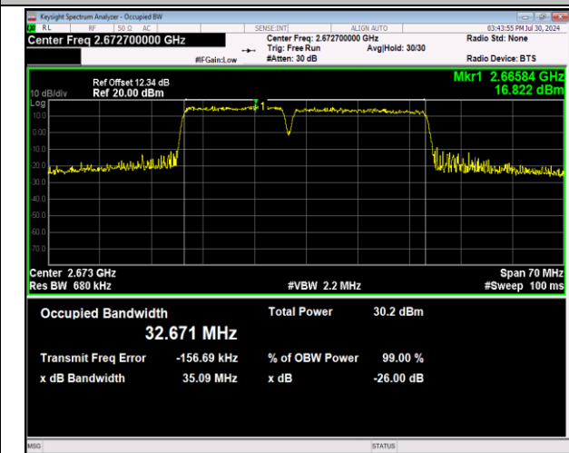
41-41-15MHz-20MHz-64QAM-64QAM-41319-41490-75RB #0-100RB#0-PASS
