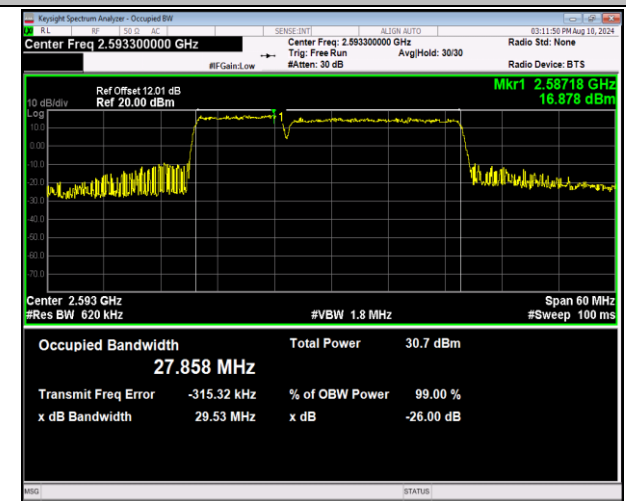
41-41-10MHz-20MHz-QPSK-QPSK-40526-40670-50RB#0 -100RB#0-PASS
