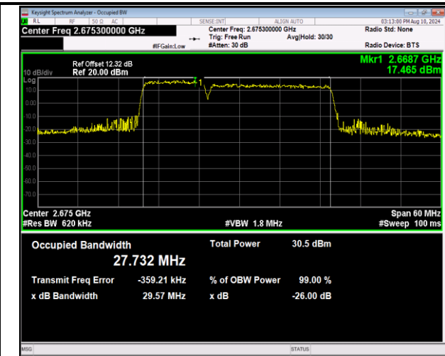
41-41-10MHz-20MHz-16QAM-16QAM-41346-41490-50RB#0 -100RB#0-PASS
