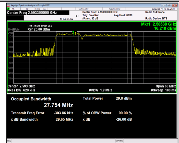
41-41-10MHz-20MHz-64QAM-64QAM-40526-40670-50RB #0-100RB#0-PASS
