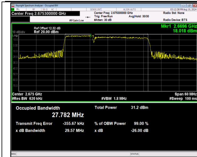
41-41-10MHz-20MHz-QPSK-QPSK-41346-41490-50RB#0 -100RB#0-PASS
