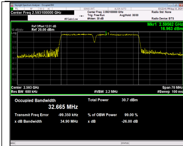
41-41-15MHz-20MHz-QPSK-QPSK-40523-40694-75RB#0 -100RB#0-PASS
