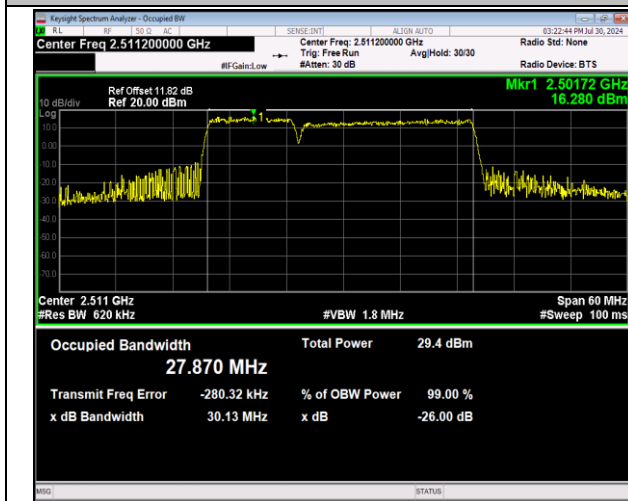
41-41-10MHz-20MHz-64QAM-64QAM-39705-39849-50RB #0-100RB#0-PASS
