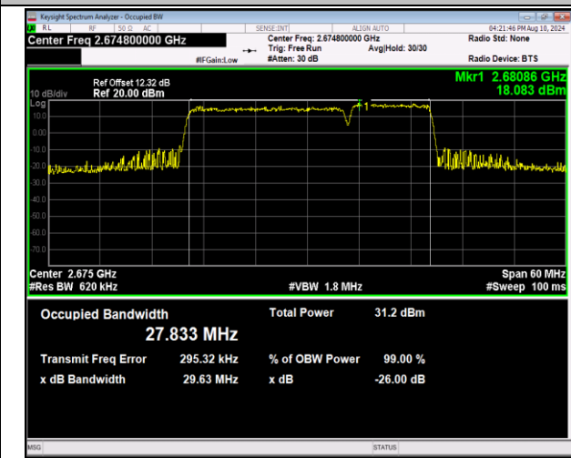
41-41-20MHz-10MHz-QPSK-QPSK-41391-41535-100RB#0-50RB#0-PASS
